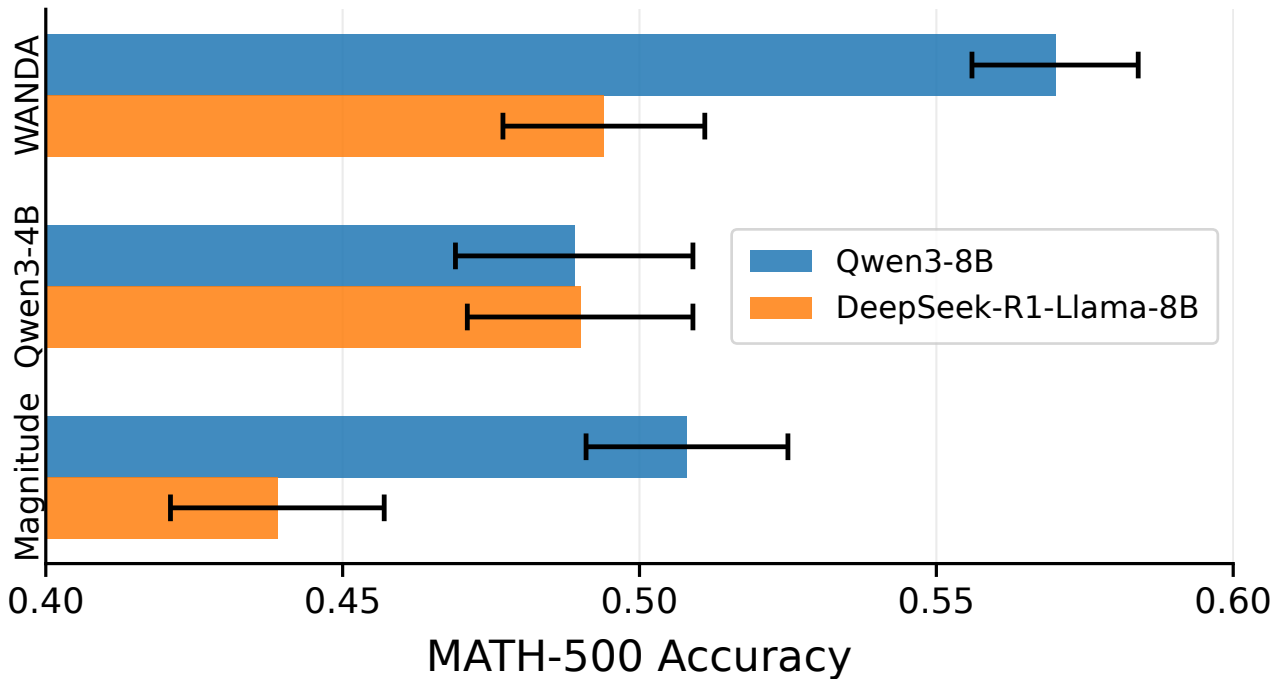
MATH-500 Accuracy by Teacher and Method
