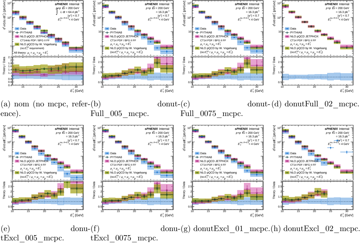
Figure 13: Per-variant final cross section with MC-purity correction enabled (mc_purity_correction=1). Nominal (no mcpc) panel included as reference. The donutExcl_005_mcpc panel no longer shows the negative-yield pathology at high p_T .
