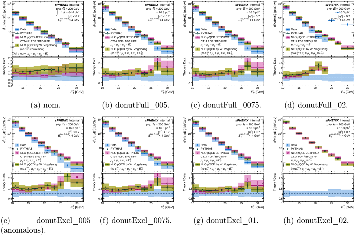
Figure 8: Per-variant final isolated-photon cross section d^2\sigma/d\eta dp_T vs. p_T^\gamma , produced by plot_final_selection.C. Nominal topo04 iso (first panel) for reference. The donutExcl_005 panel shows the high- p_T anomaly noted above.
