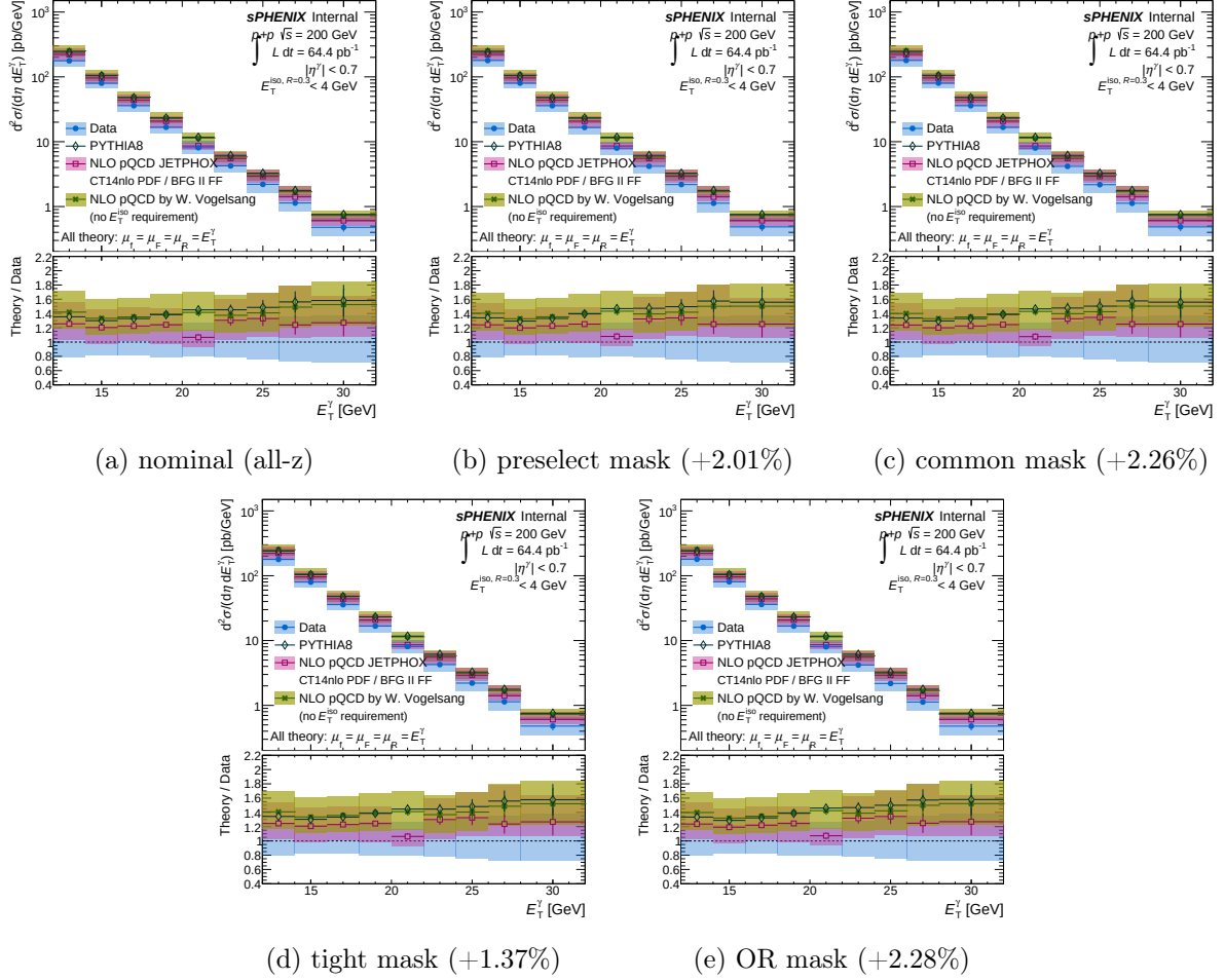
Figure 6: Official PPG12 cross-section plots (upper: Data vs NLO theory; lower: Theory/Data) for the nominal and four phi-symm variants. All four variants produce nearly-identical spectra — the mask does not distort the E_T^\gamma shape.
