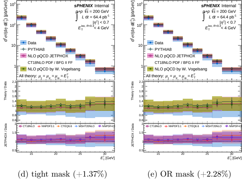
Figure 6: Official PPG12 cross-section plots (upper: Data vs NLO theory; lower: Theory/Data) for the nominal and four phi-symm variants. All four variants produce nearly-identical spectra — the mask does not distort the E_T^\gamma shape.
