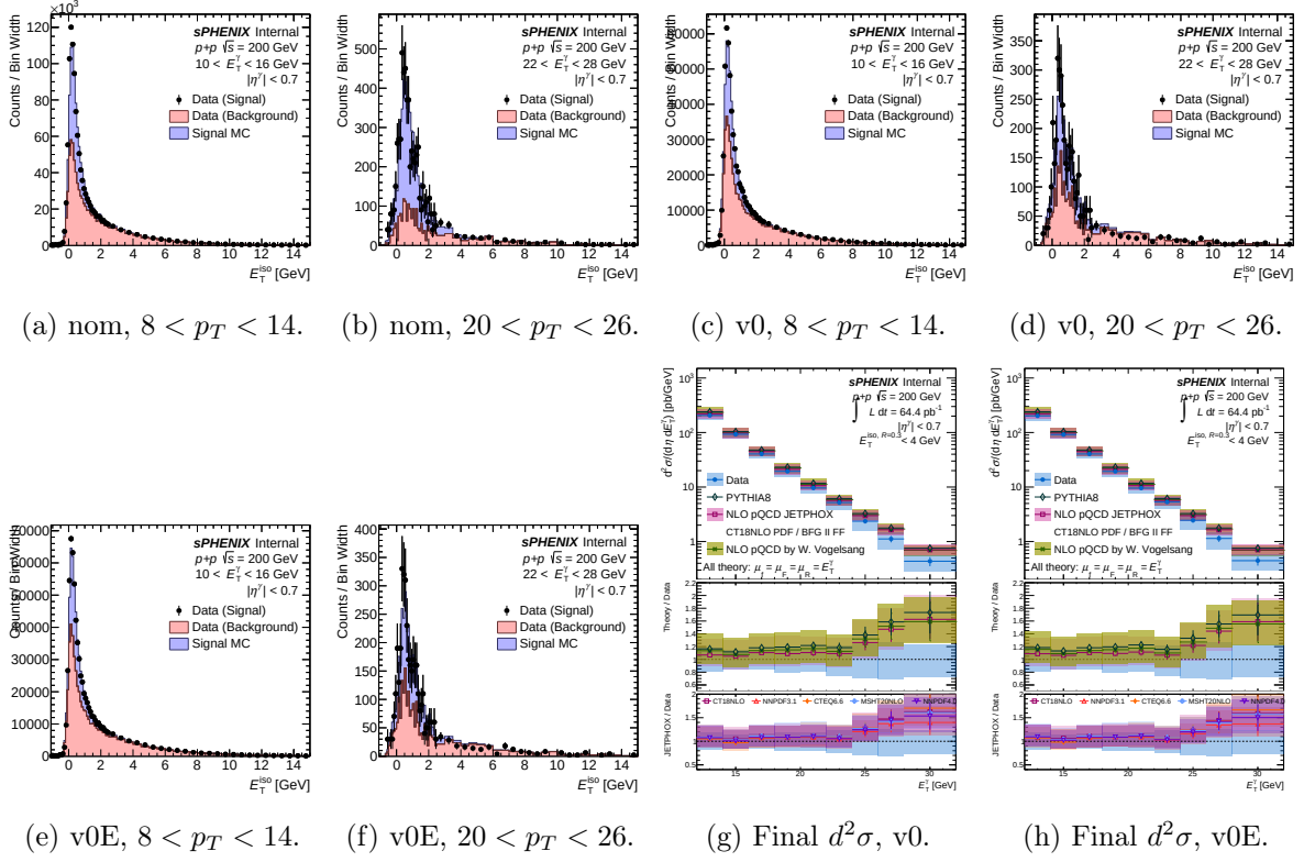
Figure 12: CONF template overlays (h1D_iso_*: tight data points, MC signal template in blue fill, non-tight background template in red fill) for nominal and the two alternative BDT models at two p_T ranges, followed by the unfolded final cross section per alternative model. Poorer template agreement for v0/v0E at high p_T is consistent with the weaker closure reported above.
