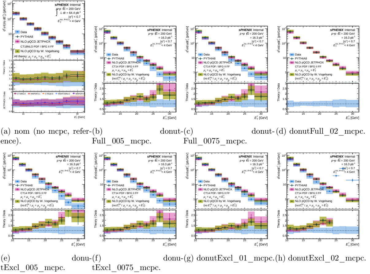
Figure 13: Per-variant final cross section with MC-purity correction enabled ( mc_purity_correction=1 ). Nominal (no mcpc) panel included as reference. The donutExcl_005_mcpc panel no longer shows the negative-yield pathology at high p_T .
