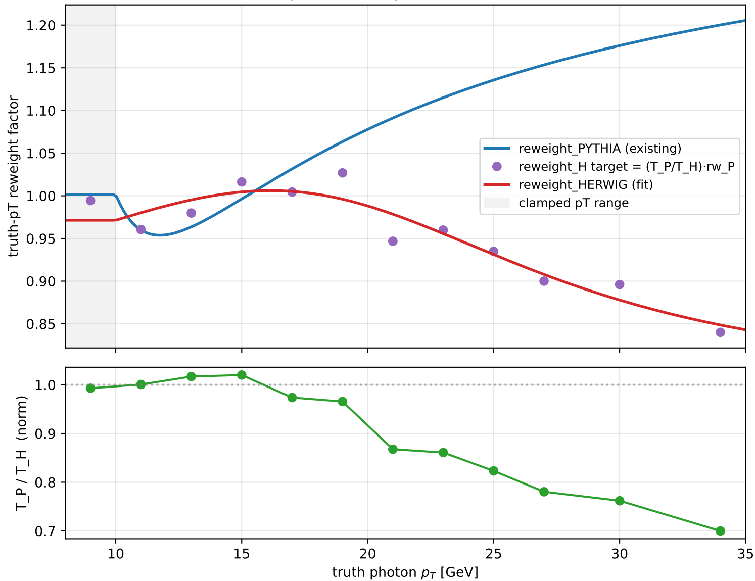
HERWIG-specific reweight derivation (1.5 mrad)
