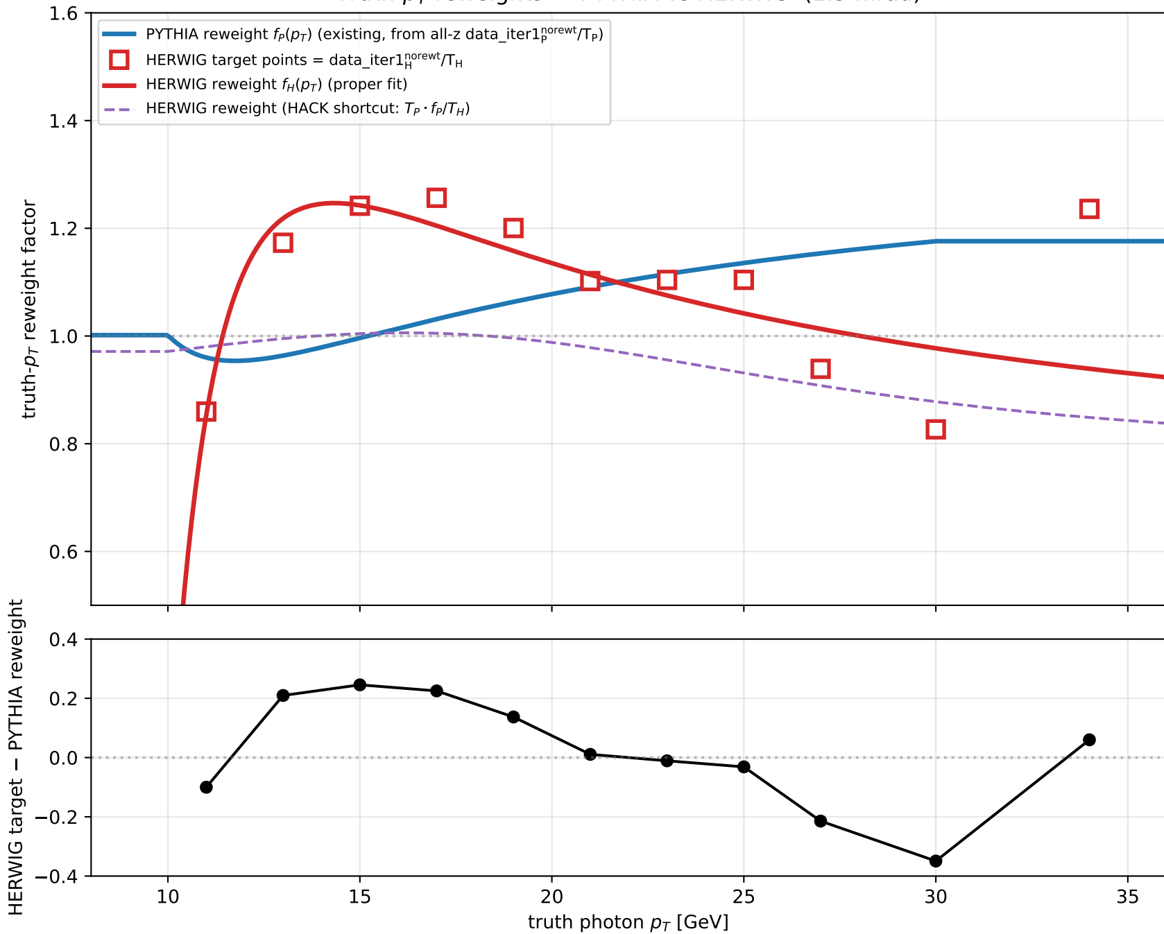
Truth- p_T reweights — PYTHIA vs HERWIG (1.5 mrad)
