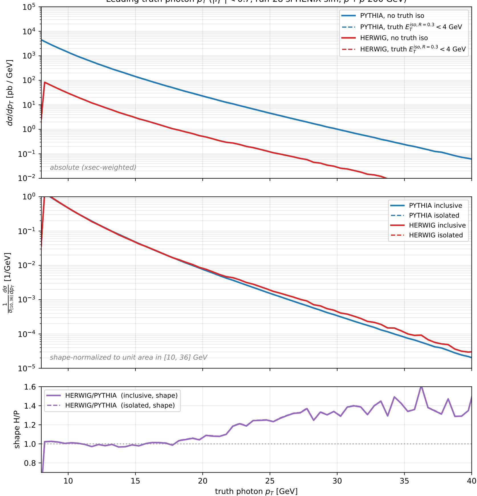
Leading truth photon p_T ( |\eta^\gamma| < 0.7 , run-28 sPHENIX sim, p + p 200 GeV)
