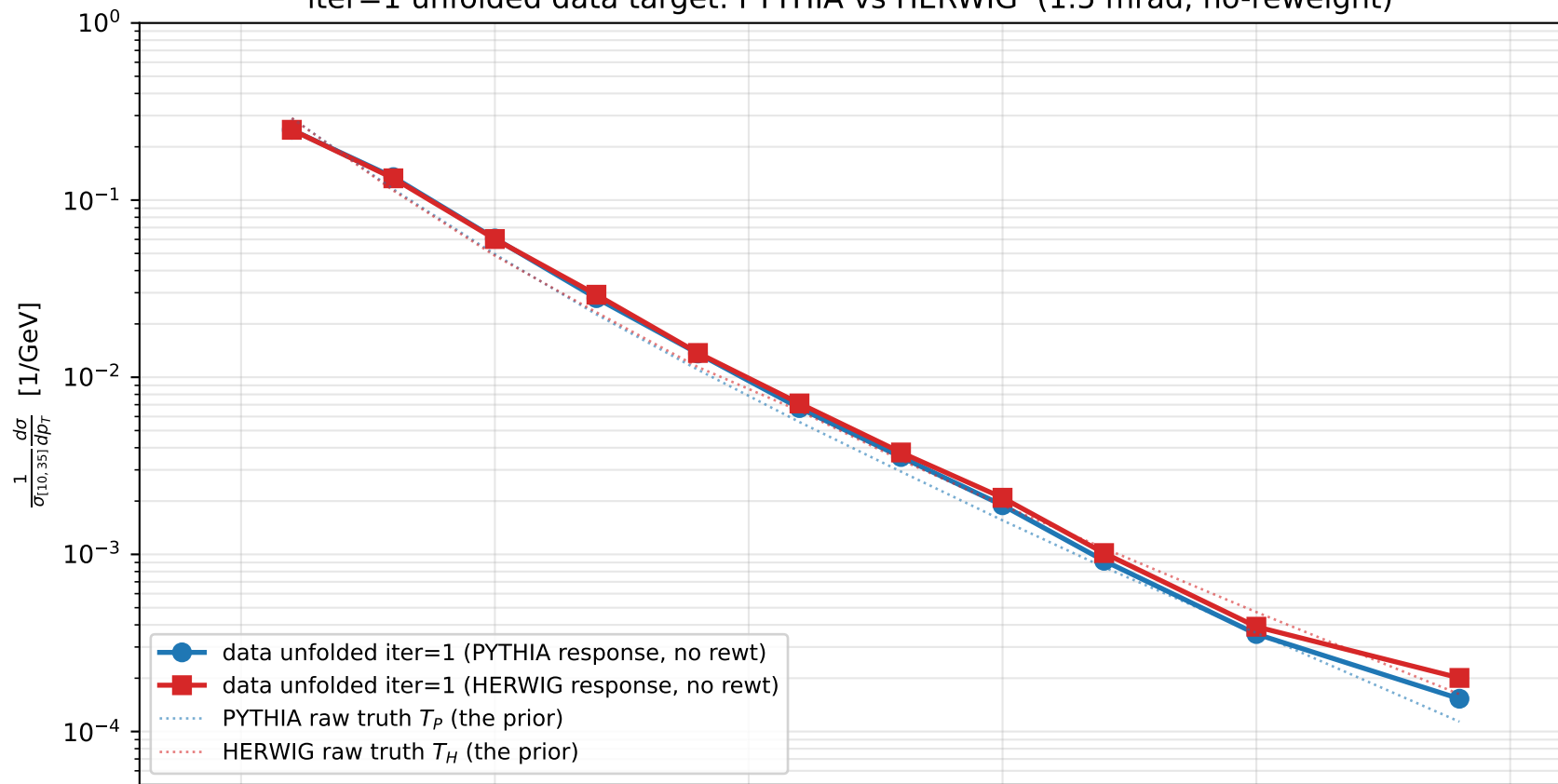
iter=1 unfolded data target: PYTHIA vs HERWIG (1.5 mrad, no-reweight)
