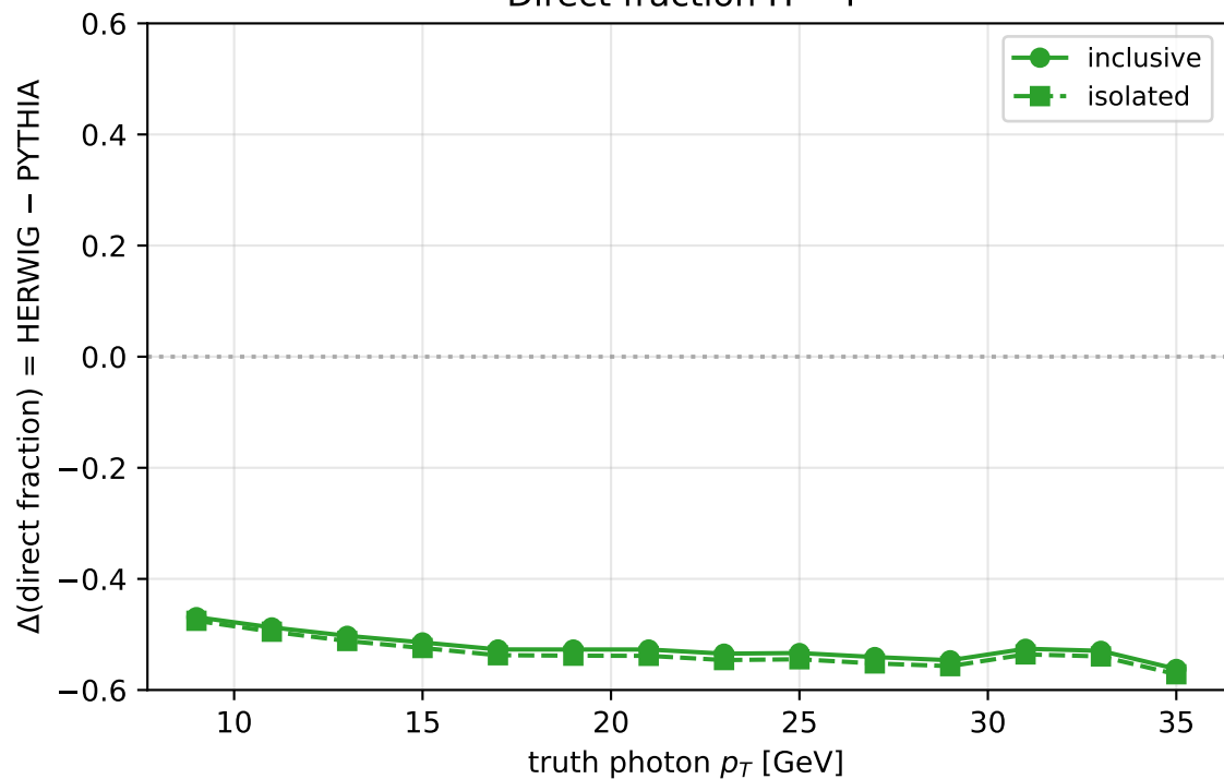
Direct fraction H – P
