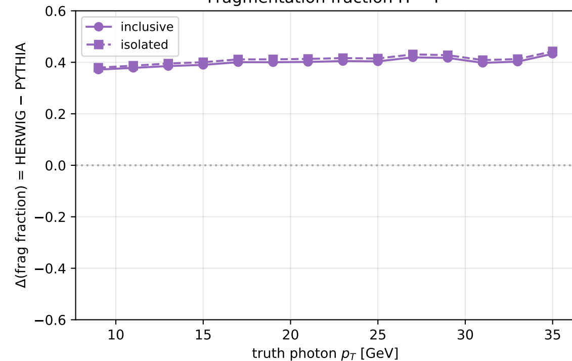
Fragmentation fraction H – P
