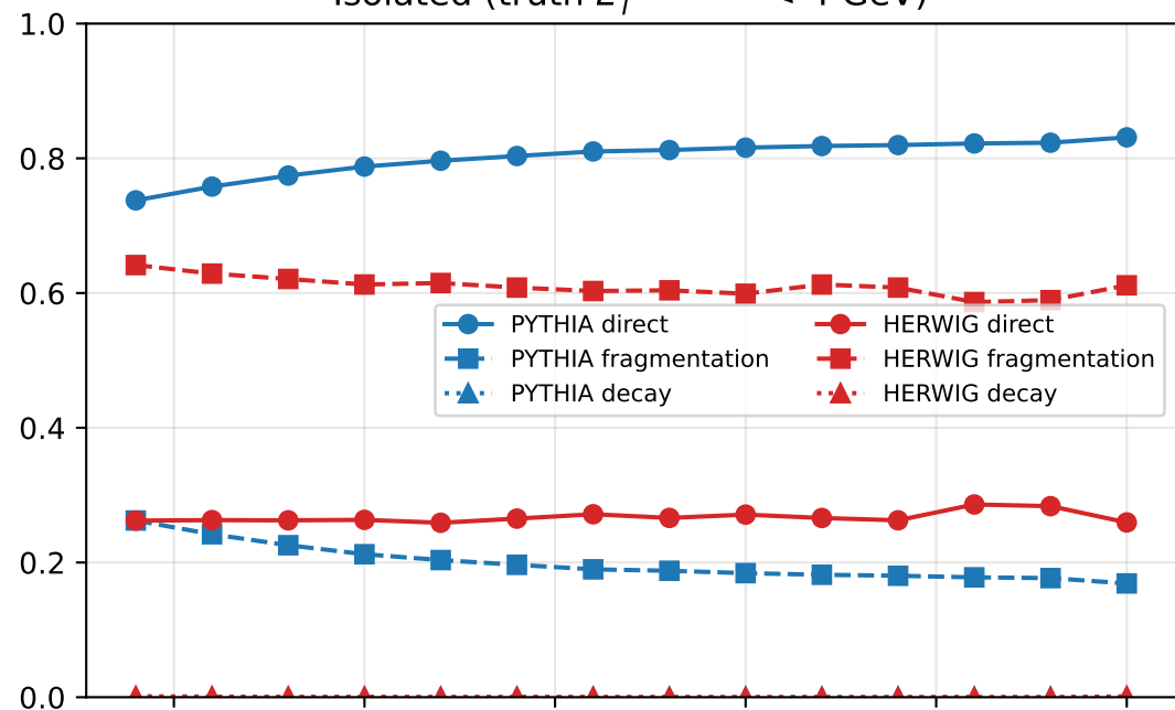
Direct fraction H – P
