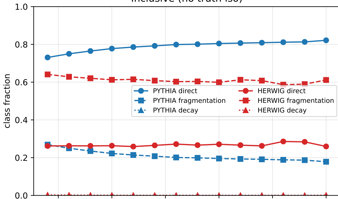
Fragmentation fraction H – P
