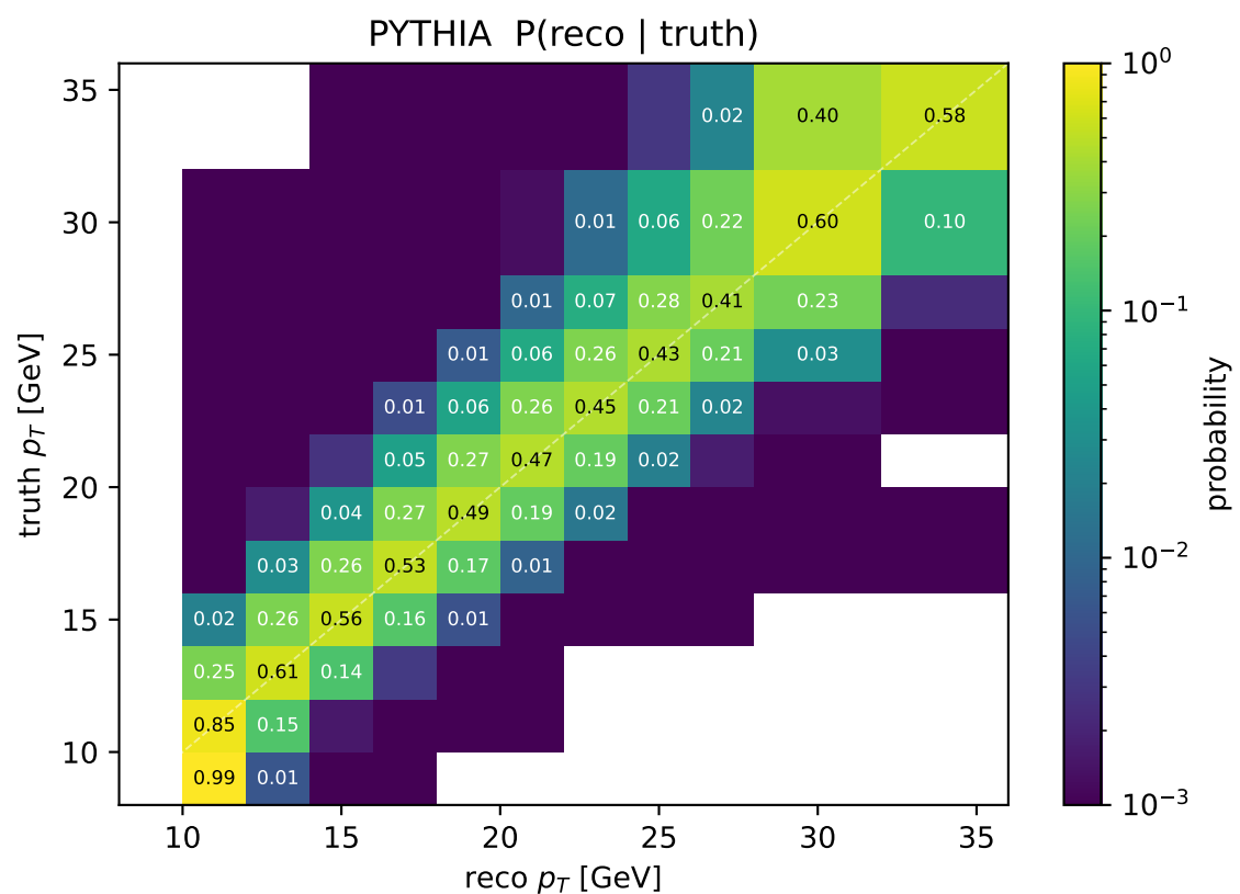
Row-normalized response matrix P(\text{reco} \mid \text{truth}) — PYTHIA vs HERWIG (1.5 mrad)
