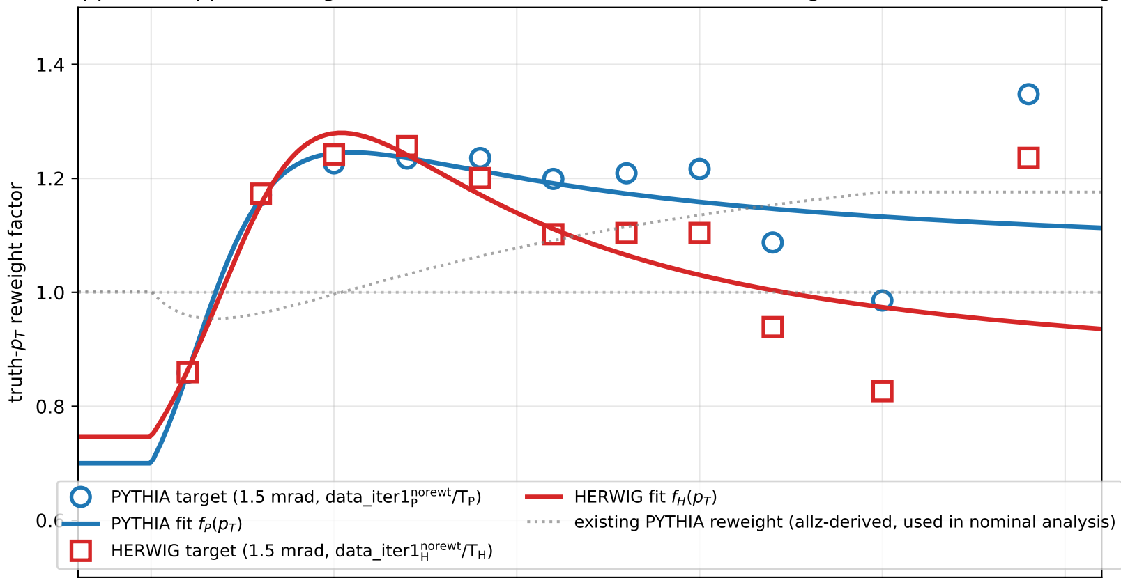
Apples-to-apples reweight derivation: PYTHIA & HERWIG, no-reweight iter=1, 1.5 mrad config
