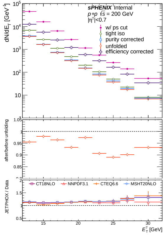
(a) All correction steps — \text{bdt\_nom}
