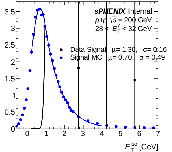
(b) IsoET fit template (pT bins 9–9) — bdt_none
