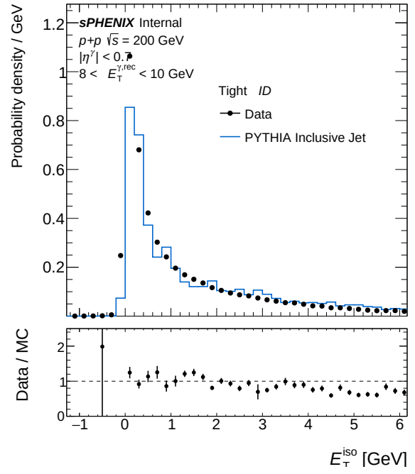
(b) IsoET Tight, pT bin 0 — bdt_nosplit
