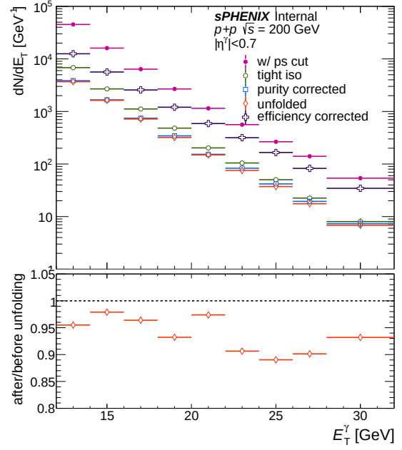
(b) All correction steps — \text{bdt\_vtxreweight0}
