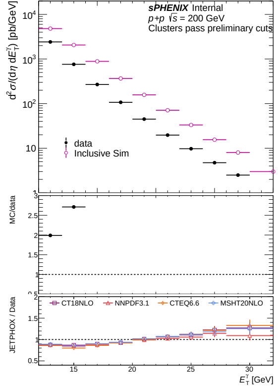
(b) Common cluster yield (data vs MC) — bdt_none
