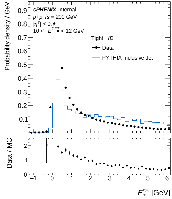
(b) IsoET Tight, pT bin 0 — bdt_none
