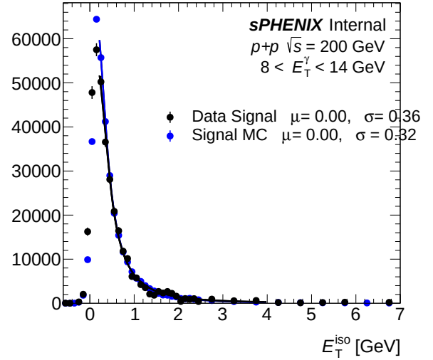
(b) IsoET fit template (pT bins 0-2) — bdt_nosplit
