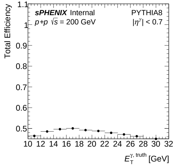
(b) Total efficiency — bdt_none
