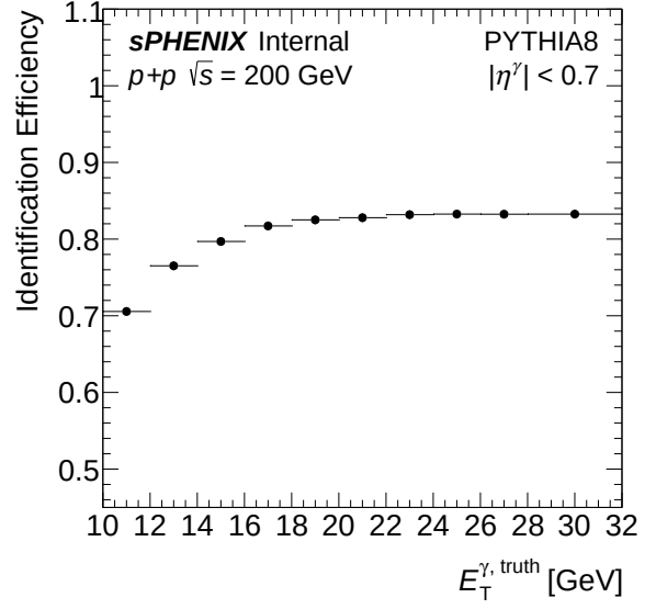
(b) Identification efficiency — bdt_none
