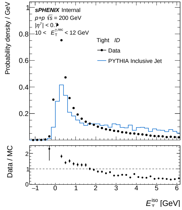
(b) IsoET Tight, pT bin 0 — bdt_npb03
