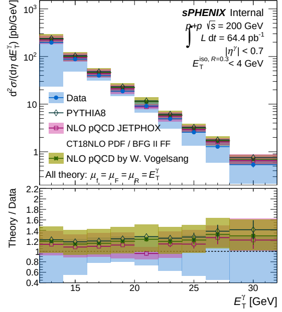
(b) Final cross section result — bd_t_npb03
