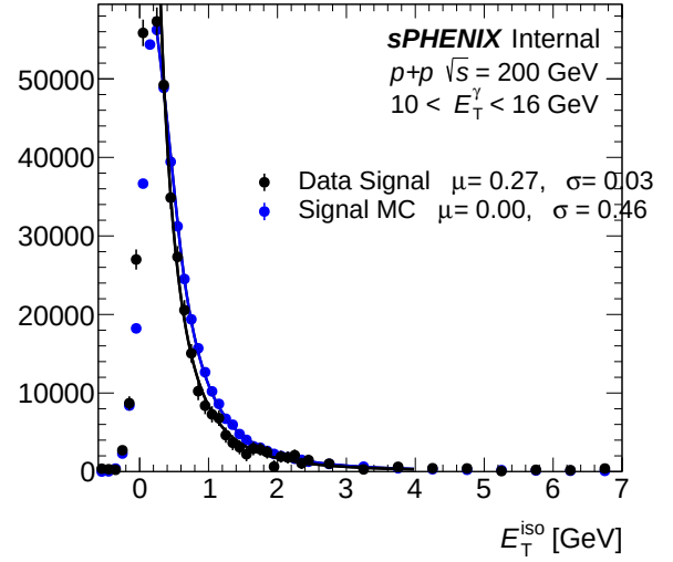
(b) IsoET fit template (pT bins 0-2) — bdt_npb03
