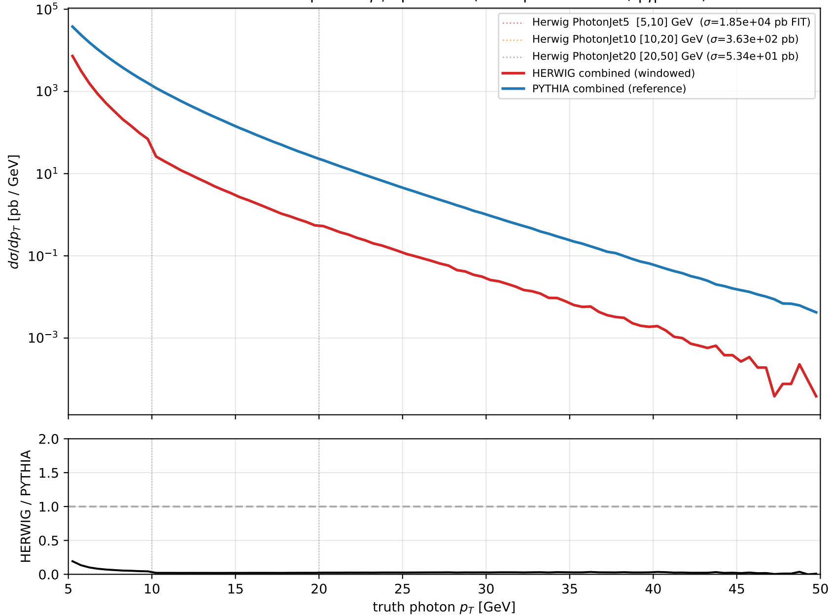
Combined truth photon p_T spectrum (truth- p_T windowed; |\eta| < 0.7 )
