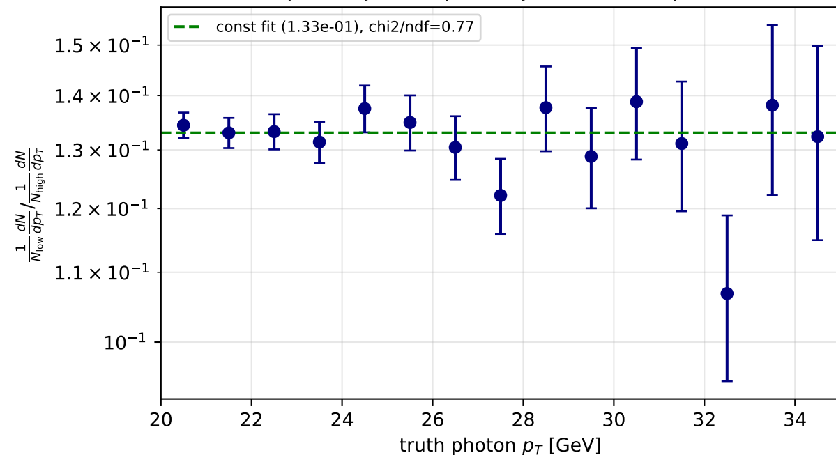
HERWIG photonjet10 / photonjet20 (overlap 20-35 GeV)
