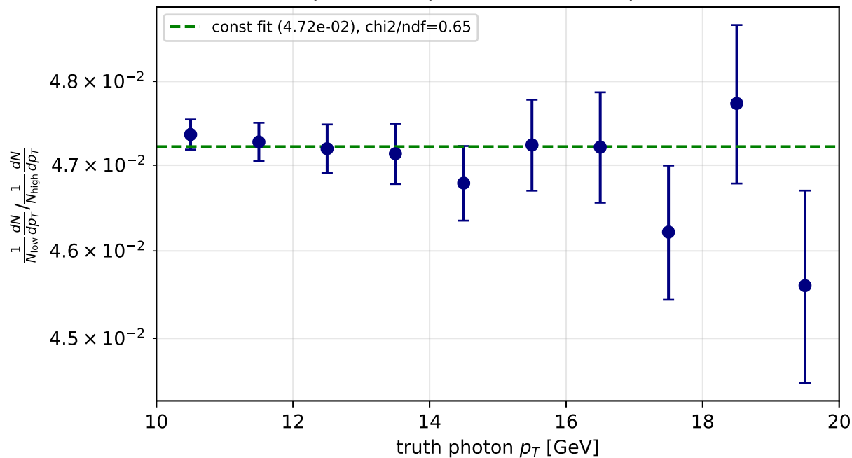
PYTHIA photon5 / photon10 (overlap 10-20 GeV)
