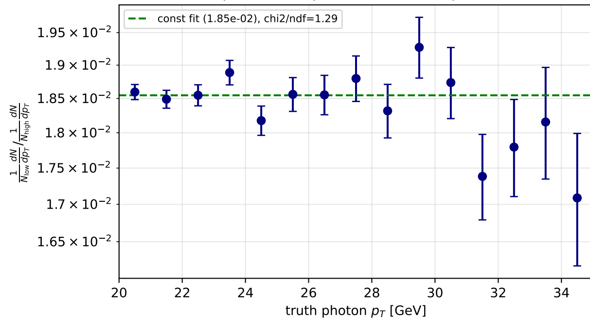
PYTHIA photon10 / photon20 (overlap 20-35 GeV)
