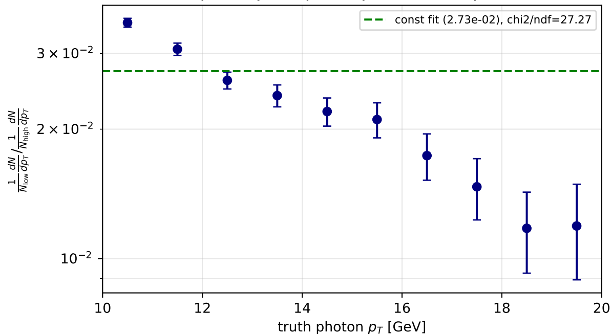
HERWIG photonjet5 / photonjet10 (overlap 10-20 GeV)
