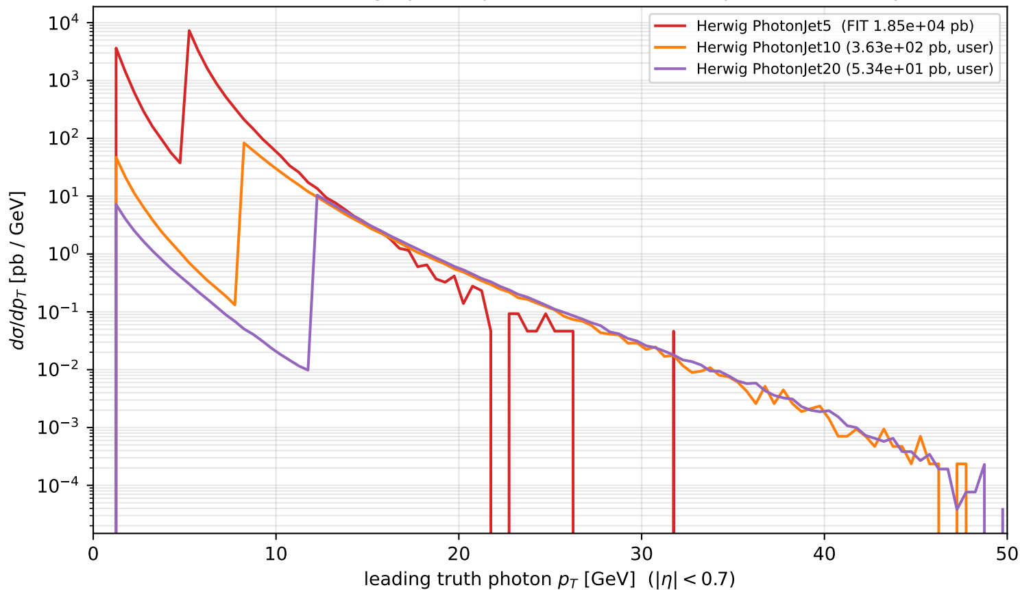
HERWIG stitching - photonjet5 fitted ( 1.85\text{e}+04 pb) from overlap
