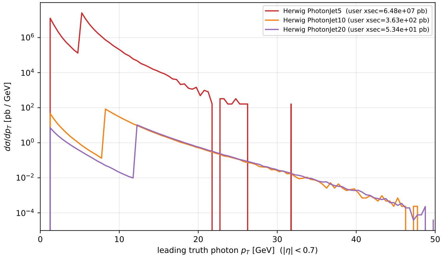
HERWIG photonjet stitching — user xsec (literal pb)
