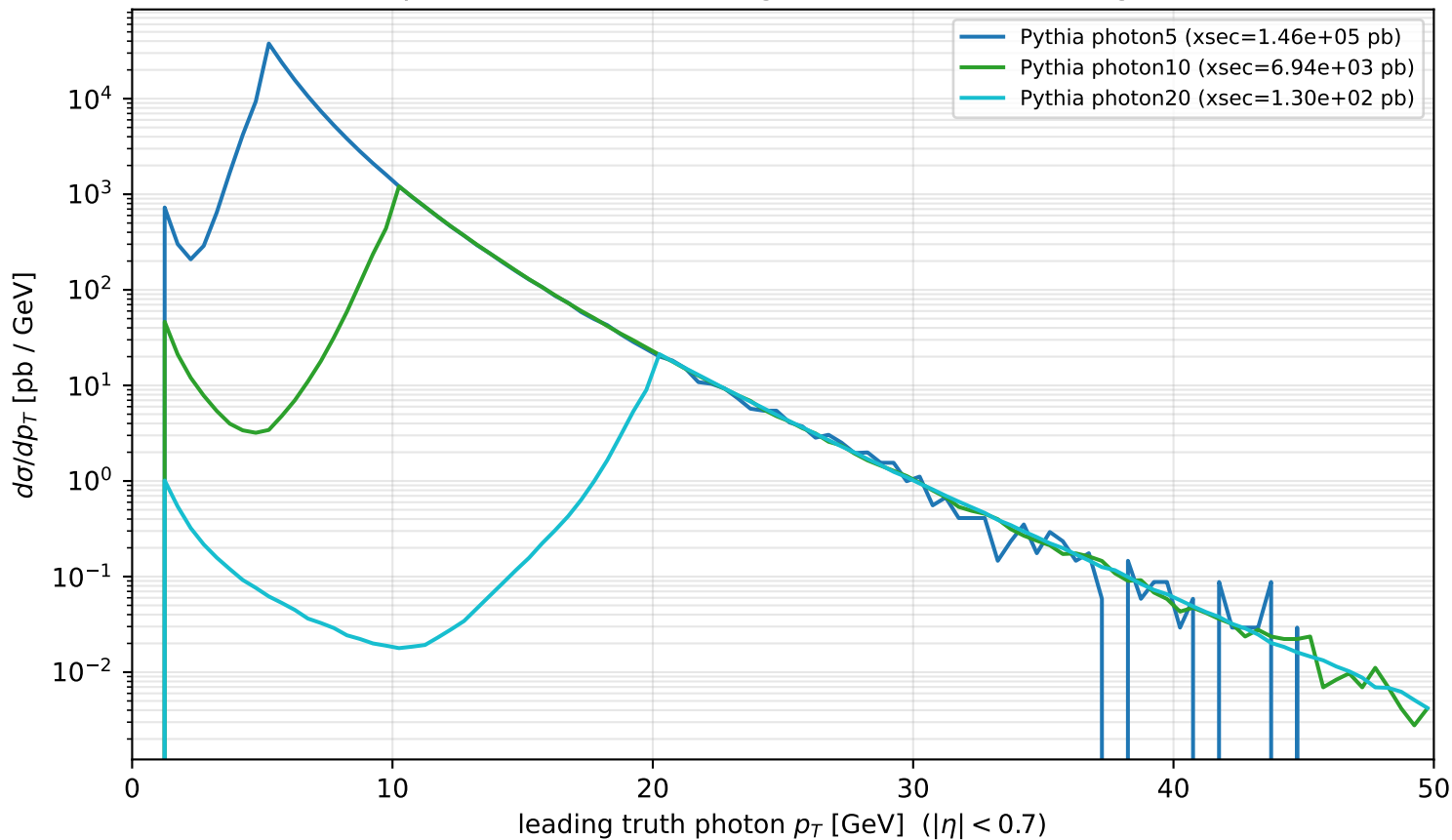
PYTHIA photon5/10/20 stitching — reference (known-good xsec)
