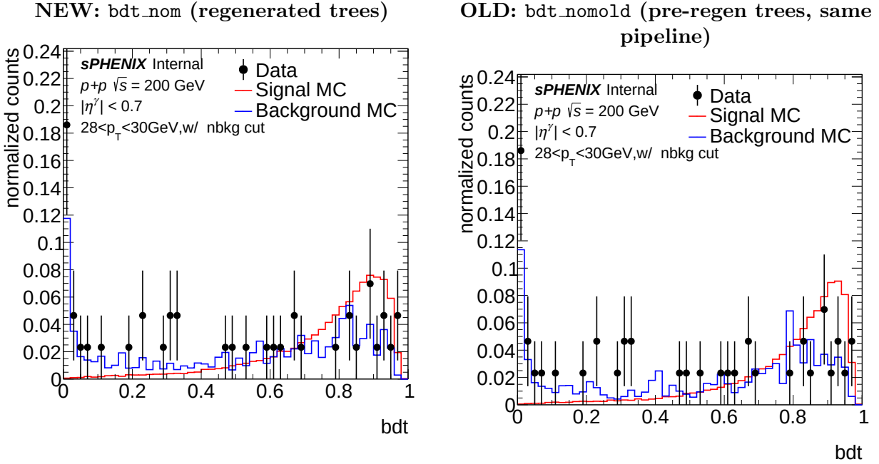
Figure 5: [Item 4 — shower-shape BDT score, THE DRIVER .] Signal-MC BDT photon-ID score (1.5 mrad, 28–30 GeV) from plot_showershapes.C . The NEW signal BDT shifts to lower values (mean 0.762 vs 0.785; fraction with \text{BDT} > 0.5 : 0.904 vs 0.920) — the direct cause of the ID-efficiency drop.
