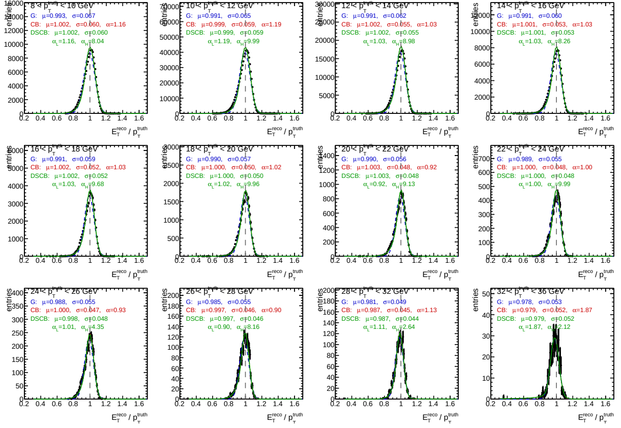
Figure 18: DSCB fit QC grid for single-interaction MC at tight-iso level. Gauss (blue dashed), one-sided CB (red dotted), and DSCB (green solid) fits overlaid. DSCB absorbs both the low-side and the high-side tails; the stated \mu, \sigma, \alpha_L, \alpha_H are from the DSCB fit.
