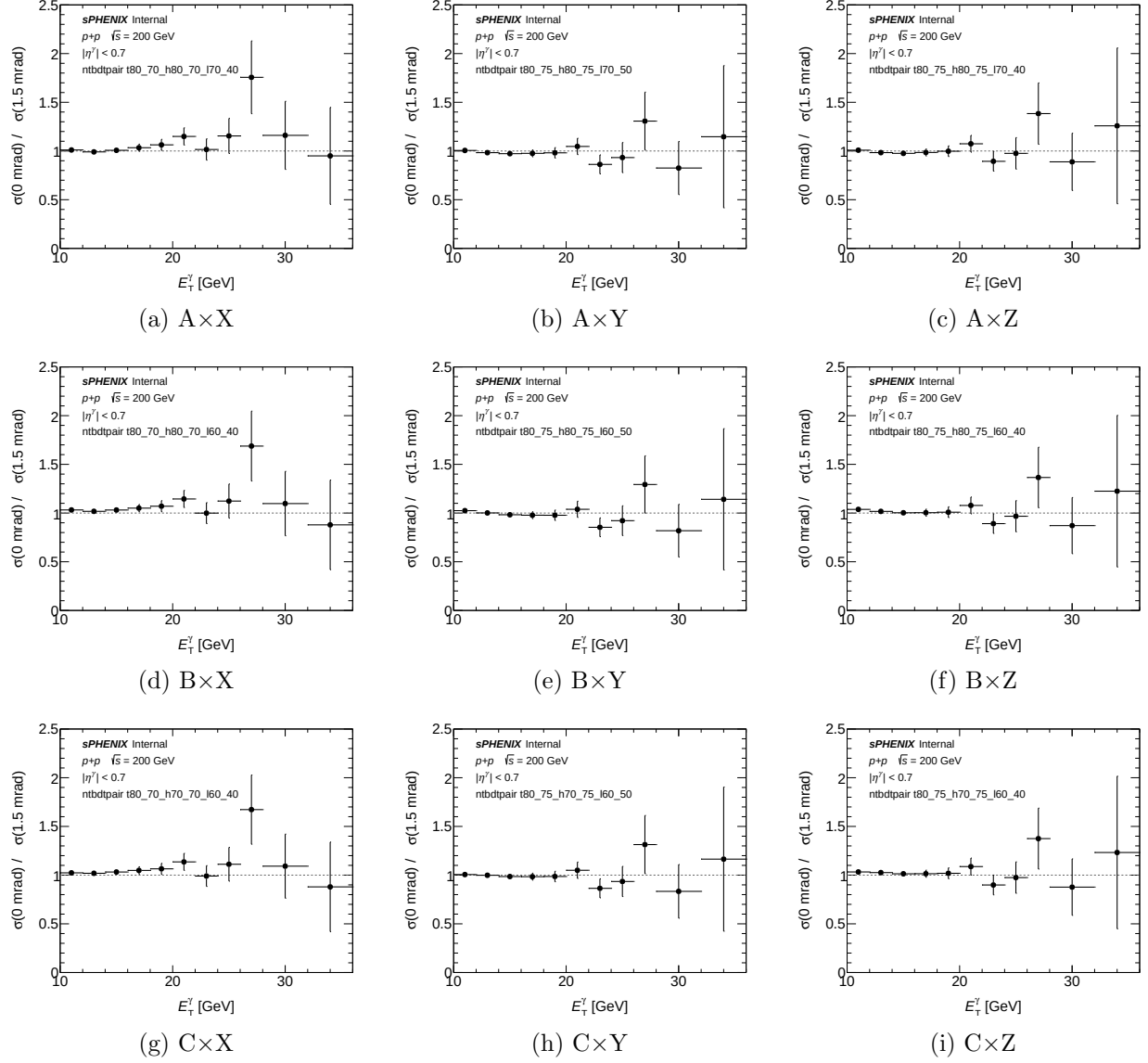
Figure 13: Per-variant unfolded cross-section ratio \sigma_{\text{var}}^{0\text{mrad}}/\sigma_{\text{var}}^{1.5\text{mrad}} vs E_T^\gamma . Generated by plotting/plot_ntbdtpair_period_ratio.C (new macro, h_unfold_sub_result divided bin-by-bin between the two period outputs). Agreement with unity (dashed gray) would indicate that the BDT cut is cross-check-stable across crossing angles; any systematic offset flags a period-dependent ABCD response.
