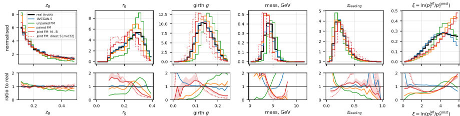
Fig. 6: substructure, R = 0.4 , 20 < p_T^{real} < 30 GeV, PYTHIA+HIJING (val) (ratio band: seed range)
