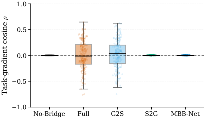
(a) ShapeNet-55: Gradient Alignment
