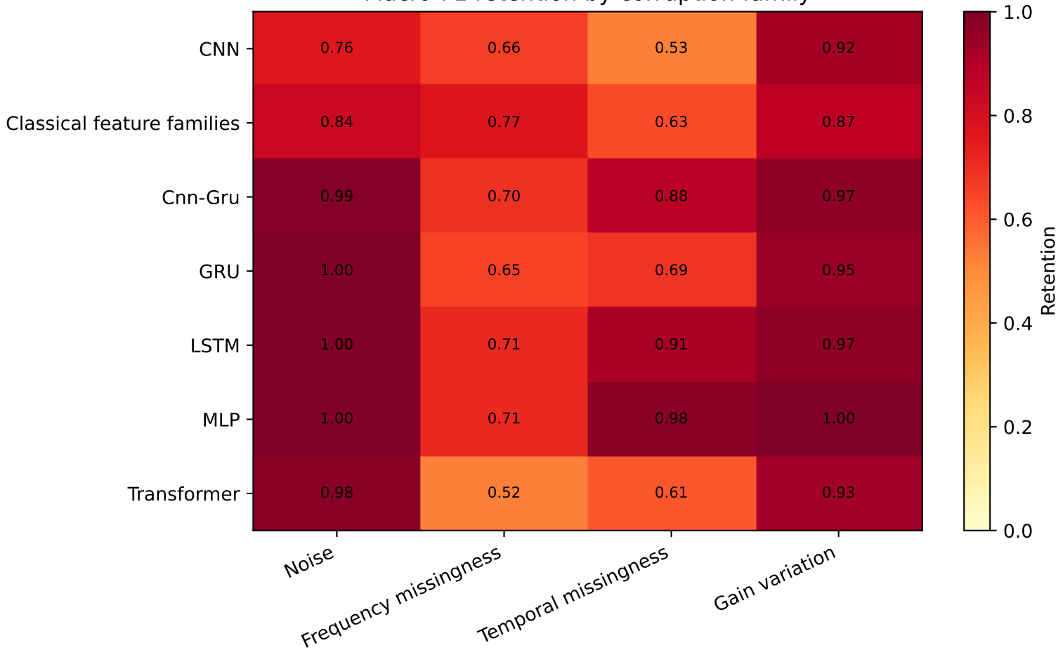
Macro-F1 retention by corruption family
