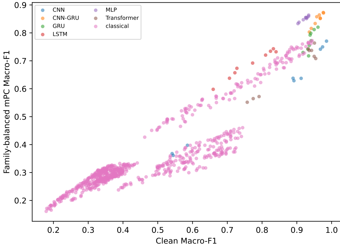
Final model bank: clean vs corrupted
