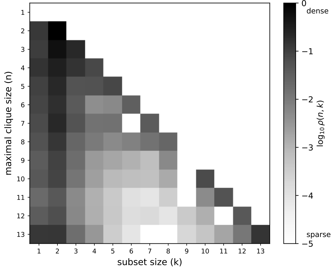
\rho(n, k) on query ( \mathcal{H}_1, \mathcal{G}_1 )
