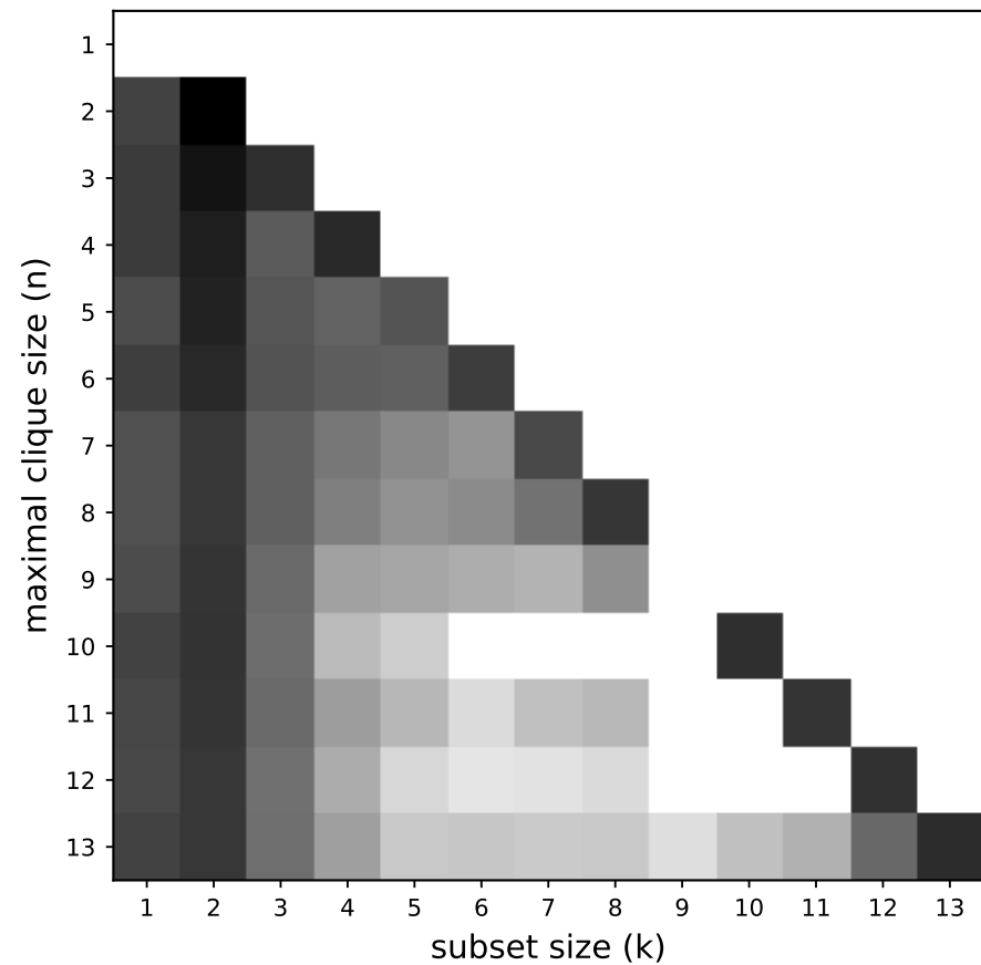
\rho(n, k) on training ( \mathcal{H}_0, \mathcal{G}_0 )
