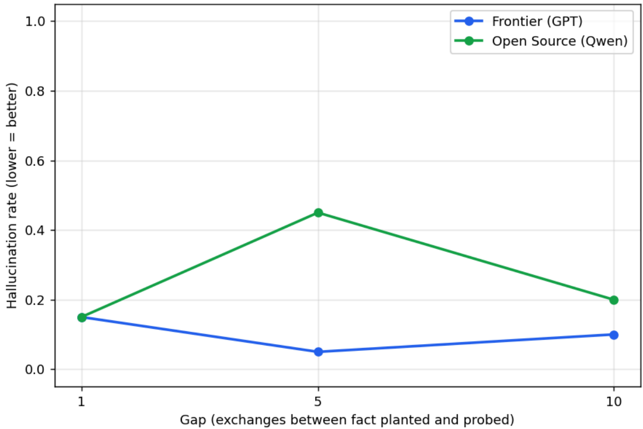
Hallucination vs turn-distance
