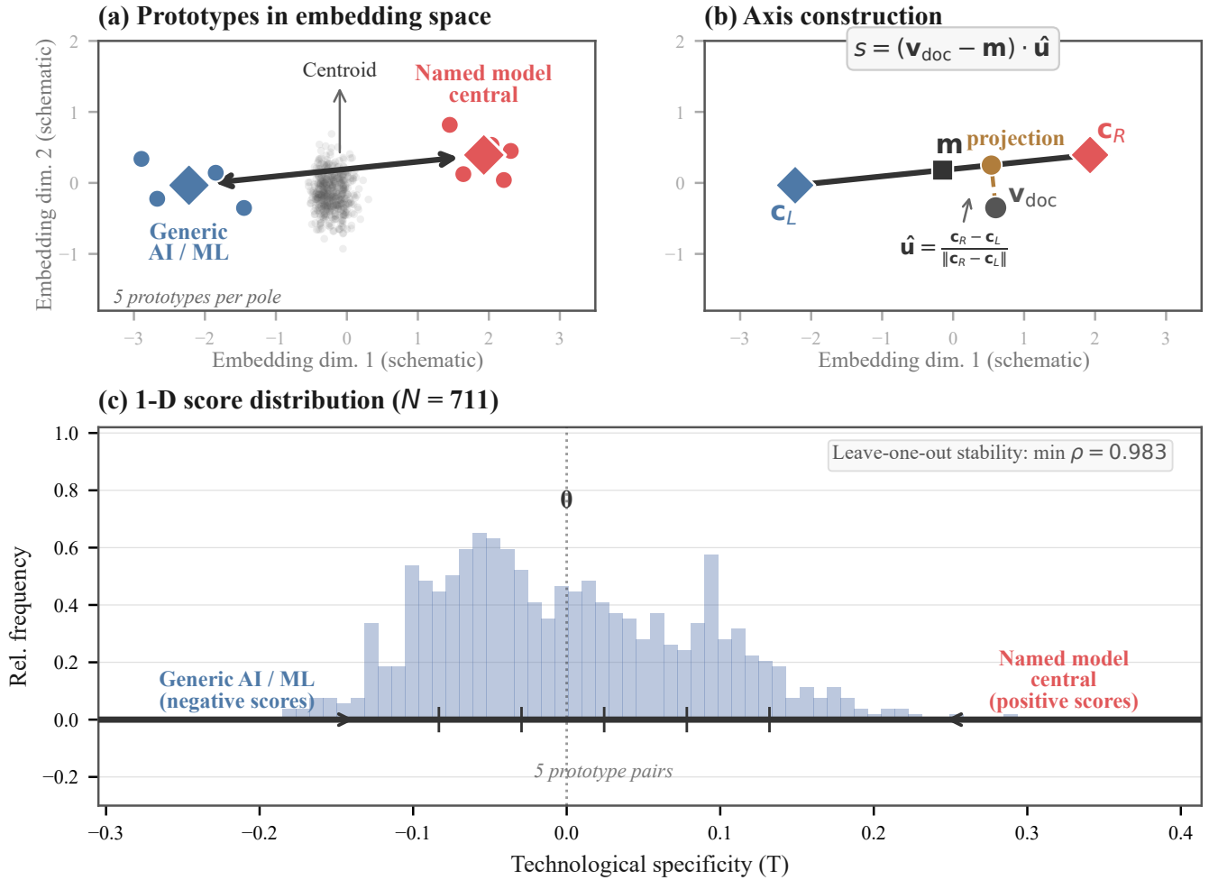
Fig. 1. Construction and interpretation of a prototype-based semantic axis, illustrated with the technological-specificity ( T ) dimension. (a) Five prototype abstracts are written at each pole and embedded with BGE-M3; their centroids define the axis direction. (b) A document's score is its centred projection onto the unit vector between centroids: s = (\mathbf{v}_{\text{doc}} - \mathbf{m}) \cdot \hat{\mathbf{u}} . (c) The resulting 1-D score distribution for the 711-record corpus, with leave-one-out prototype stability (minimum \rho = 0.983 ) confirming that the axis is not determined by any single prototype.
