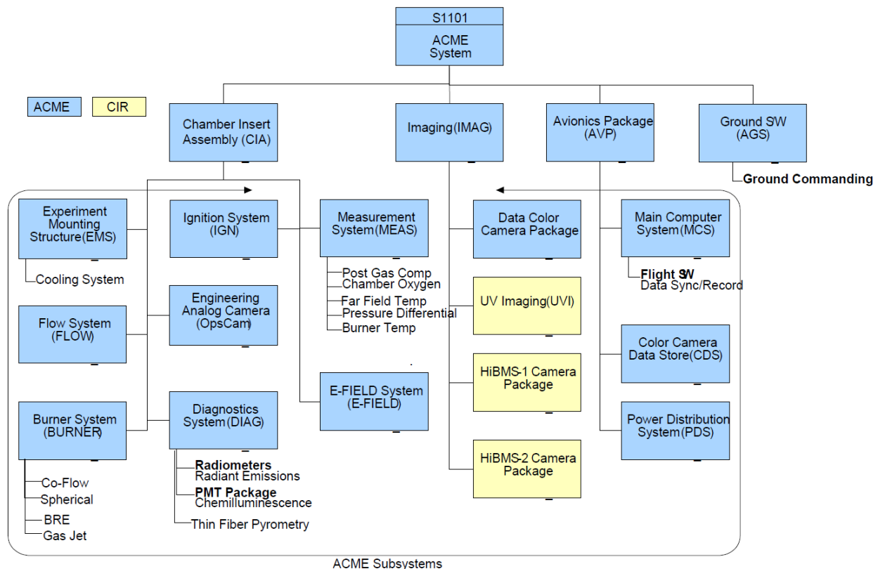
Figure 9. ACME subsystems as identified in ACME's Critical Design Review (CDR) held in Nov. 2013.
