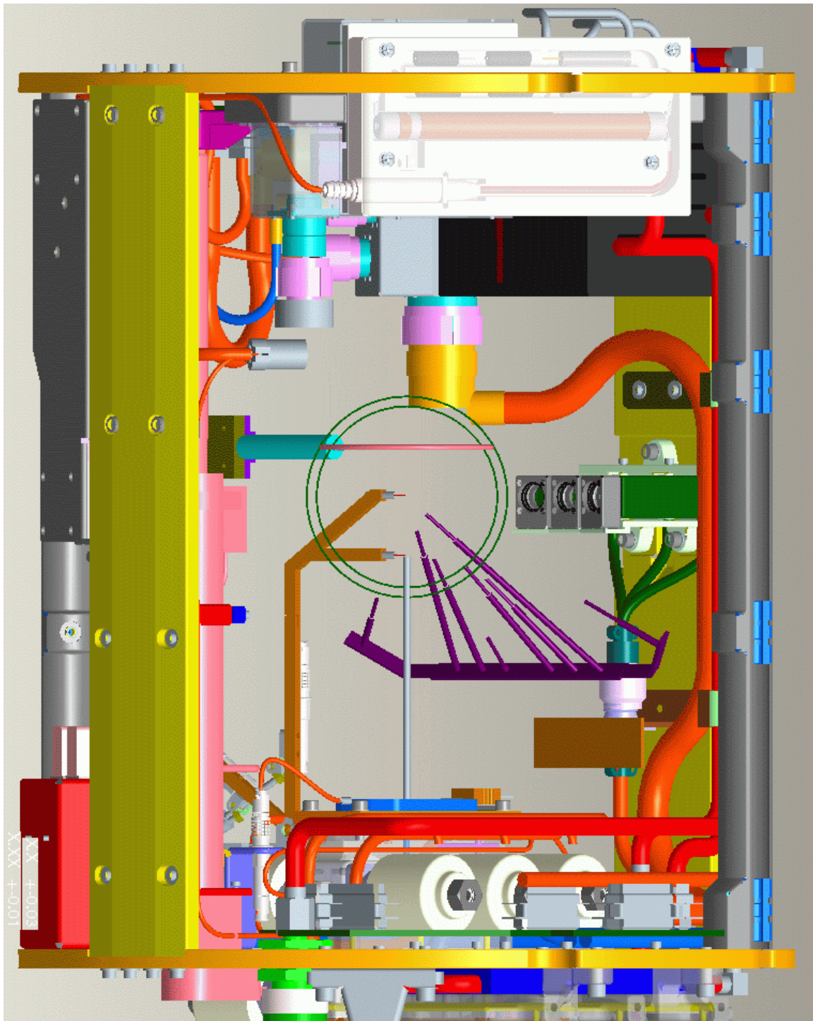
Figure 64. Solid model representation of the chamber insert as seen looking from the ACME Data Camera (DataCam). The thermocouple rake, of which there are two versions, was only used for the spherical flame experiments. To be clear, this figure is not meant to represent the camera's Field of View (FOV).
