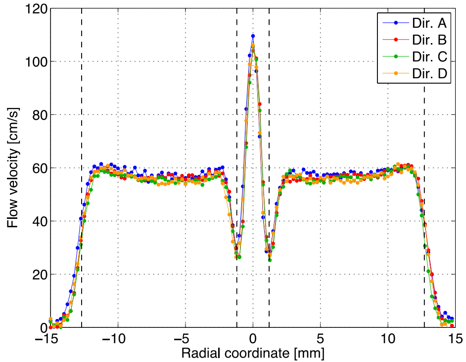
Figure 24. Velocity profiles 0.5 mm downstream of the coflow burner's inner tube with inner and annular velocities intended to be matched at 50 cm/s.
