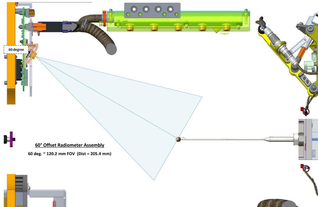
Figure 67. Representation of the offset radiometer's FOV, where that detector is always present. It was primarily intended to support the experiments with spherical flames and features a thermopile detector with a faster response than the other radiometers.
