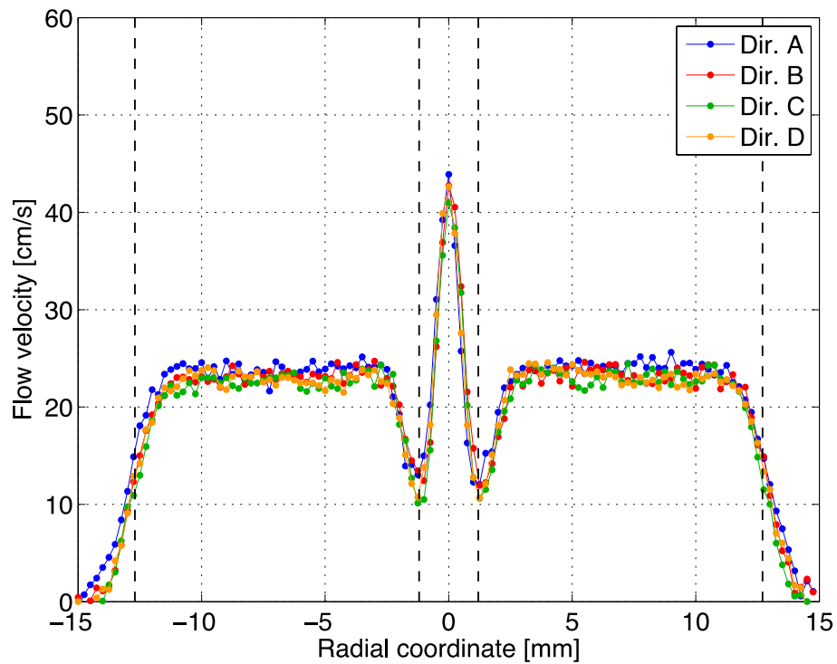
Figure 21. Velocity profiles 0.5 mm downstream of the coflow burner's inner tube with inner and annular velocities intended to be matched at 20 cm/s.
