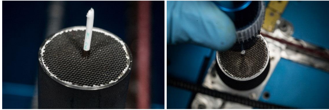
Figure 18. Images from the coflow burner cleaning carried out by astronaut Ricky Arnold on 19 June 2018. In the left image [ISS056e021501], a piece of insulated wire is used to ensure that the inner tube’s interior is unobstructed by soot. In the right image [iss056e021495], a flashlight is used to verify that the honeycomb is not blocked by soot.
