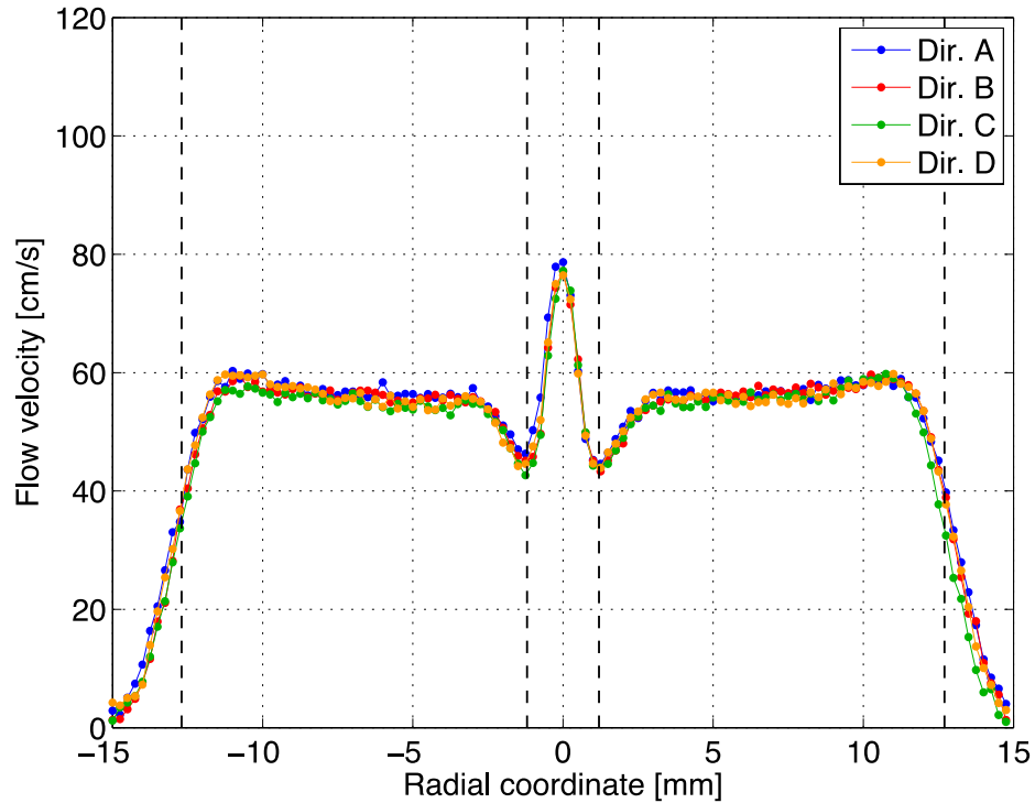
Figure 29. Velocity profiles 5 mm downstream of the coflow burner's inner tube with inner and annular velocities intended to be matched at 50 cm/s.
