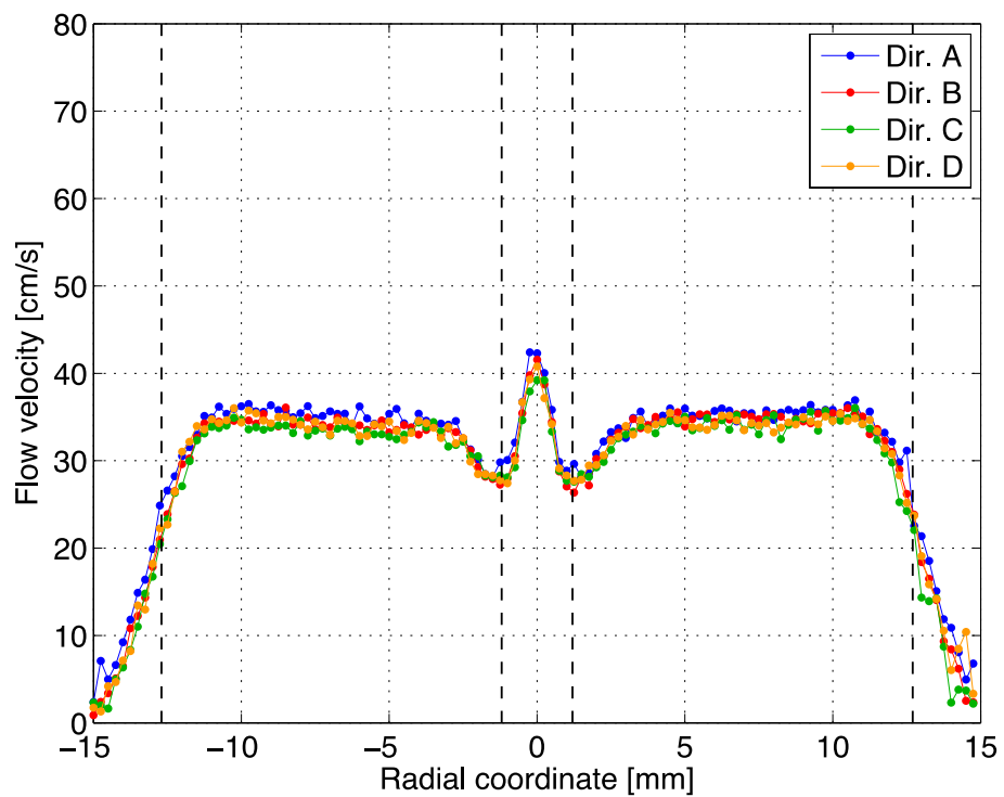
Figure 27. Velocity profiles 5 mm downstream of the coflow burner's inner tube with inner and annular velocities intended to be matched at 30 cm/s.
