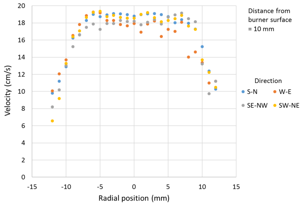
Figure 55. Flow profiles measured for the spaceflight copy of the 25-mm burner.
