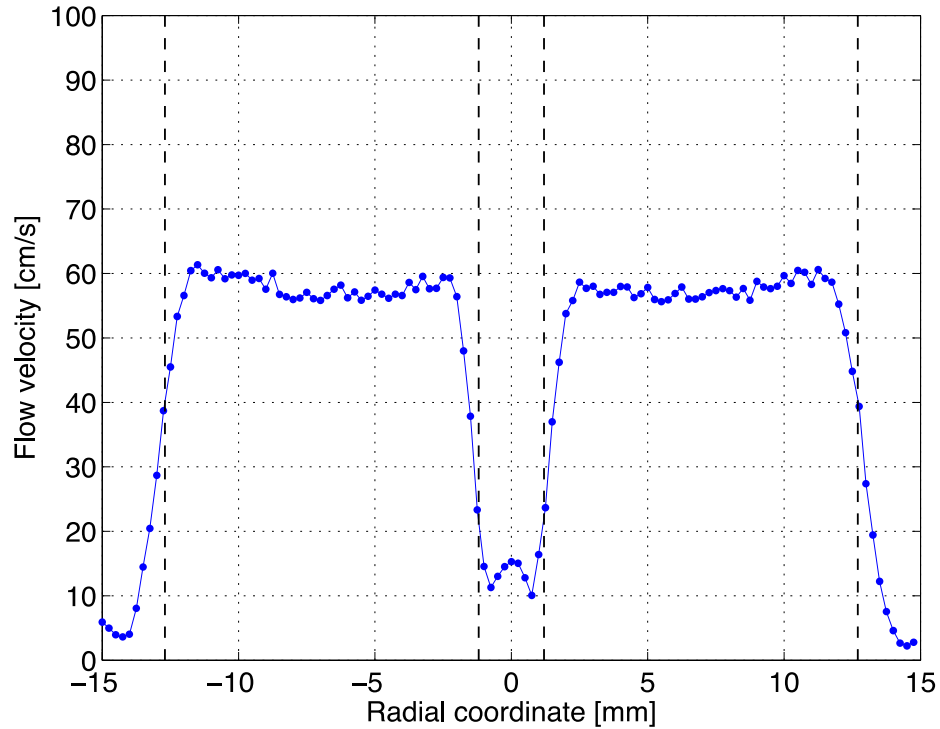
Figure 41. Velocity profiles 0.5 mm downstream of the coflow burner's inner tube with mismatched inner and annular velocities respectively intended to be 10 and 50 cm/s.
