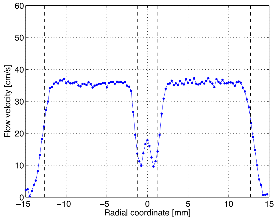
Figure 40. Velocity profiles 0.5 mm downstream of the coflow burner's inner tube with mismatched inner and annular velocities respectively intended to be 10 and 30 cm/s.
