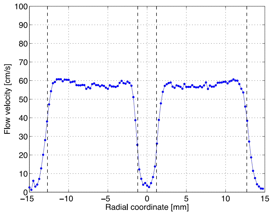
Figure 39. Velocity profiles 0.5 mm downstream of the coflow burner's inner tube with mismatched inner and annular velocities respectively intended to be 0 and 50 cm/s.
