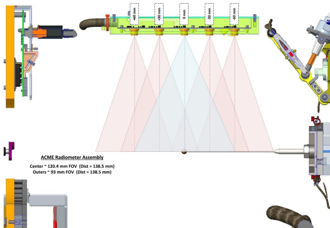
Figure 66. Representation of the FOVs of the five radiometers in the standard linear array. The thermopile detectors are of the same make and model, but the FOV is restricted by an additional aperture (not a lens) in front of each of the four outer radiometers.
