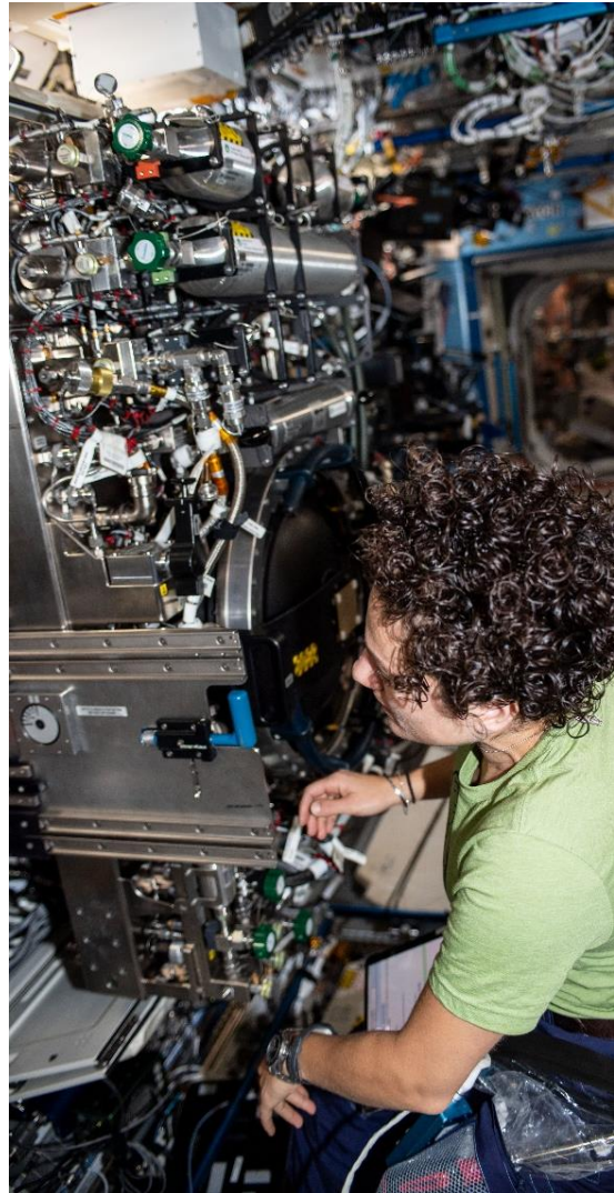
Figure 1. NASA astronaut Jessica Meir working on 24 Oct. 2019 to remove and replace a failed hard drive in one of the CIR's Image Processing and Storage Units (IPSUs). [Cropped detail from ISS061e013306]
