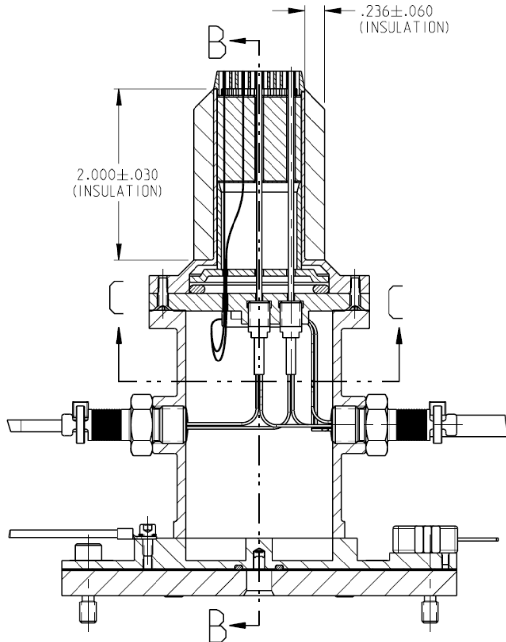
Figure 48. Assembly schematic for the 25-mm BRE burner, a detail from drawing S1101MFA1245. The dimensions for the ceramic insulation are in inches.
