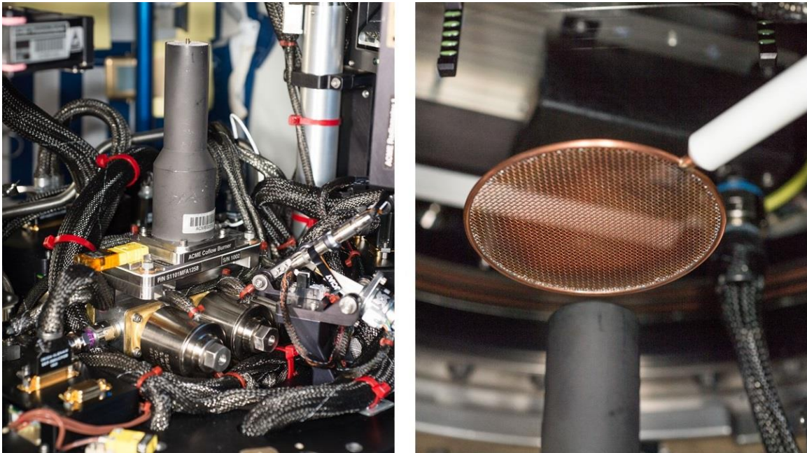
Figure 4: (a) Detail of the ACME chamber insert featuring the coflow burner (in the image center) used by the E-FIELD Flames experiment. This is from a photograph [ISS053e096074] taken by ESA astronaut Paolo Nespoli on 12 Oct. 2017 after he installed the burner on the chamber insert. (b) Detail of the ACME chamber insert where the copper electrode mesh, used by the E-FIELD Flames experiment, can be seen above the coflow burner. This is from a photograph [ISS055e001252] taken by NASA astronaut Scott Tingle on 8 March 2018 following his installation of the electrode mesh.
