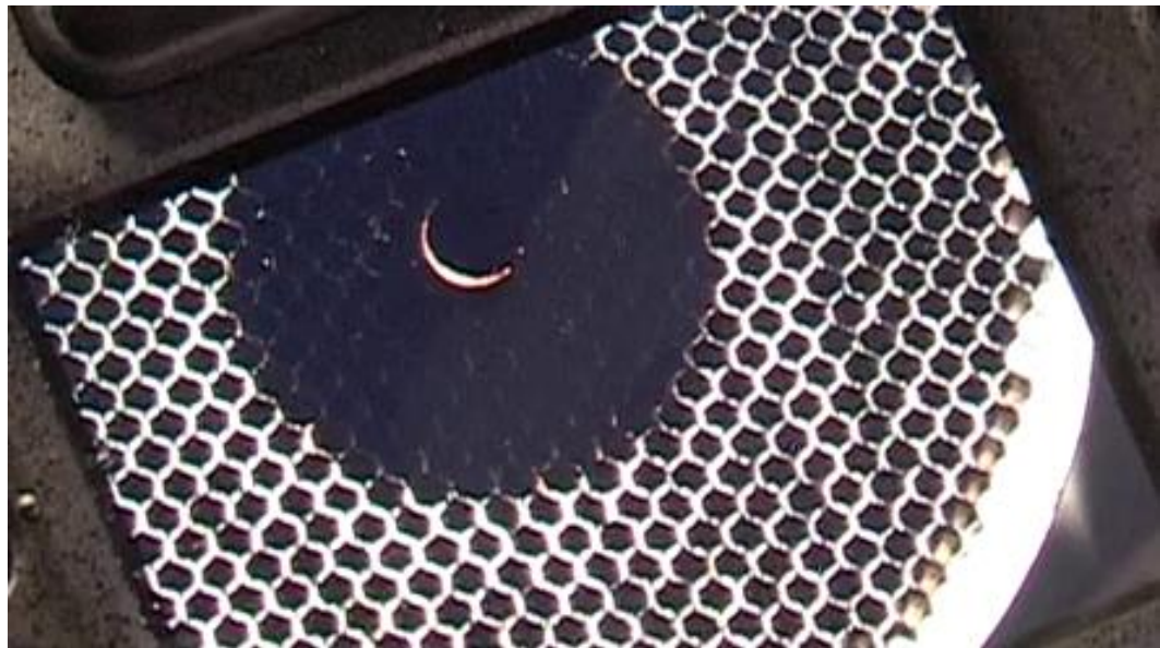
Figure 17. The coflow burner outlet (as seen in the display of a handheld digital camera) from a high-definition video downlink from the ISS on 19 June 2018 prior to the burner cleaning. The central portion of the burner's outlet, including the honeycomb is blackened by soot.
