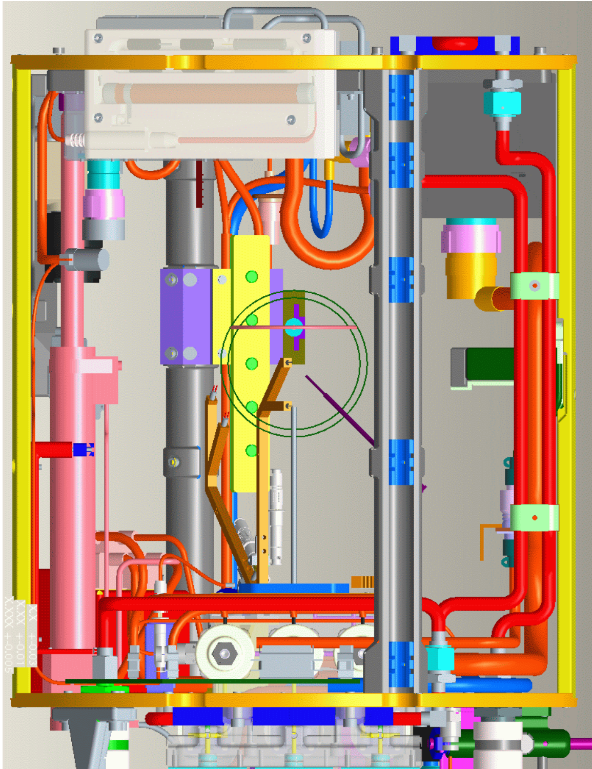
Figure 63. Solid model representation of the chamber insert as seen looking from the direction of the High Bit-depth Multispectral (HiBMs) camera toward the opposing illumination package. Close inspection will reveal that the illumination was significantly blocked in the E-FIELD Flames experiment by the bracket for the electrode mesh. The radiometer array is to the left of the burner and igniter arm (when inserted). To be clear, this figure is not meant to represent the camera's Field of View (FOV).
