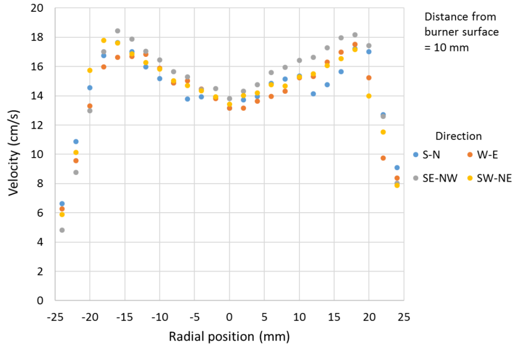
Figure 56. Flow profiles measured for the spaceflight copy of the 50-mm burner.
