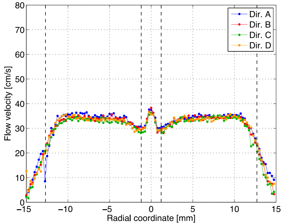
Figure 32. Velocity profiles 10 mm downstream of the coflow burner's inner tube with inner and annular velocities intended to be matched at 30 cm/s.
