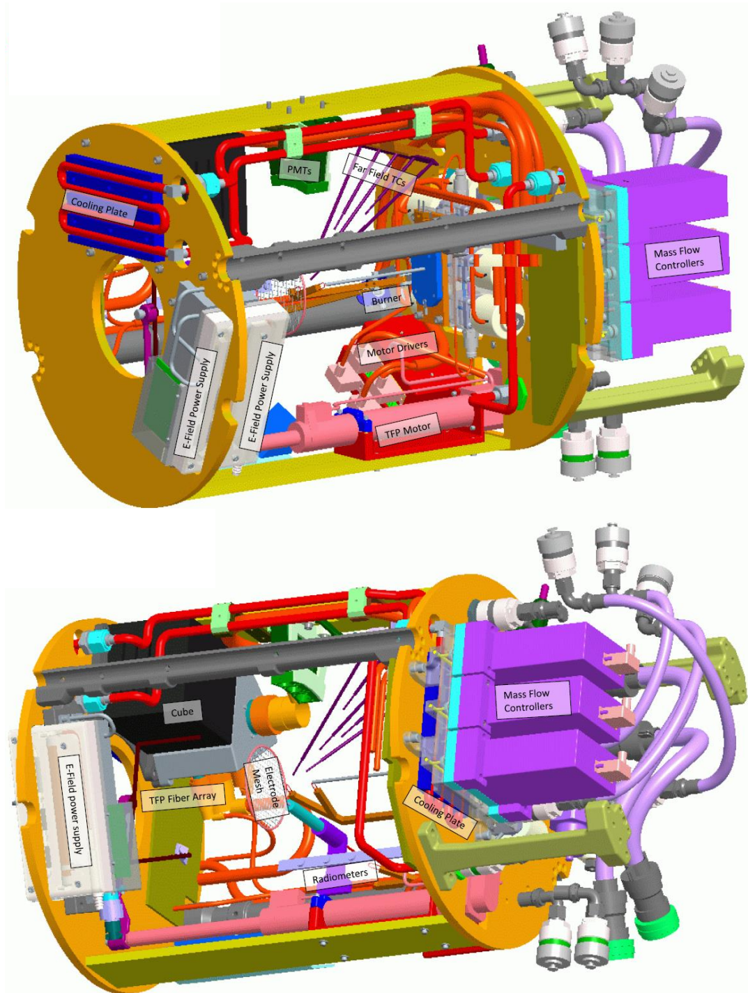
Figure 10. Solid model representation of the chamber insert from two external perspectives.
