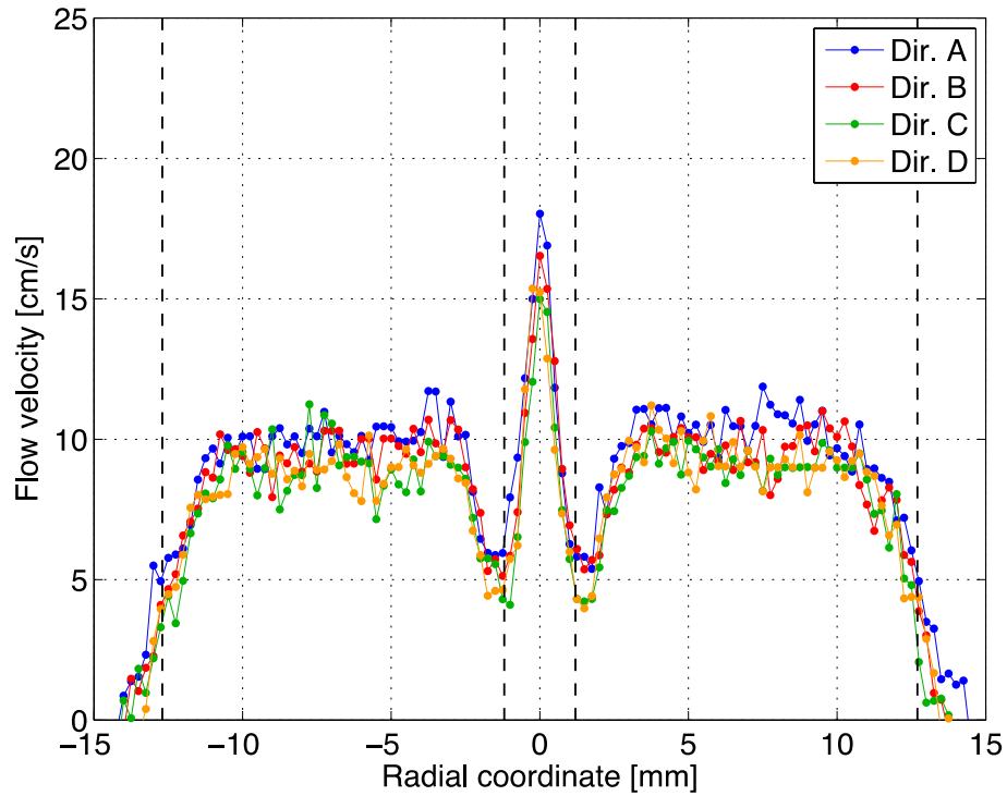
Figure 20. Velocity profiles 0.5 mm downstream of the coflow burner's inner tube with inner and annular velocities intended to be matched at 10 cm/s.
