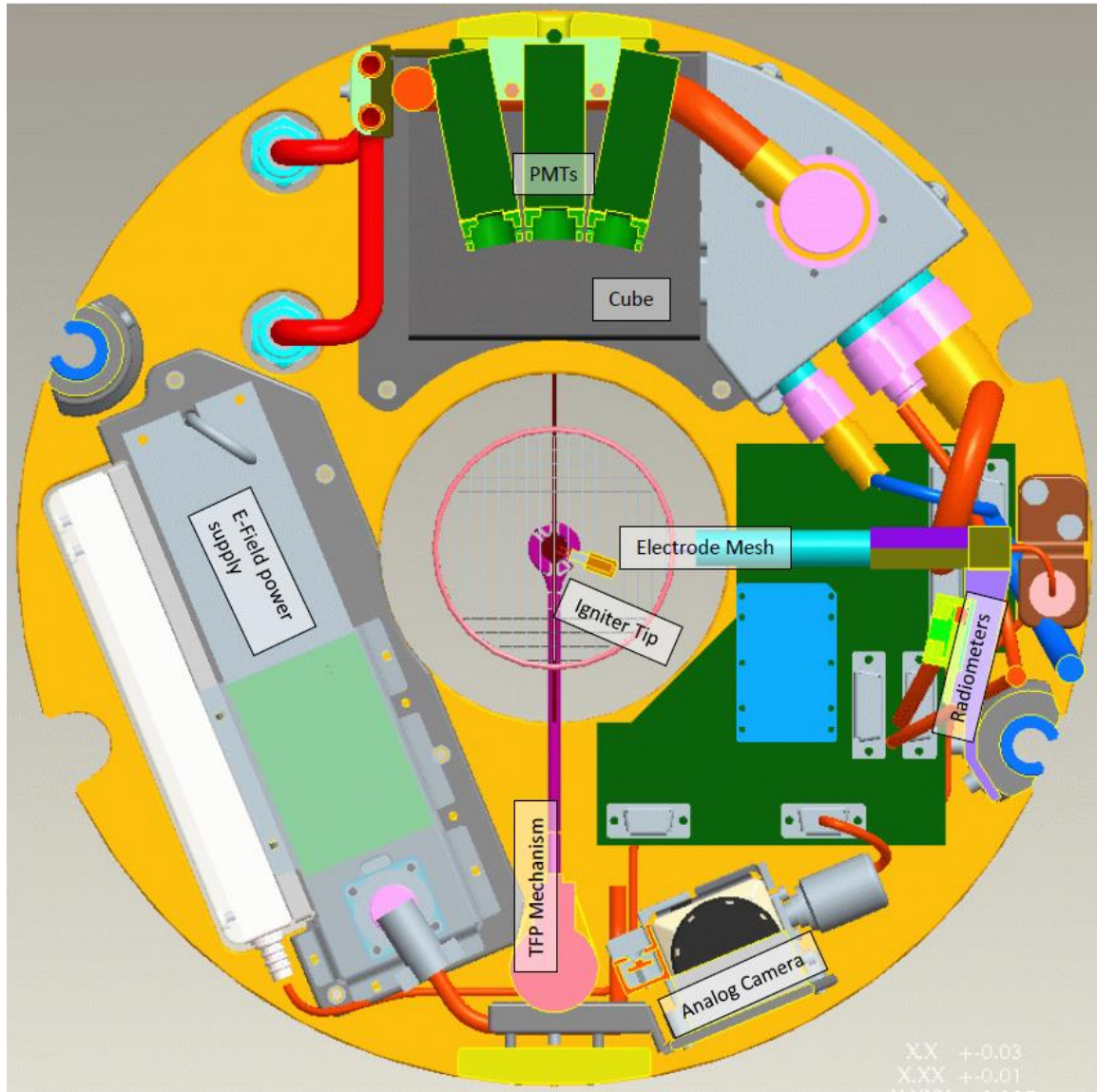
Figure 12. Solid model representation of the chamber insert's interior as seen looking away from the burner toward the opposite end plate. Note that the electrode mesh was only installed for the E-FIELD Flames experiment, where it obstructed use of the Thin Filament Pyrometry (TFP) fiber array. Furthermore, its mounting bracket interfered with illumination for possible soot volume fraction measurements via light extinction.
