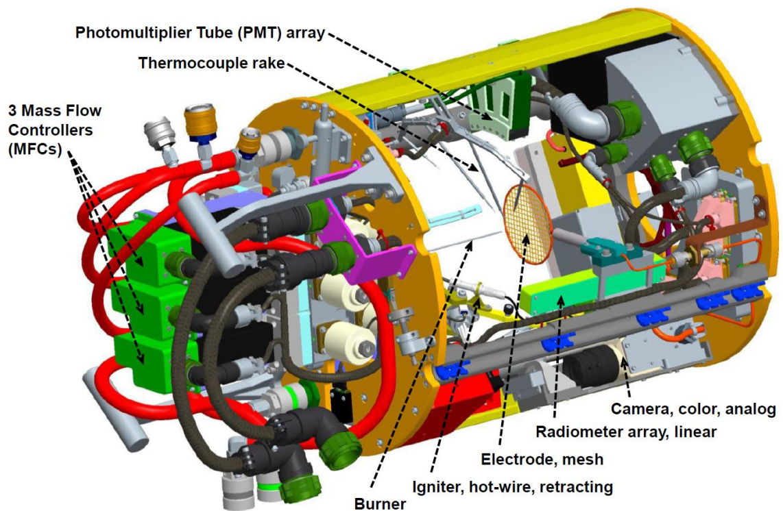
Figure 3: Solid model representation of the ACME chamber insert.
