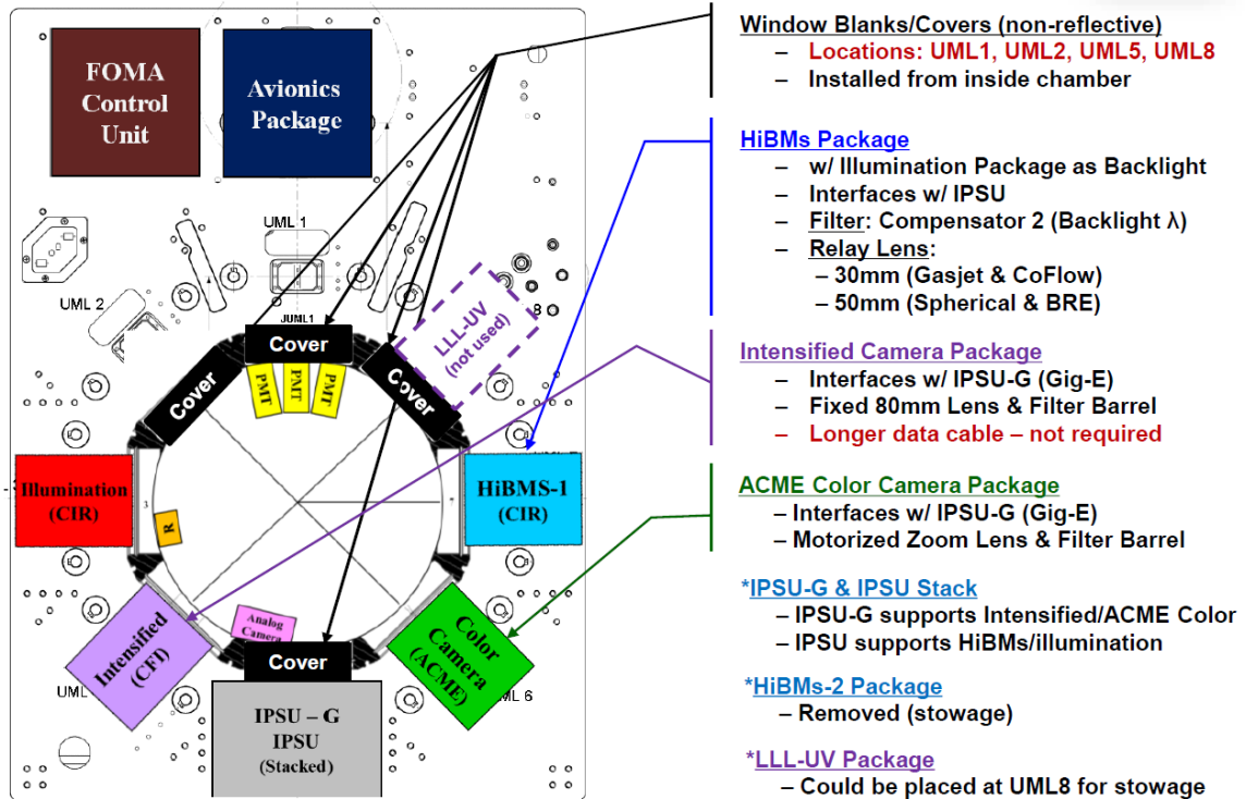
Figure 60. Optical arrangement for all ACME investigations except the Structure and Response of Spherical Diffusion Flames (s-Flame) experiment.
