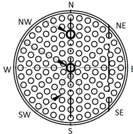
Figure 54. Drawing detail showing the arrangement of the four lines, N-S, NE-SW, E-W, and SE-NW, along which flow profiles were measured prior to launch. In this arrangement, the offset heat flux transducer is to the north (N), while the two separate thermocouples are to the south (S).
