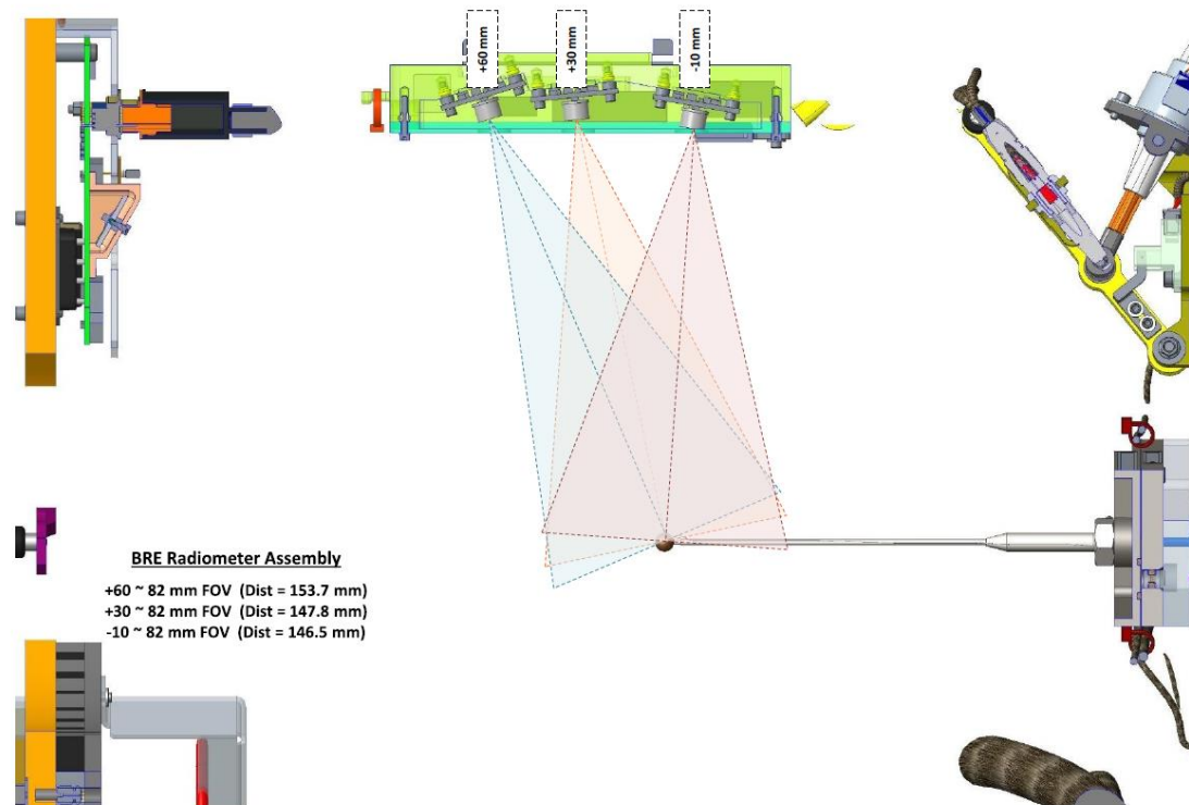
Figure 68. Representation of the FOVs for the Burning Rate Emulator (BRE) radiometer array, which was used in place of the standard radiometer array during BRE's first round of testing.
