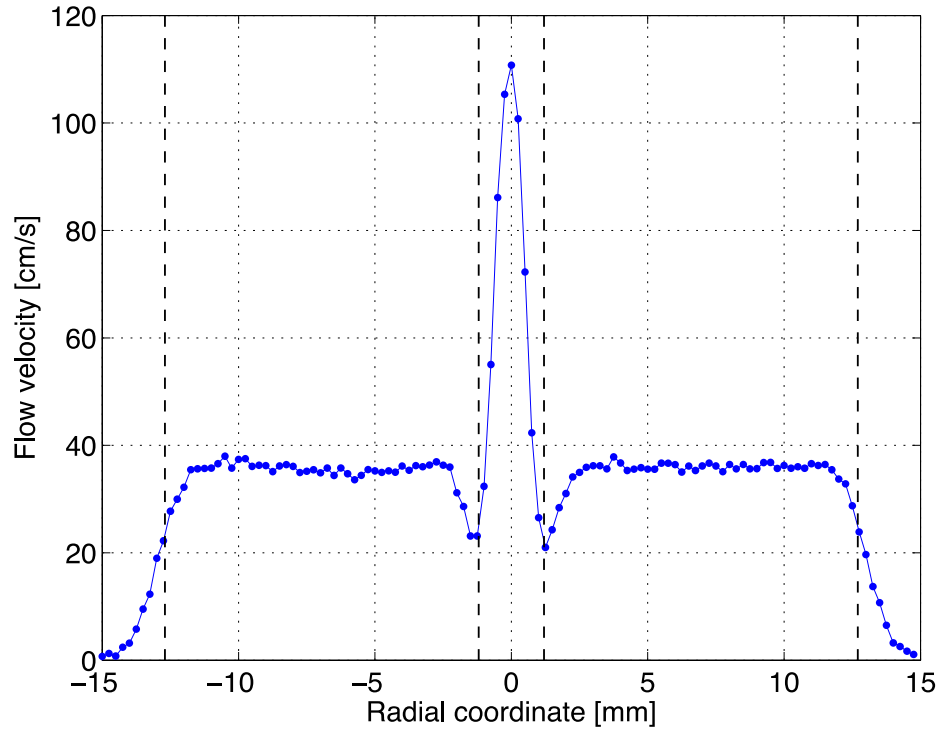
Figure 45. Velocity profiles 0.5 mm downstream of the coflow burner's inner tube with mismatched inner and annular velocities respectively intended to be 50 and 30 cm/s.
