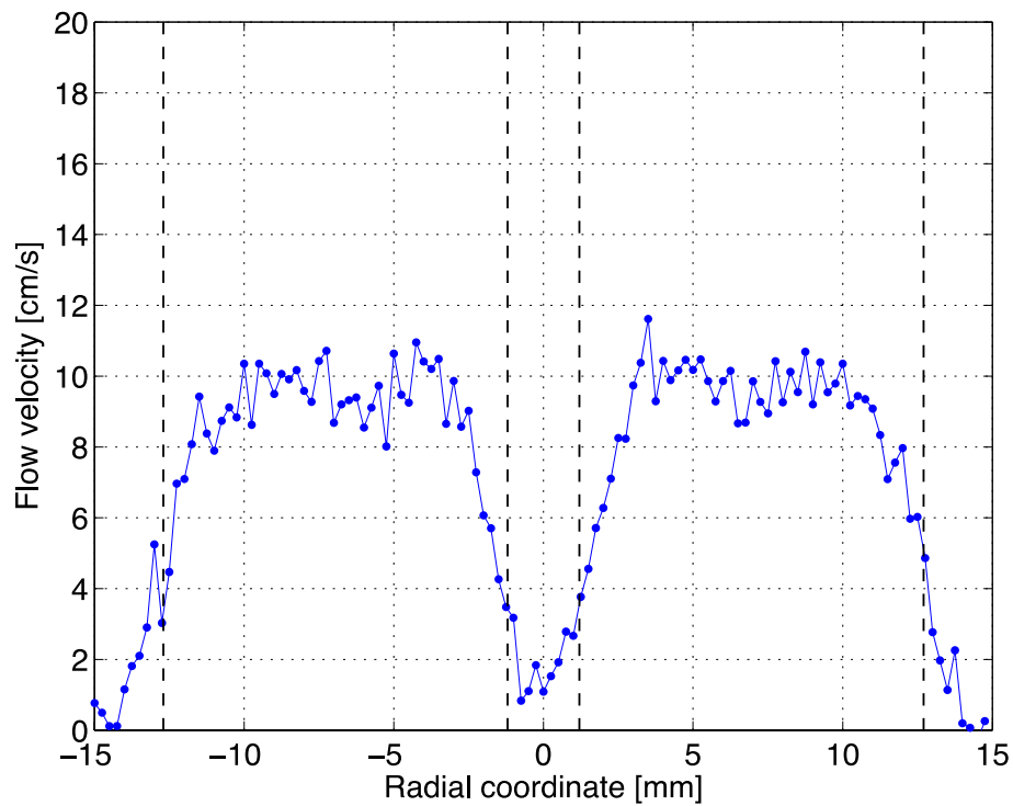
Figure 35. Velocity profiles 0.5 mm downstream of the coflow burner's inner tube with mismatched inner and annular velocities respectively intended to be 0 and 10 cm/s.
