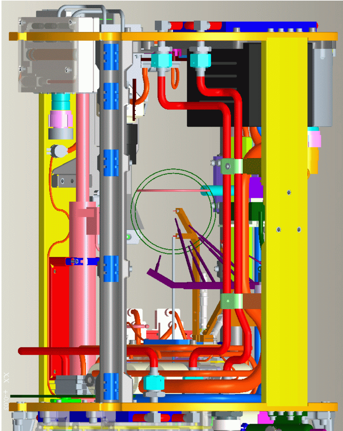
Figure 62. Solid model representation of the chamber insert as seen looking from the Low Light Level Ultraviolet (LLL-UV) camera, which has only been used for the s-Flame experiment. Similarly, the thermocouple rake, of which there are two versions, was only used for spherical flame experiments. To be clear, this figure is not meant to represent the camera's Field of View (FOV).
