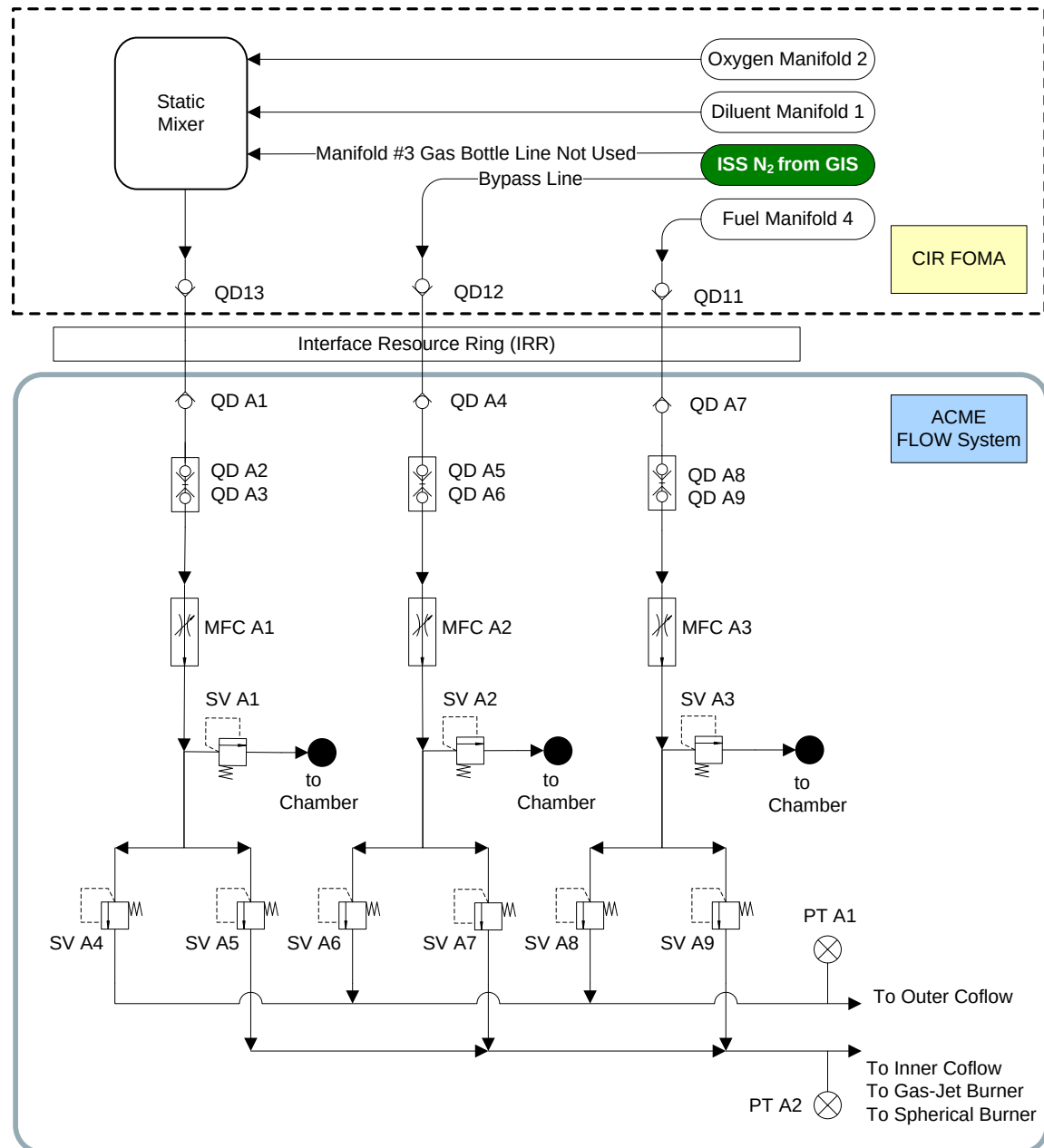
Figure 13. Schematic of gas delivery in ACME testing, where the FOMA is the CIR's Fuel and Oxidizer Management Assembly.
