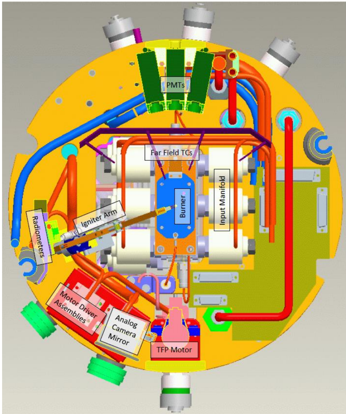
Figure 11. Solid model representation of the chamber insert's interior as seen looking toward the burner and the end plate on which it is mounted.
