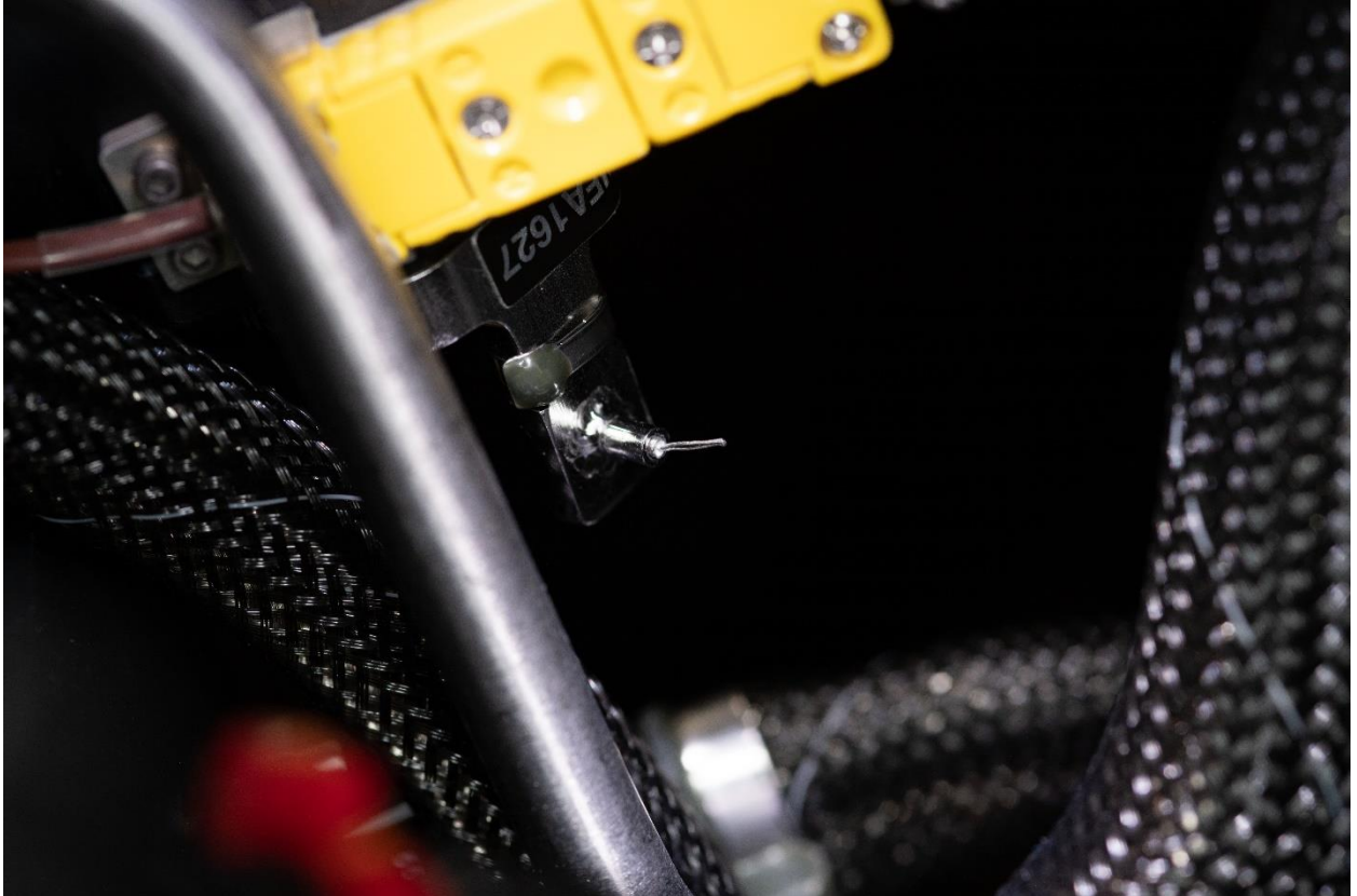
Figure 70. Bent relay-side thermocouple, meant to be 200 mm from the center of the spherical burner's porous sphere, as seen on 19 Sept. 2018 when the chamber insert was reconfigured for the second round of E-FIELD Flames testing. The bent length of exposed wire is 5 mm long. [ISS056e177654]
