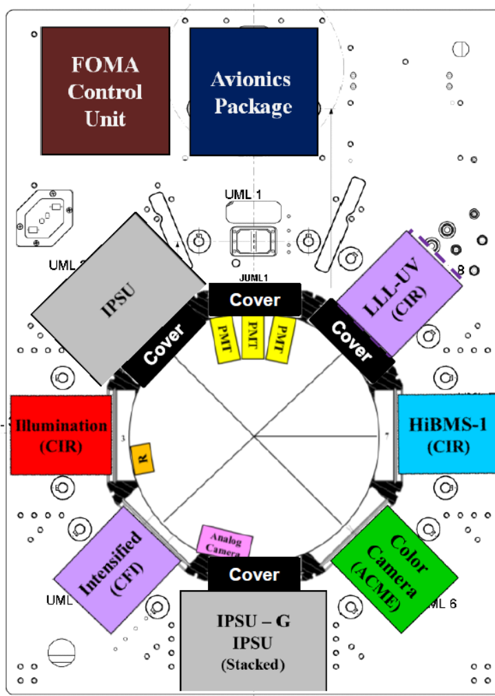
Figure 59: Full layout of the cameras and optical instrumentation, showing the location of the Fuel and Oxidizer Management Assembly (FOMA) control unit, avionics package, Low Light Level Ultraviolet (LLL-UV) camera, High Bit-depth Multispectral (HiBMs) camera and the opposing illumination package, the color ACME Data Camera (DataCam), the Image Processing and Storage Unit for Gigabit ethernet (IPSU-G) cameras (IPSU-G), the two standard IPSUs, the Cool Flame Investigation (CFI) intensified cameras, the internal window covers (as installed when not using the LLL-UV camera), array of three Photomultiplier Tubes (PMTs), analog operations camera, and the array of radiometers (simply marked 'R').
