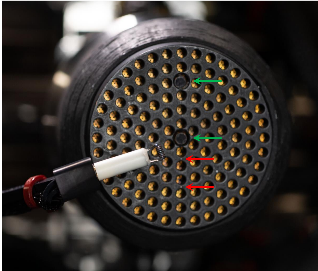
Figure 49. The 50-mm BRE burner with a coil-type igniter tip inserted above it during set-up by astronaut Chris Cassidy on 27 Aug. 2020. The center and offset heat flux transducers, which include thermocouples, are within openings in the perforated outlet plate and pointed out by green arrows. The tips of two additional thermocouples are visible as faint dots between holes in the black outlet below the transducers, as pointed out by the red arrows. [Cropped detail from ISS063e078811]
