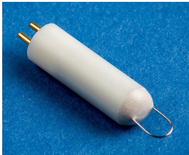
Figure 57. A standard ACME igniter tip prior to launch. The igniter tip's white ceramic insulator is 4.75 mm in diameter and the pin-to-pin spacing (as measured from their centers) is 2 mm.
