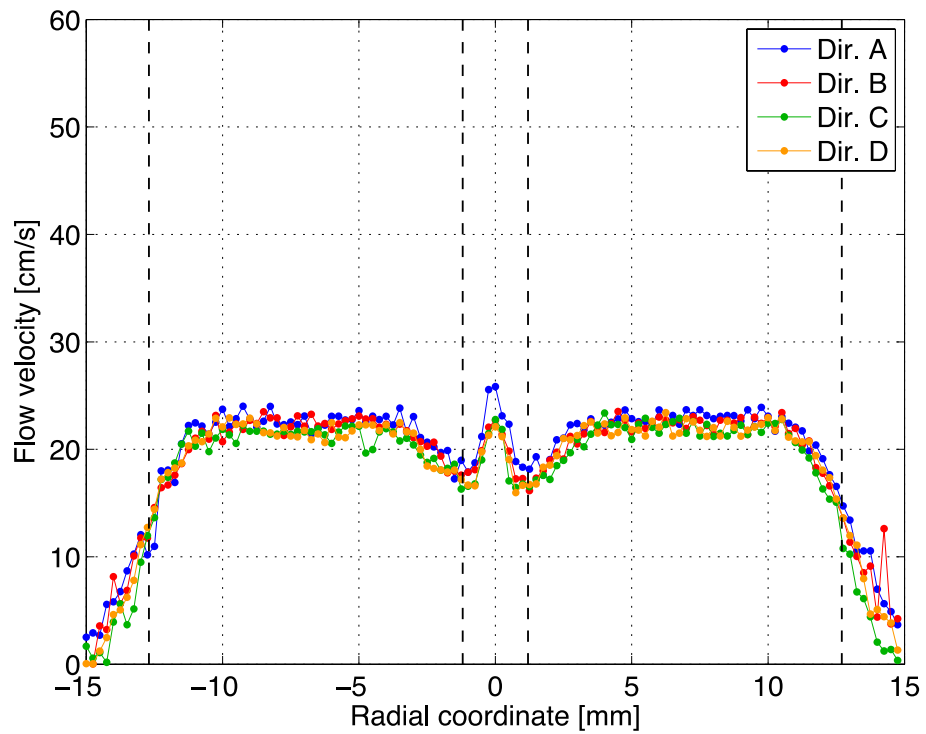
Figure 26. Velocity profiles 5 mm downstream of the coflow burner's inner tube with inner and annular velocities intended to be matched at 20 cm/s.
