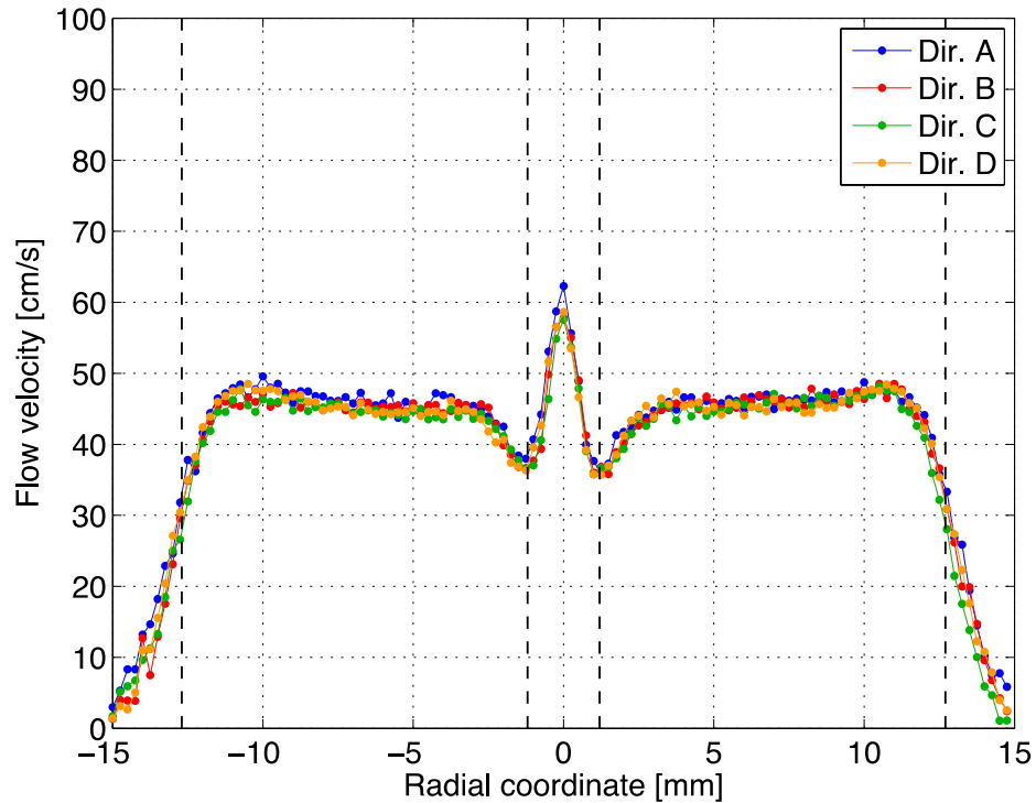
Figure 28. Velocity profiles 5 mm downstream of the coflow burner's inner tube with inner and annular velocities intended to be matched at 40 cm/s.
