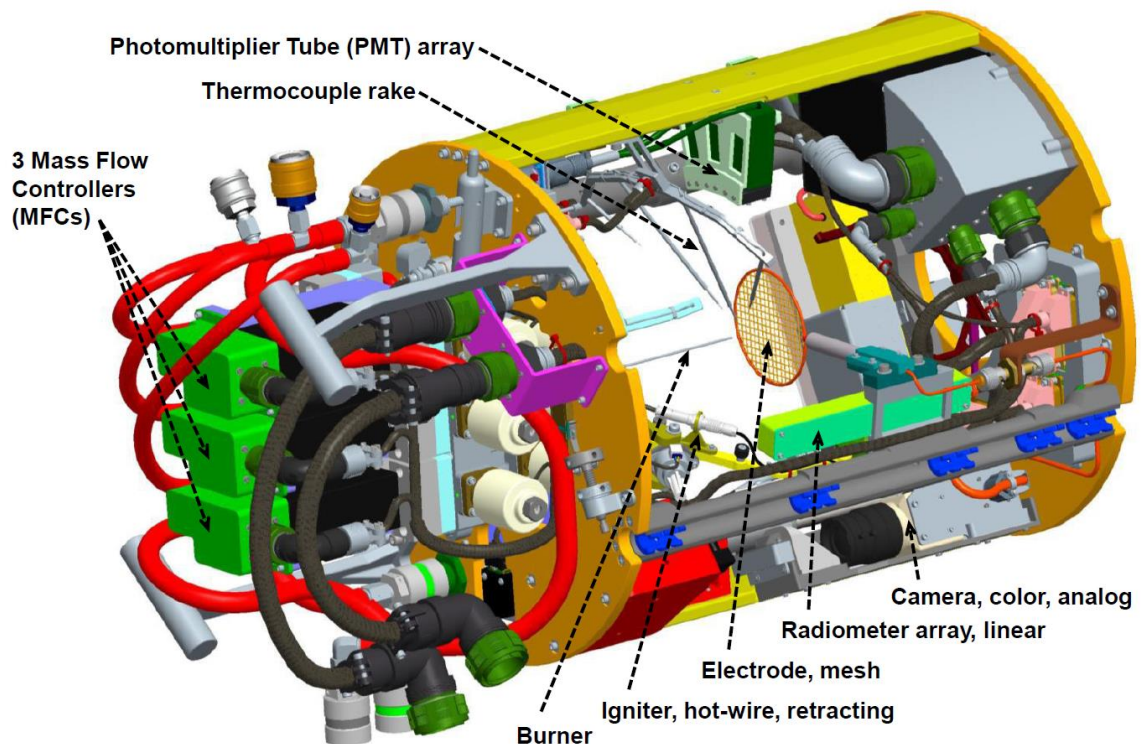
Figure 2: Design of the Advanced Combustion via Microgravity Experiments (ACME) chamber insert that will be used in the Combustion Integrated Rack (CIR) on ISS.
