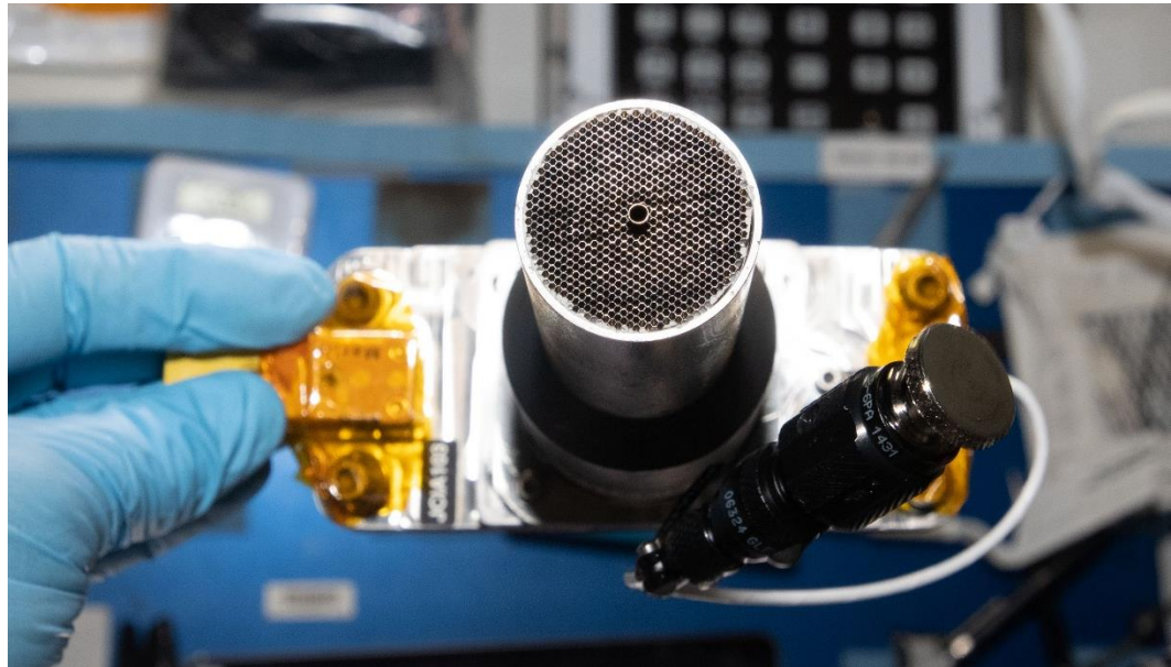
Figure 15. The coflow burner aboard the space station, where the inner tube extends downstream of the annular outlet featuring a fine honeycomb. The white cable with the black connector on the right is for grounding, while the yellow connector on the left was used to secure the cable for the burner thermocouple, even though the coflow burner isn't equipped with a thermocouple. [Cropped detail from ISS064e028847]
