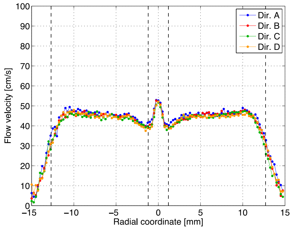
Figure 33. Velocity profiles 10 mm downstream of the coflow burner's inner tube with inner and annular velocities intended to be matched at 40 cm/s.
