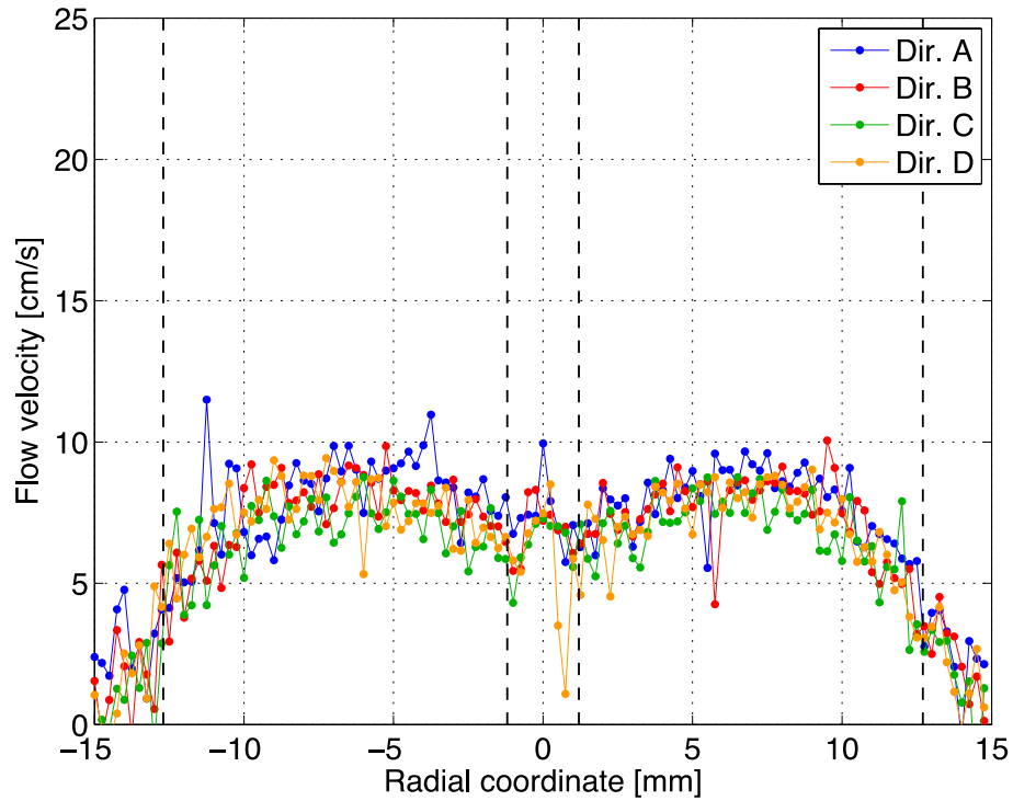
Figure 30. Velocity profiles 10 mm downstream of the coflow burner's inner tube with inner and annular velocities intended to be matched at 10 cm/s.
