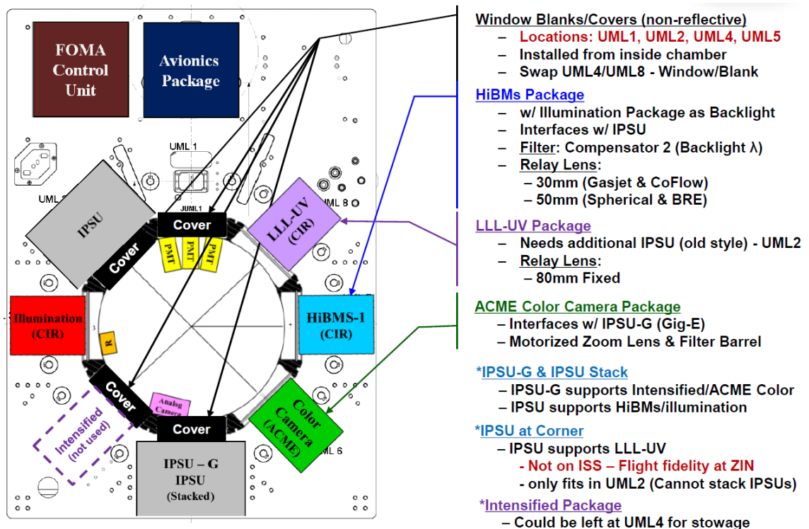
Figure 61. Optical arrangement for ACME's Structure and Response of Spherical Diffusion Flames (s-Flame) experiment, with the important exception that the CFI intensified camera was used for s-Flame and was not blocked with an internal window cover.
