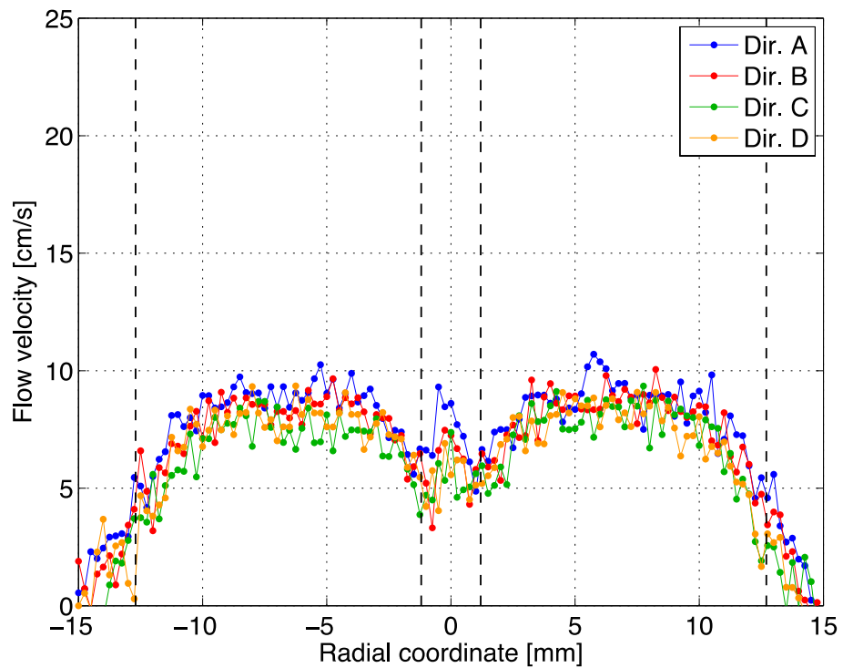
Figure 25. Velocity profiles 5 mm downstream of the coflow burner's inner tube with inner and annular velocities intended to be matched at 10 cm/s.
