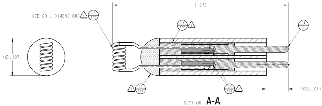
Figure 58. Coil type igniter from details in drawing S1101MFA1339, where the dimensions are in inches.
