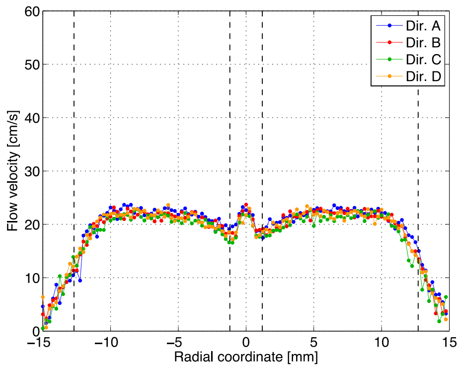
Figure 31. Velocity profiles 10 mm downstream of the coflow burner's inner tube with inner and annular velocities intended to be matched at 20 cm/s.
