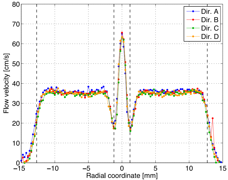
Figure 22. Velocity profiles 0.5 mm downstream of the coflow burner's inner tube with inner and annular velocities intended to be matched at 30 cm/s.
