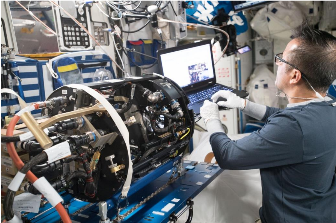
Figure 2: NASA astronaut Joe Acaba reviewing procedures to align the hot-wire igniter on the ACME chamber insert to his left, in a photograph [ISS054e014660] taken by NASA astronaut Mark Vande Hei on 5 Jan. 2018.
