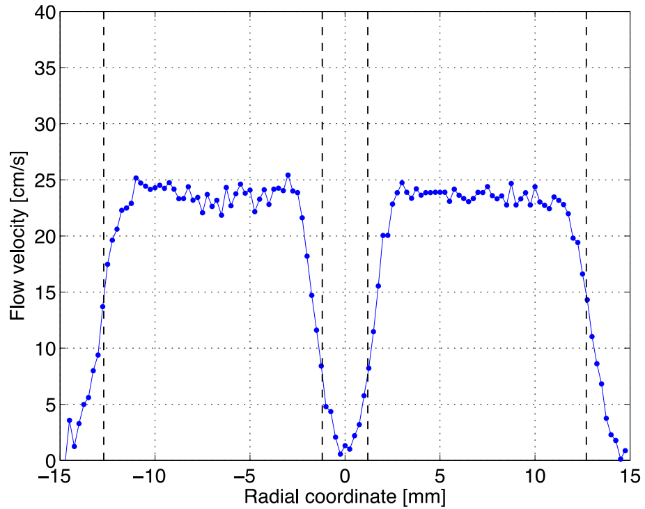
Figure 36. Velocity profiles 0.5 mm downstream of the coflow burner's inner tube with mismatched inner and annular velocities respectively intended to be 0 and 20 cm/s.
