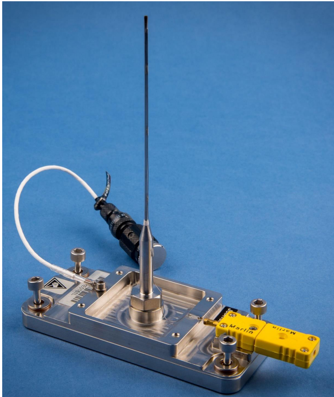
Figure 14. A gas-jet burner prior to launch. The white cable on the left was for grounding, while the yellow connector is for the burner's type-K thermocouple.
