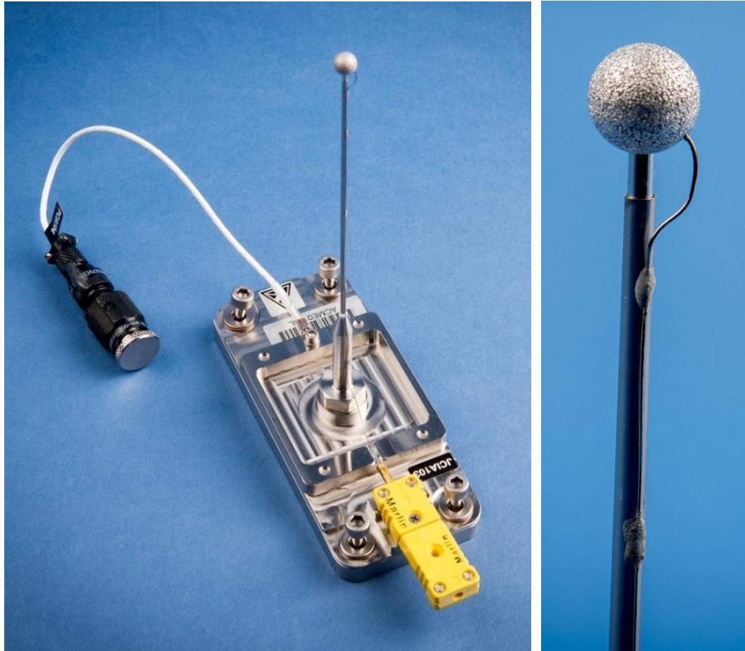
Figure 46. A spherical burner, prior to launch, showing the positioning of the slightly embedded thermocouple. The gap between the support tube and porous sintered sphere can also be seen. The white cable with the black connector on the left is for grounding, while the yellow connector is for the type-K thermocouple.
