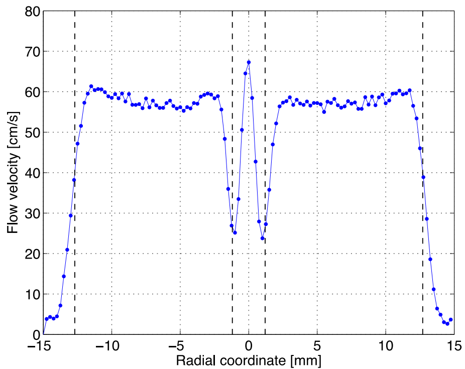
Figure 43. Velocity profiles 0.5 mm downstream of the coflow burner's inner tube with mismatched inner and annular velocities respectively intended to be 30 and 50 cm/s.
