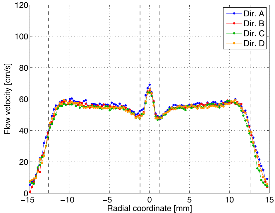
Figure 34. Velocity profiles 10 mm downstream of the coflow burner's inner tube with inner and annular velocities intended to be matched at 50 cm/s.
