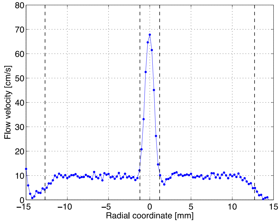
Figure 42. Velocity profiles 0.5 mm downstream of the coflow burner's inner tube with mismatched inner and annular velocities respectively intended to be 30 and 10 cm/s.
