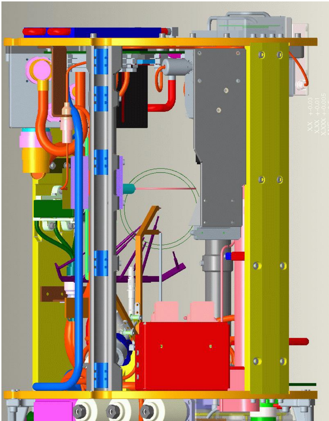
Figure 65. Solid model representation of the chamber insert as seen looking from the Cool Flames Investigation (CFI) intensified camera. The thermocouple rake, of which there are two versions, was only used for the spherical flame experiments. To be clear, this figure is not meant to represent the camera's Field of View (FOV).
