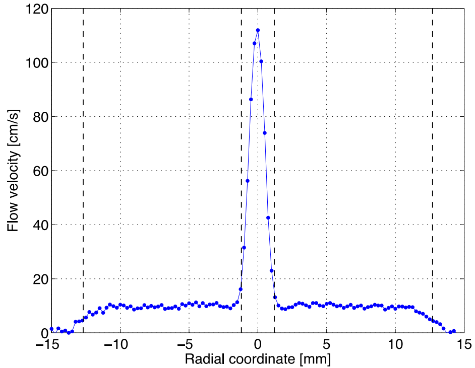
Figure 44. Velocity profiles 0.5 mm downstream of the coflow burner's inner tube with mismatched inner and annular velocities respectively intended to be 50 and 10 cm/s.
