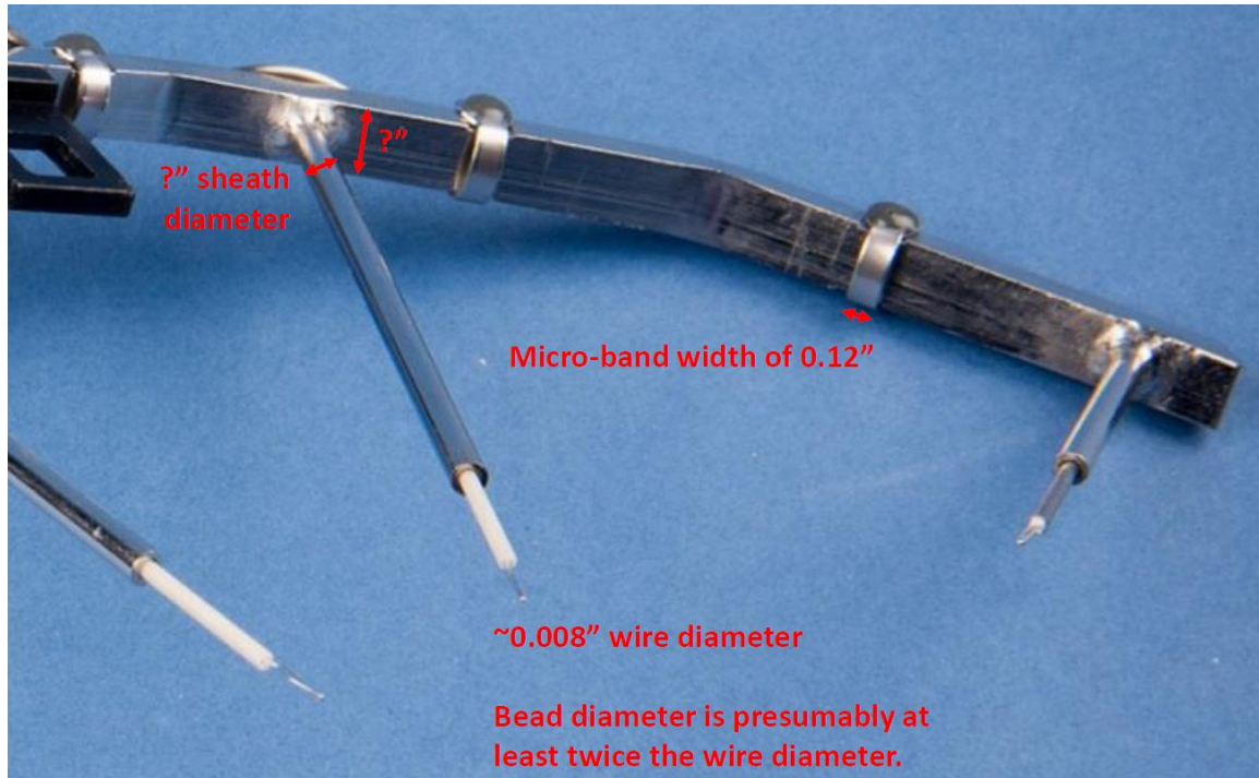
Figure 69. Thermocouple rake dimensions.
