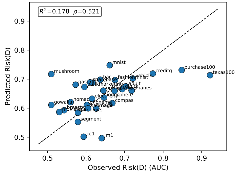
Linear Regression (LOO-CV)
