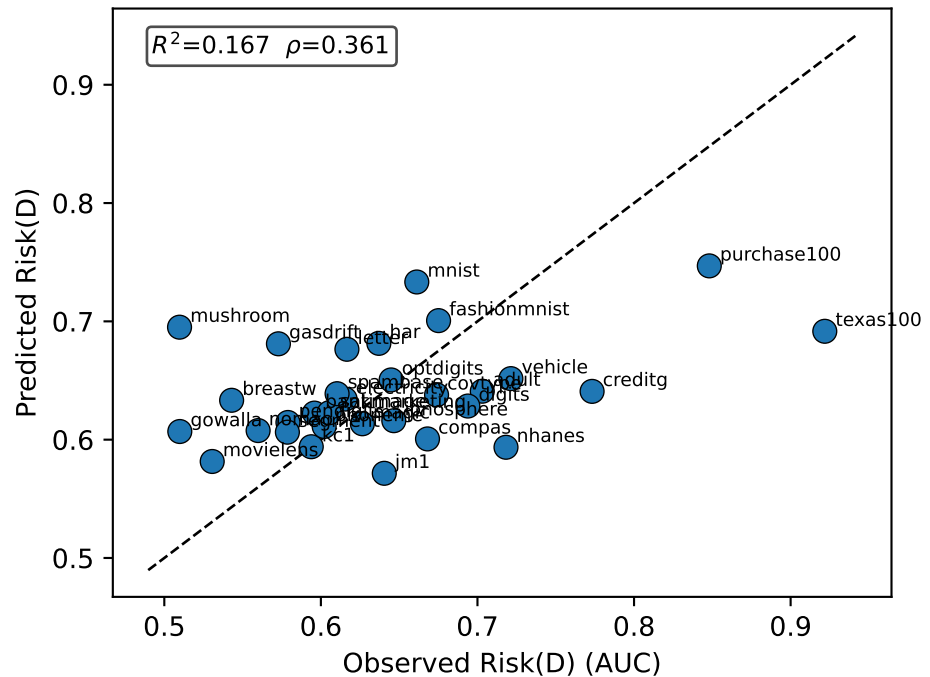
Random Forest (LOO-CV)
