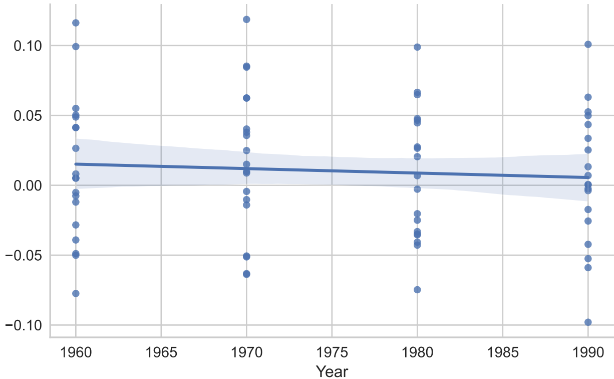
Embedding Bias
