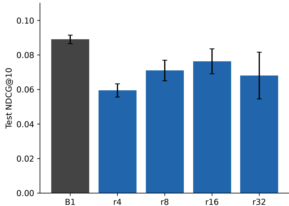
Full / low-rank federated models (5 seeds)
