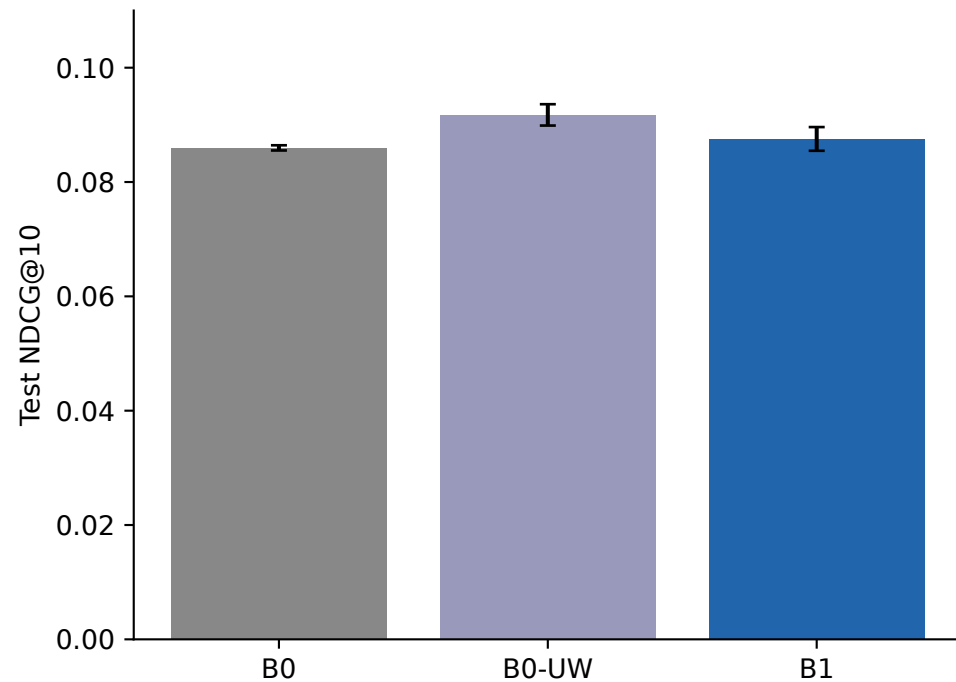
Centralized / federated controls (3 seeds)
