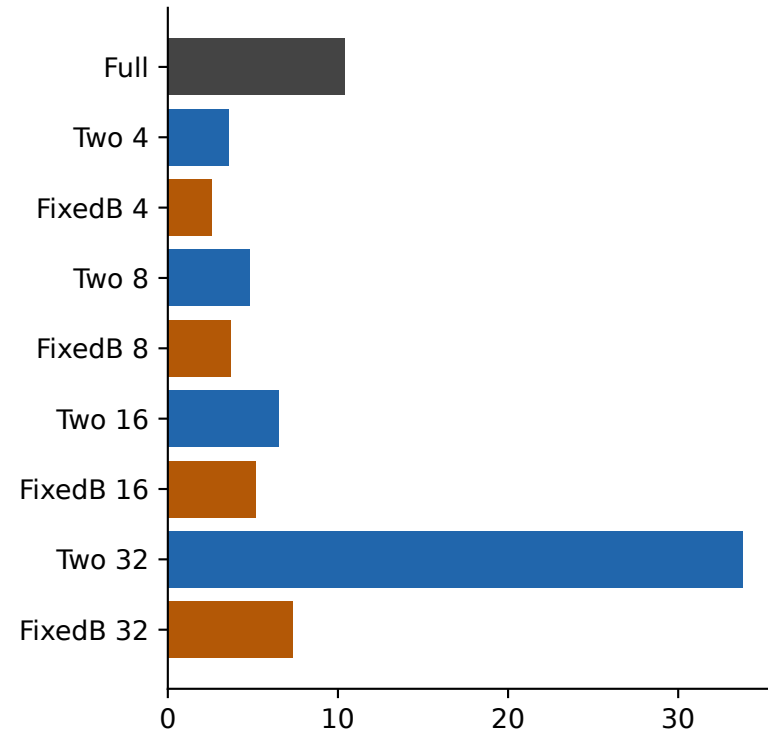
Item-matrix shock RMS
