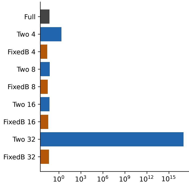
Score shock RMSE (log scale)
