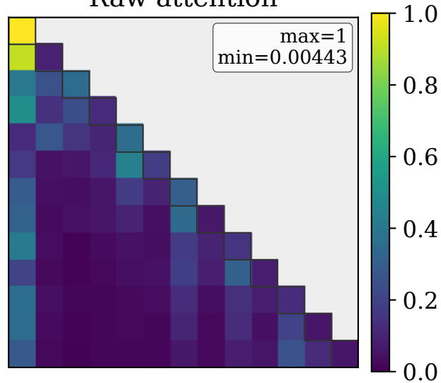
Raw attention
