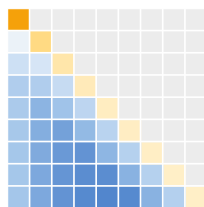
Baseline Attention
