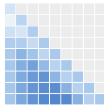
Diagonal-suppressed
