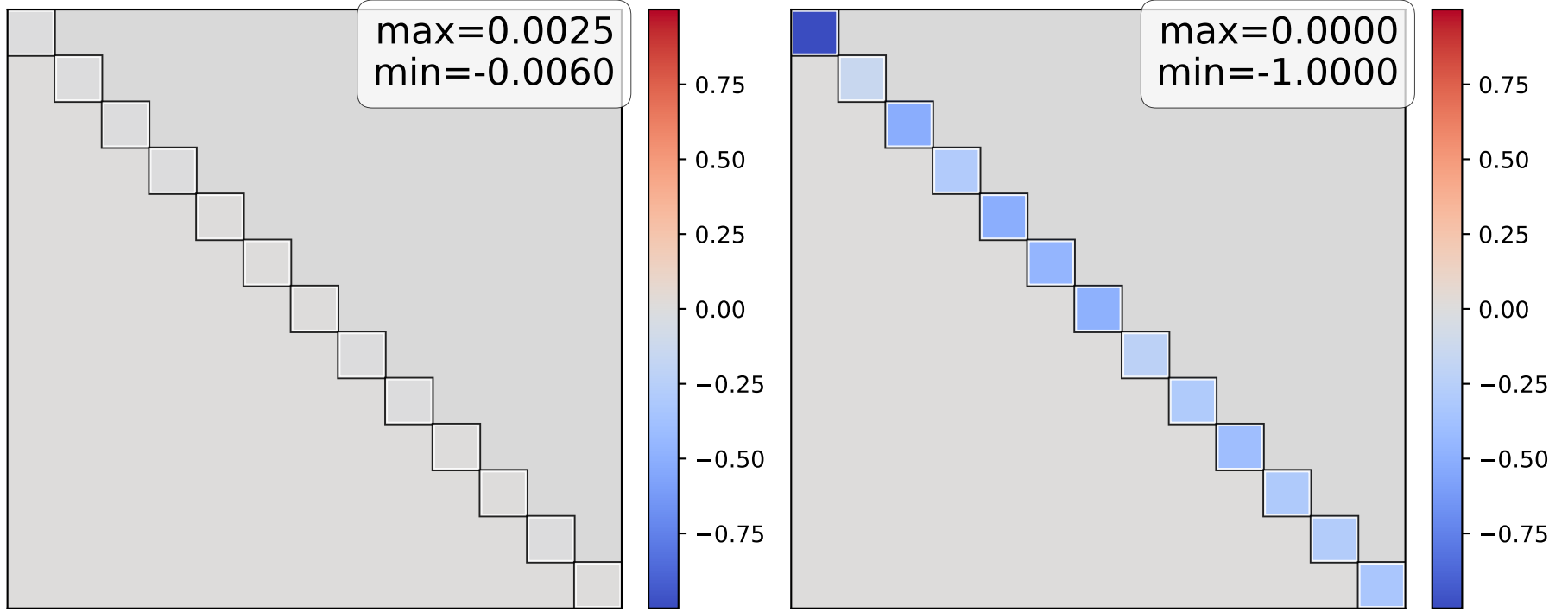
Qwen3-4B Layer 19 Head 6 residual-based Qwen3-4B Layer 19 Head 6 value-based diag delta
