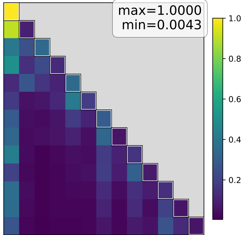
Baseline Attention
