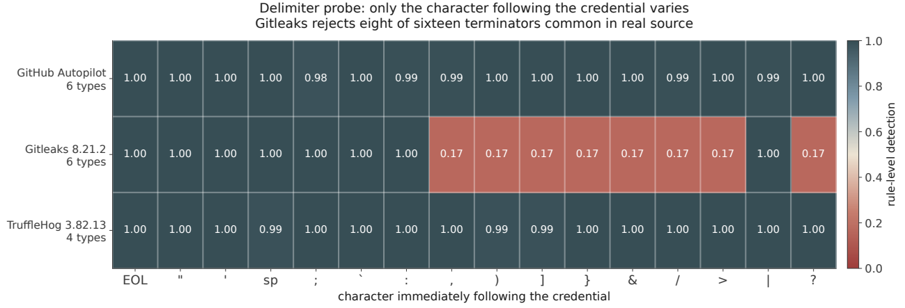
Fig. 8. Delimiter probe: only the character immediately following the credential varies. Gitleaks rejects eight of sixteen terminators that occur routinely in real source.
