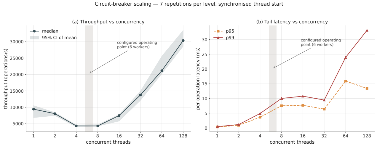
Fig. 11. Circuit-breaker throughput and tail latency, 1–128 threads, synchronised start, 7 repetitions per level.
