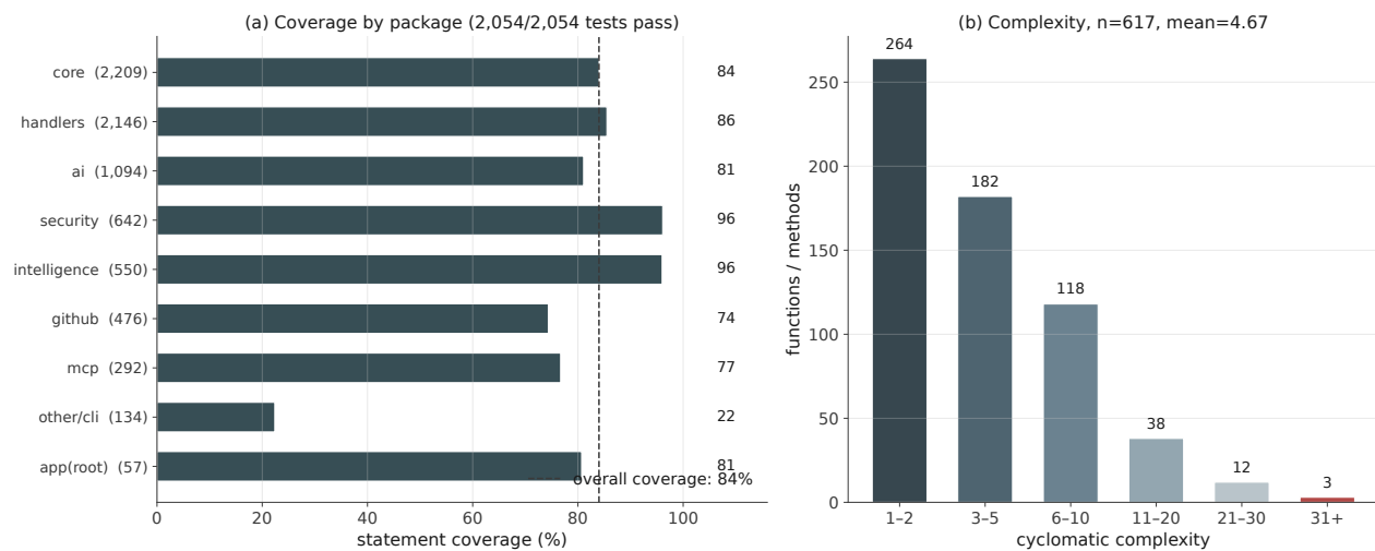
Fig. 14. Statement coverage by package and cyclomatic-complexity distribution for the primary subject.
