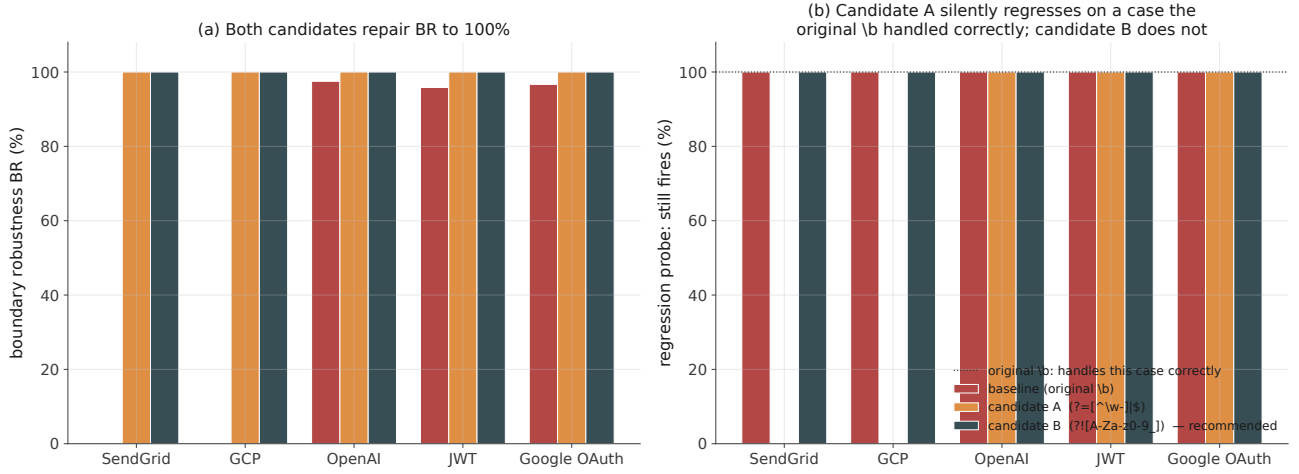
Fig. 6. Fix validation. (a) Both candidates repair boundary robustness to 1.0 on all five affected rules. (b) A regression probe — a credential ending in a word character, followed by a hyphen — that the original rule handled correctly. Candidate A silently fails it on the two fixed-count-quantifier rules; Candidate B does not.
