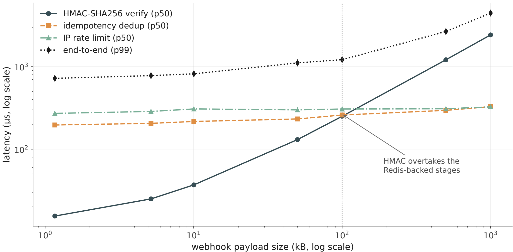
Ingress pipeline latency versus payload size
