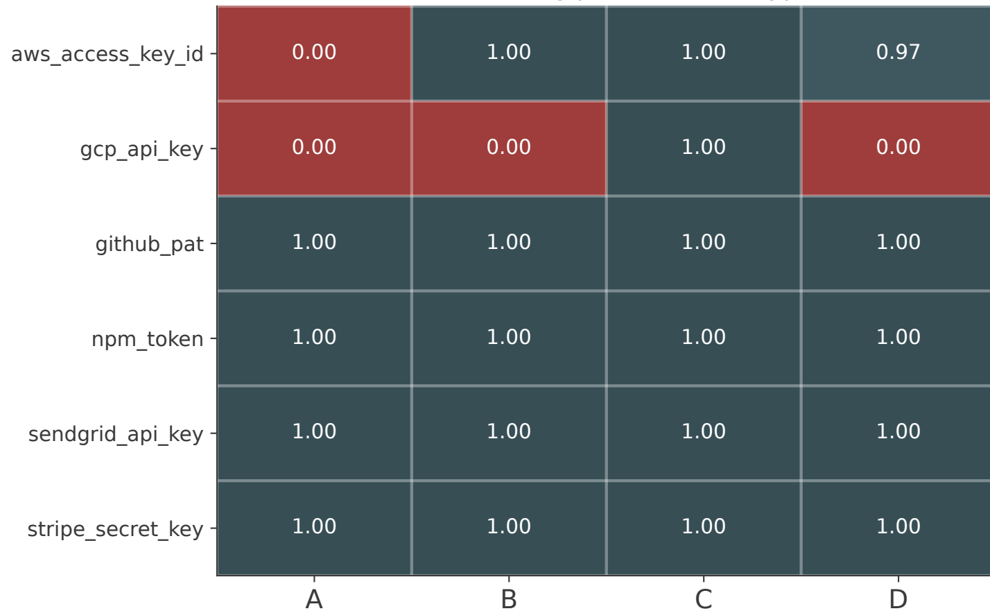
(b) TruffleHog per credential type
