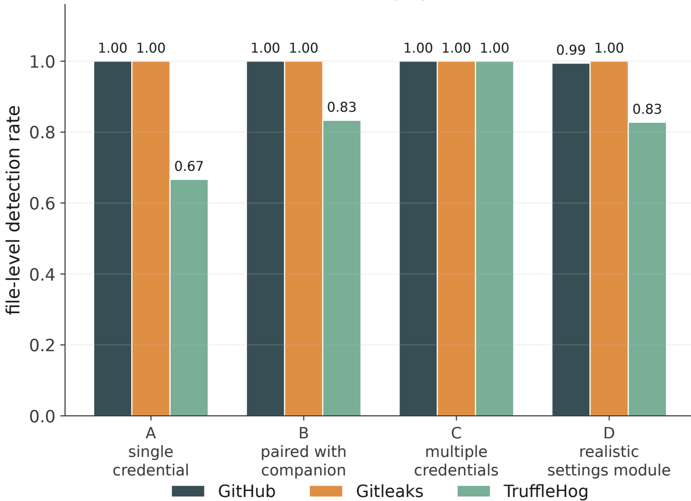
(a) Detection across deployment conditions
