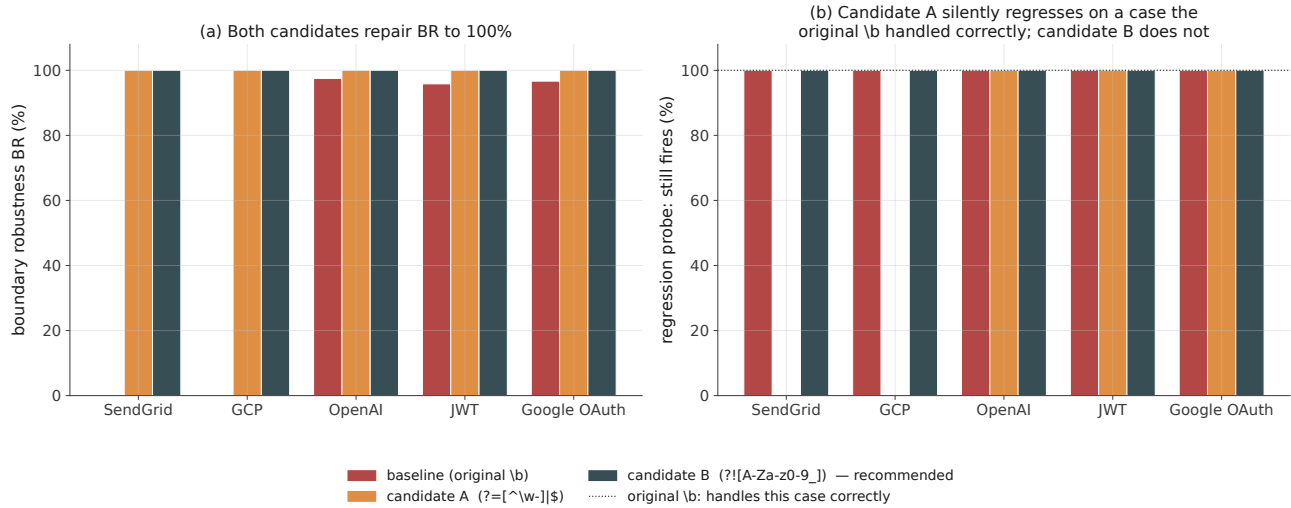
Fig. 6. Fix validation. (a) Both candidates repair boundary robustness to 1.0 on all five affected rules. (b) A regression probe — a credential ending in a word character, followed by a hyphen — that the original rule handled correctly. Candidate A silently fails it on the two fixed-count-quantifier rules; Candidate B does not.
