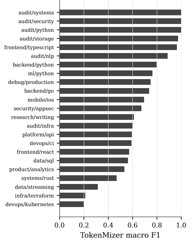
Fig. 7. TokenMizer macro F1 by domain, n=100, 23 domains. The three domains at 100% are audit/* real sessions; infrastructure-heavy synthetic domains (devops/kubernetes, infra/terraform, data/streaming) score lowest.
