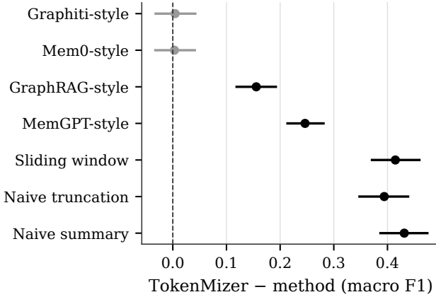
Fig. 4. Paired bootstrap difference (TokenMizer 0.5.4 - method) on macro F1, n=100 , 95% CI. Intervals excluding zero (black) are reliable differences; the two grey intervals (Graphiti-style, Mem0-style) cross zero.
