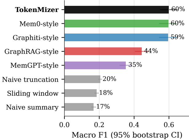
Fig. 3. Macro F1 by method, ranked, n=100 , with 95% bootstrap confidence intervals. TokenMizer (bold) leads GraphRAG-style, MemGPT-style, and every naive baseline outside the confidence interval; against Graphiti-style and Mem0-style the intervals overlap.
