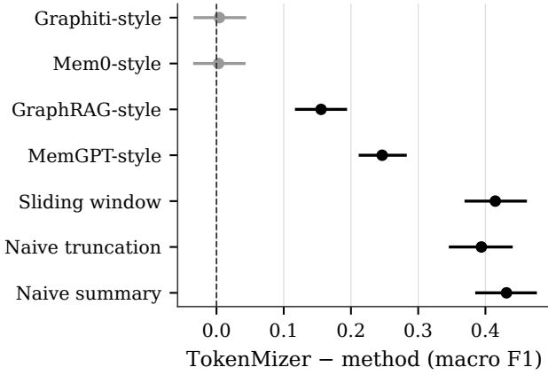
Fig. 7. Paired bootstrap difference (TokenMizer 0.5.3 — method) on macro F1, n=100, 95% CI. Intervals excluding zero (black) are reliable differences; the two grey intervals (Graphiti-style, Mem0-style) cross zero. All five black intervals sit further from zero than in the 0.5.2 measurement (Table X), and the two grey ones have moved from entirely negative to centred on zero.
