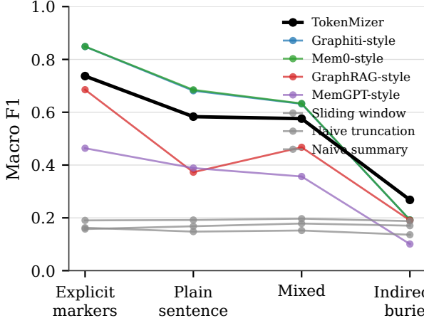
Fig. 9. Macro F1 by register, n=100, TokenMizer 0.5.3. All four pattern-matching methods converge to 19–27% once explicit markers (“Decided:”, “Completed:”) are absent from the text, a shared ceiling of the extraction strategy rather than of any one implementation.
