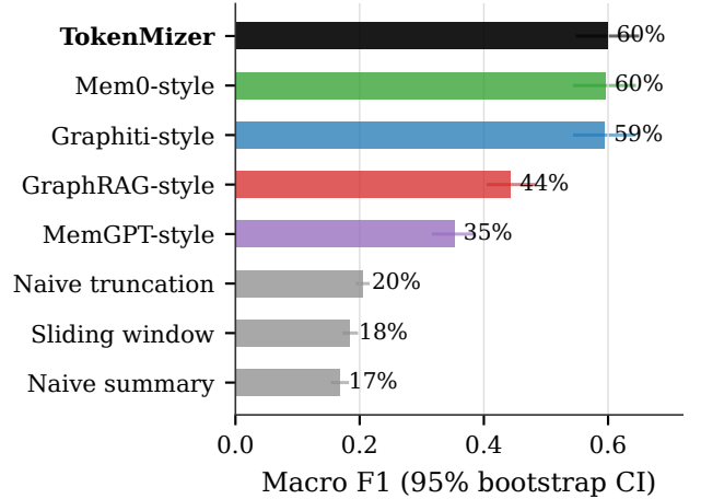
Fig. 6. Macro F1 by method, ranked, n=100 , with 95% bootstrap confidence intervals. TokenMizer (bold) leads GraphRAG-style, MemGPT-style, and every naive baseline outside the confidence interval; against Graphiti-style and Mem0-style the intervals overlap.
