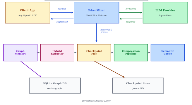
Fig. 1: TokenMizer System Architecture — Transparent OpenAI-Compatible Proxy
