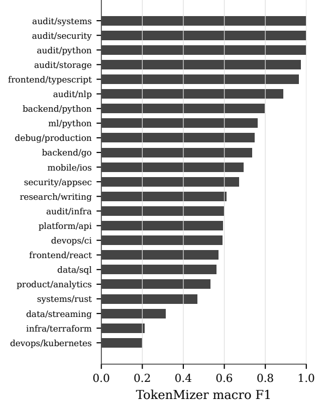
Fig. 10. TokenMizer macro F1 by domain, n=100, 23 domains. The three domains at 100% are audit/* real sessions; infrastructure-heavy synthetic domains (devops/kubernetes, infra/terraform, data/streaming) score lowest.
