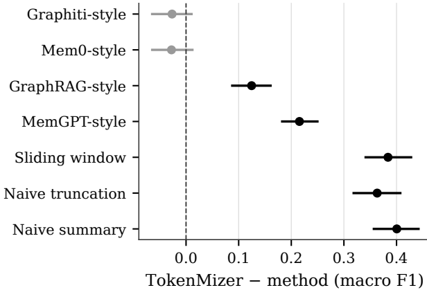
Fig. 4. Paired bootstrap difference (TokenMizer 0.5.3 - method) on macro F1, n=100 , 95% CI. Intervals excluding zero (black) are reliable differences; the two grey intervals (Graphiti-style, Mem0-style) cross zero.
