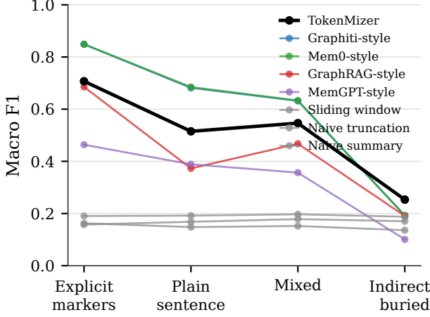
Fig. 6. Macro F1 by register, n=100. All four pattern-matching methods converge to 19–25% once explicit markers (“Decided:”, “Completed:”) are absent from the text, a shared ceiling of the extraction strategy rather than of any one implementation.
