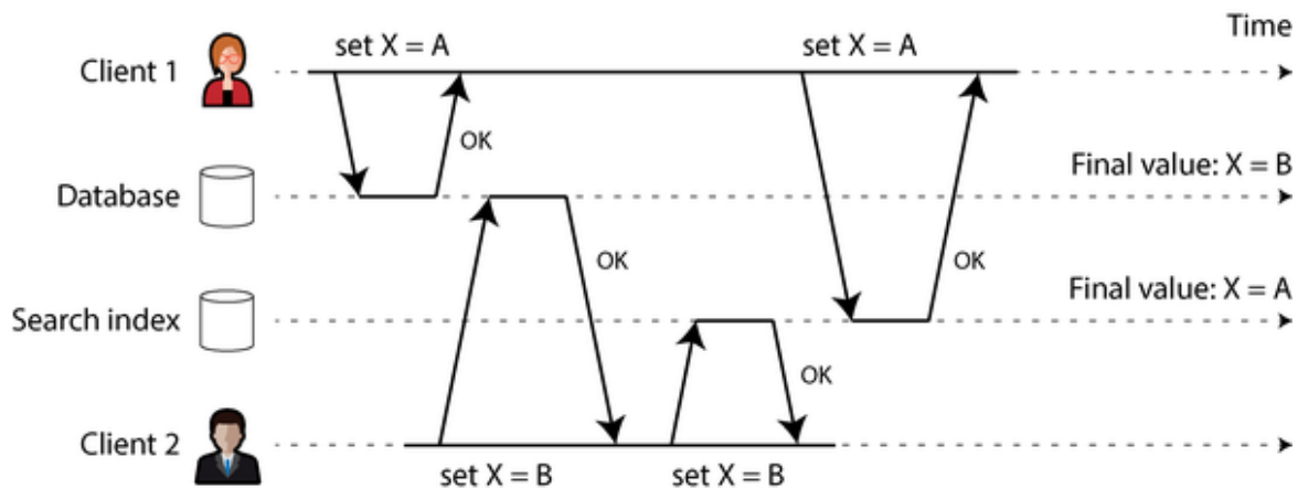
Figure 12-4. In the database, X is first set to A and then to B , while at the search index the writes arrive in the opposite order.
