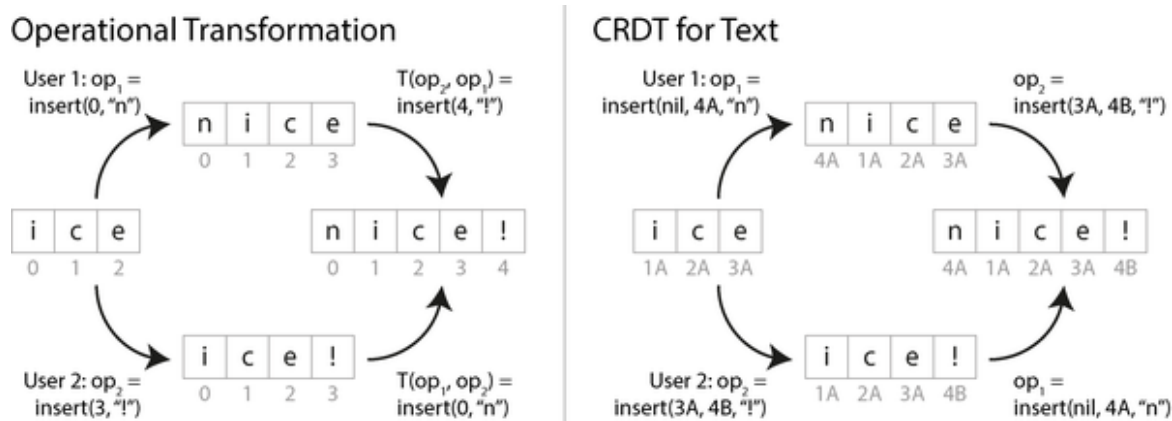
Figure 6-11. How two concurrent insertions into a string are merged by OT and a CRDT, respectively
