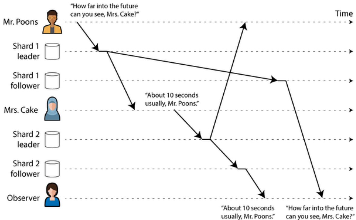
Figure 6-5. If some shards are replicated slower than others, an observer may see the answer before they see the question.
