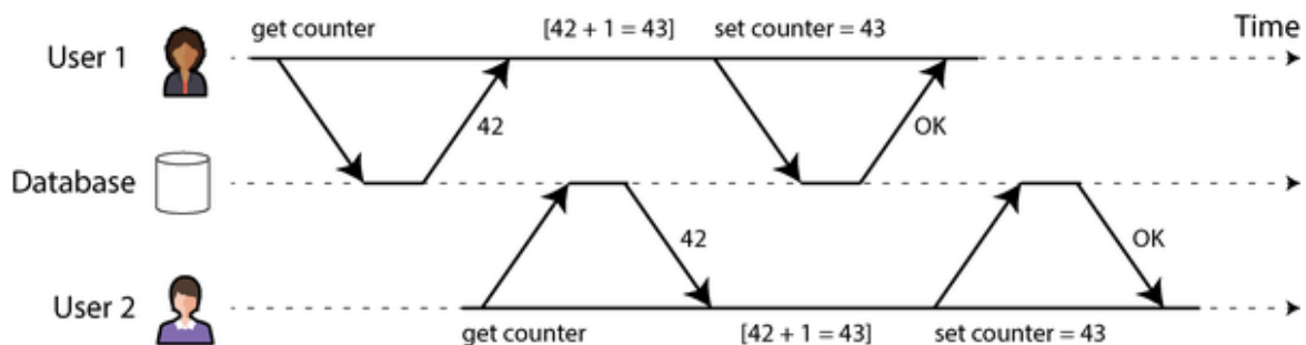
Figure 8-1. A race condition between two clients concurrently incrementing a counter
