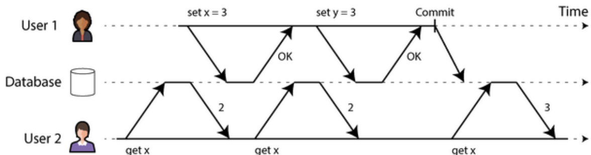
Figure 8-4. No dirty reads: user 2 sees the new value for x only after user 1's transaction has committed
