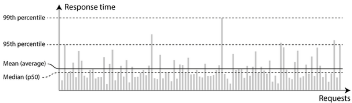
Figure 2-5. Illustrating mean and percentiles: response times for a sample of 100 requests to a service
