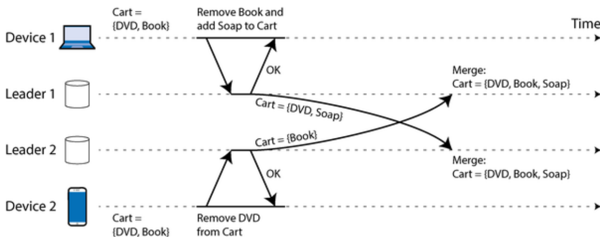
Figure 6-10. An example of Amazon's shopping cart anomaly: if conflicts are merged by taking the union of the set, deleted items may reappear
