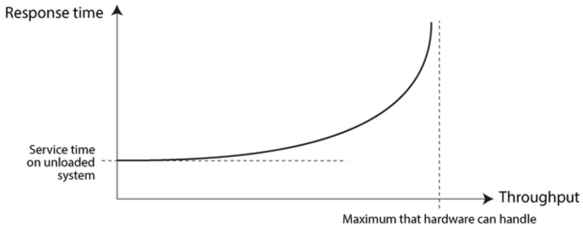
Figure 2-3. As the throughput of a service approaches its capacity, the response time increases dramatically because of queueing.
