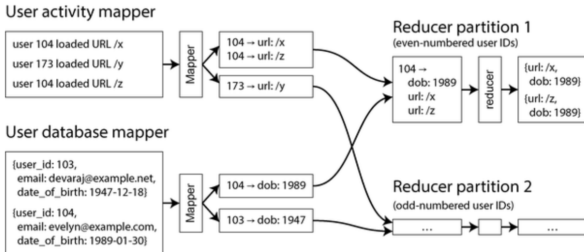
Figure 11-3. A sort-merge join on user ID; if the input datasets are sharded into multiple files, each could be processed with multiple mappers in parallel
