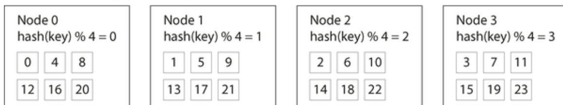
Figure 7-3. Assigning keys to nodes by hashing the key and taking it modulo the number of nodes. Changing the number of nodes results in many keys moving from one node to another.
