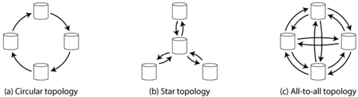
Figure 6-7. Three example topologies for multi-leader replication
