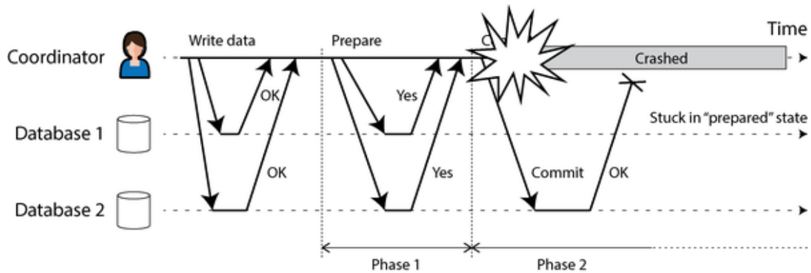
Figure 8-14. The coordinator crashes after participants vote yes. Database 1 does not know whether to commit or abort.
