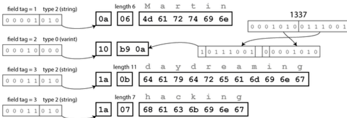
Figure 5-3. Our record encoded using Protocol Buffers
