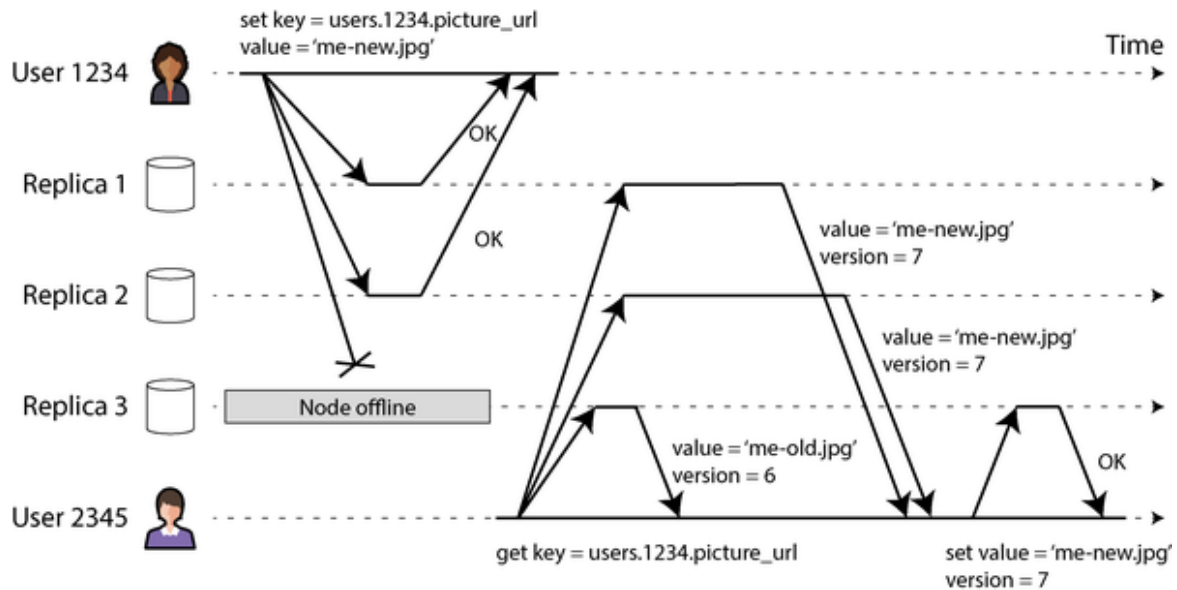
Figure 6-12. Writing to a majority of replicas, reading from a majority, and forwarding the latest value to a replica that was unavailable during the write
