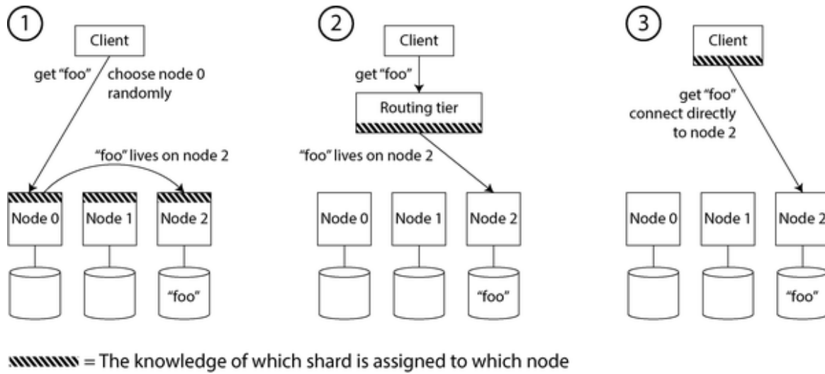
Figure 7-7. Three ways of routing a request to the right node
