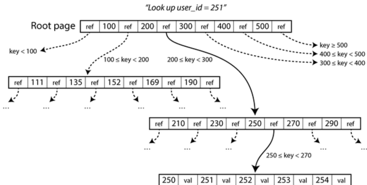
Figure 4-5. Looking up key 251 by using a B-tree index. From the root page, we first follow the reference to the page for keys 200–300, then the page for keys 250–270.
