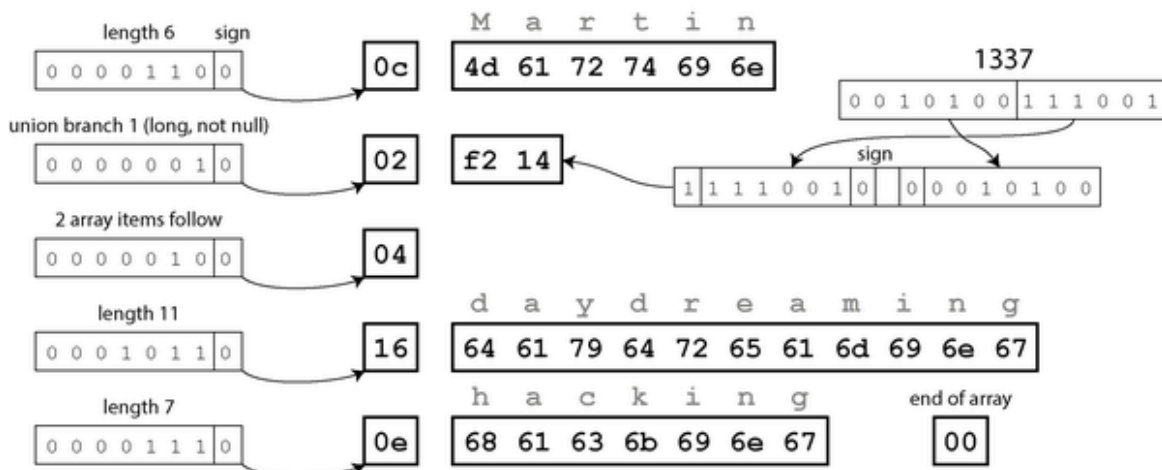
Figure 5-4. Our record encoded using Avro
