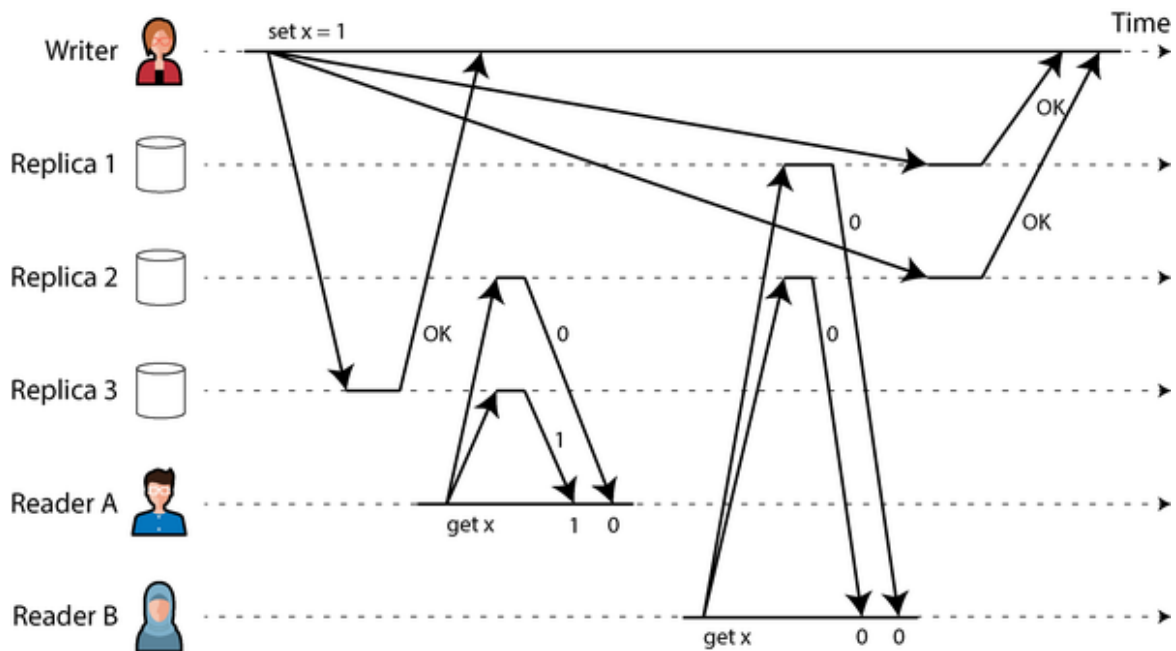
Figure 10-6. A nonlinearizable execution, despite using a quorum
