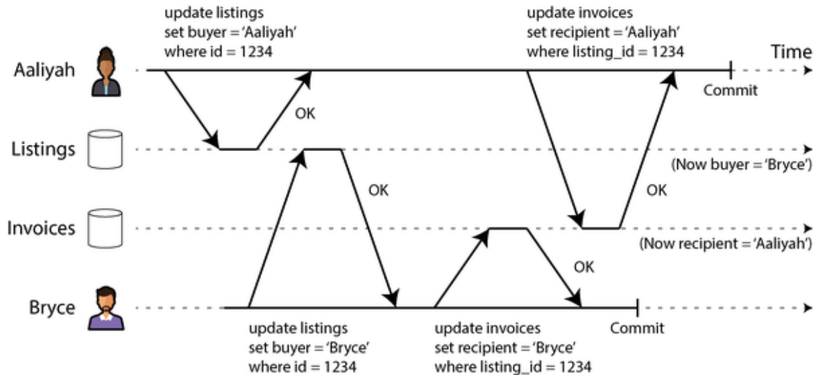
Figure 8-5. With dirty writes, conflicting writes from different transactions can be mixed up
