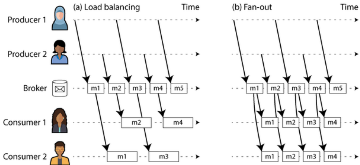
Figure 12-1. (a) Load balancing shares the work of consuming a topic among consumers; (b) with fan-out, each message is delivered to multiple consumers.
