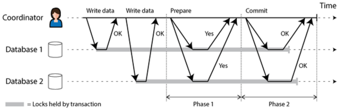
Figure 8-13. A successful execution of 2PC
