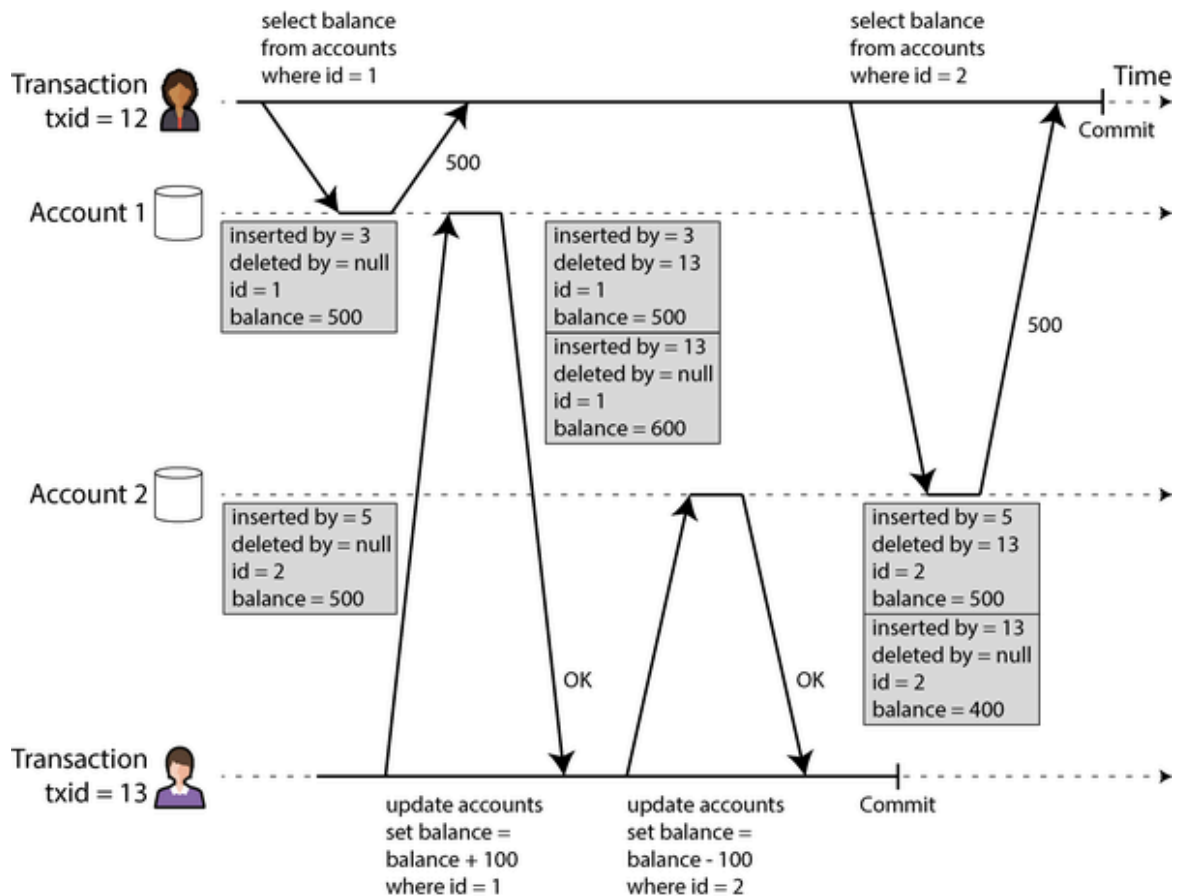
Figure 8-7. Implementing snapshot isolation using multiversion concurrency control
