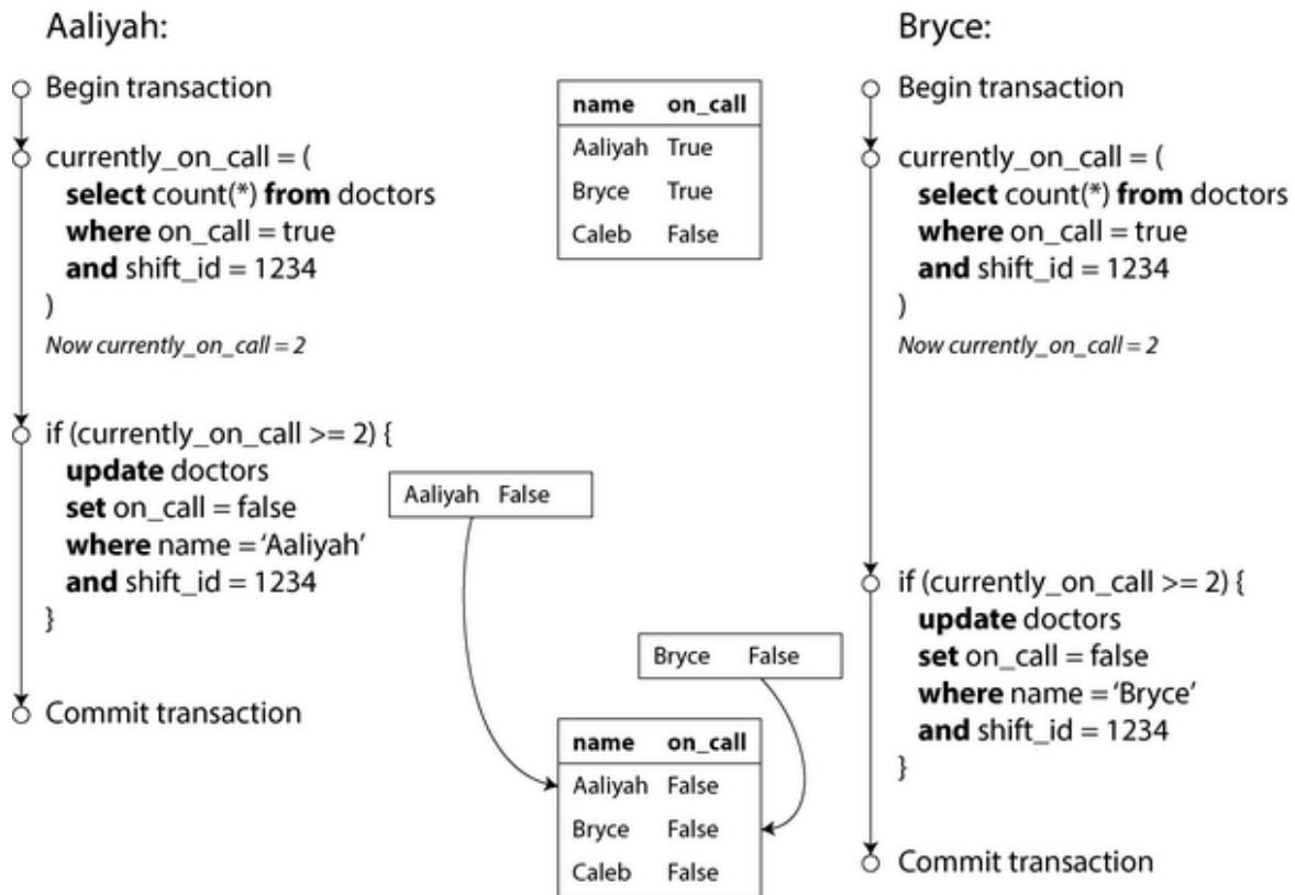
Figure 8-8. A write skew causing an application bug
