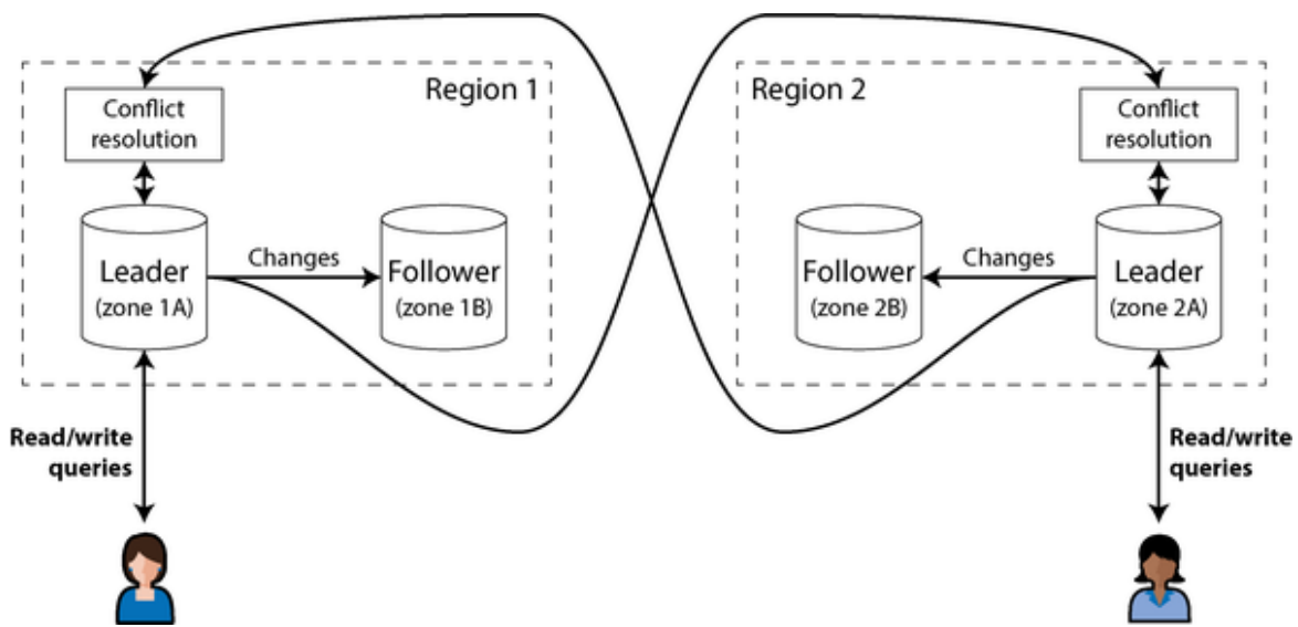
Figure 6-6. Multi-leader replication across multiple regions
