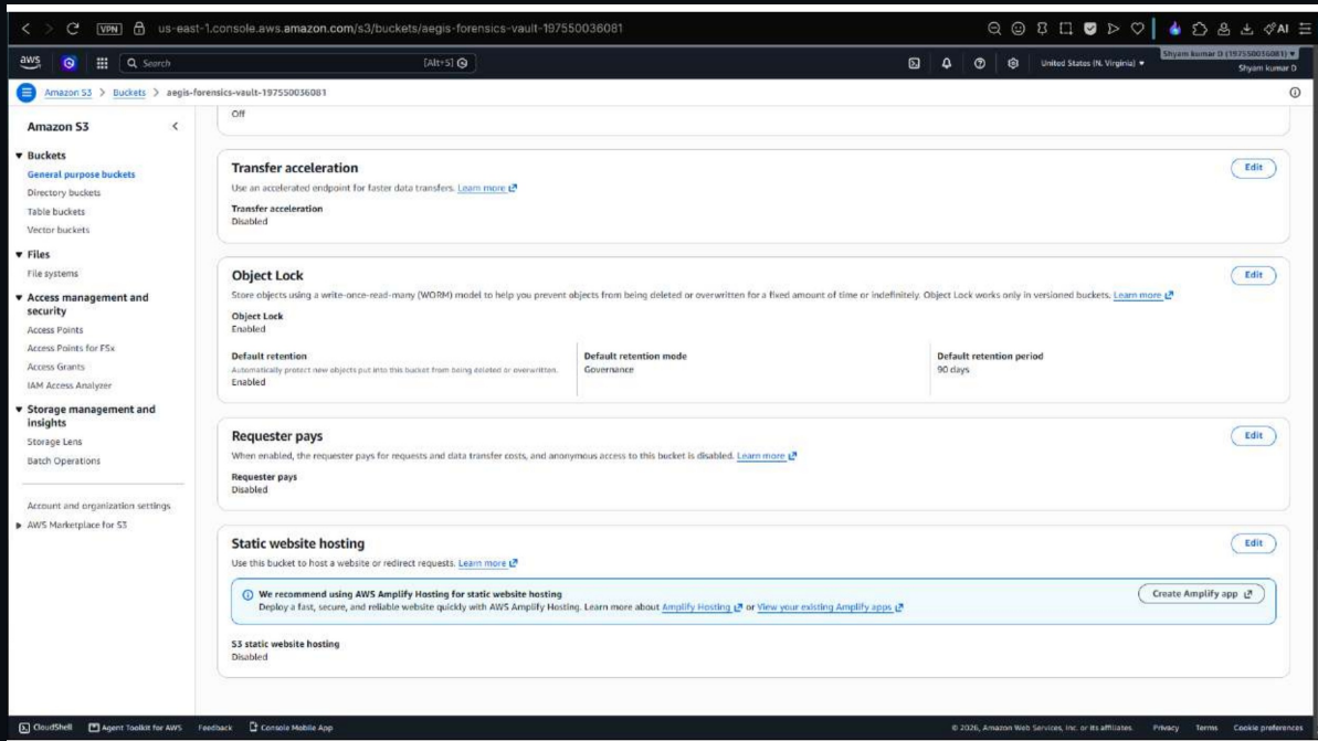
S3 bucket properties – Object Lock enabled with 90-day Governance-mode retention
