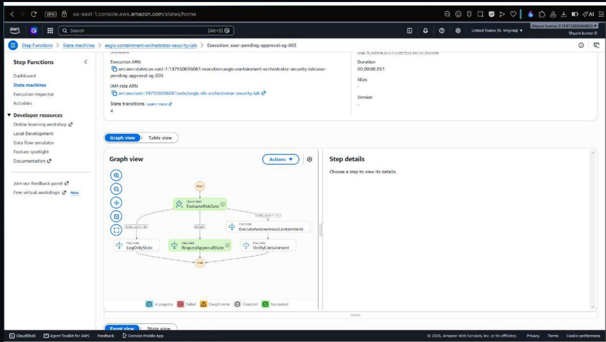
SOAR containment orchestrator – automated risk-based remediation branches
