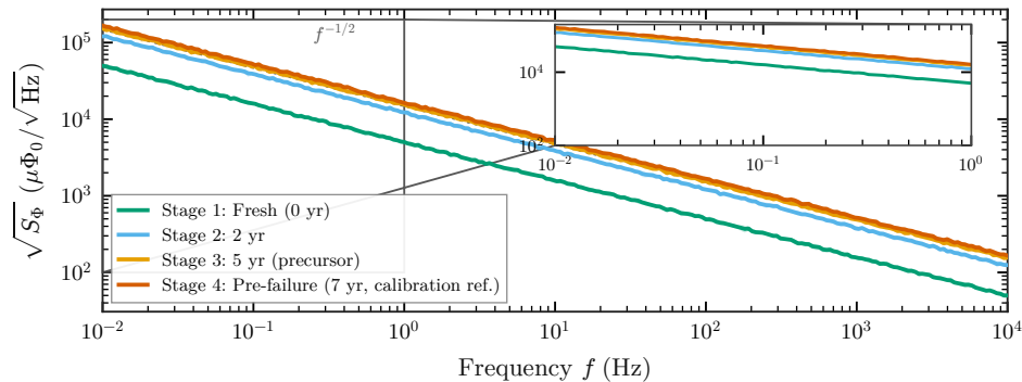
Figure 1. SQUID flux-noise spectrum evolution across sensor operating life
