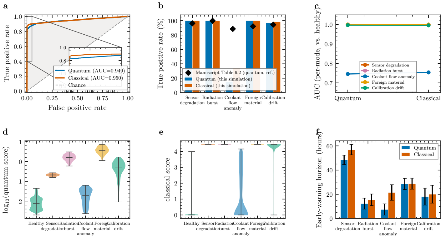
Figure 2. Quantum vs. classical anomaly-detection performance across five failure modes
